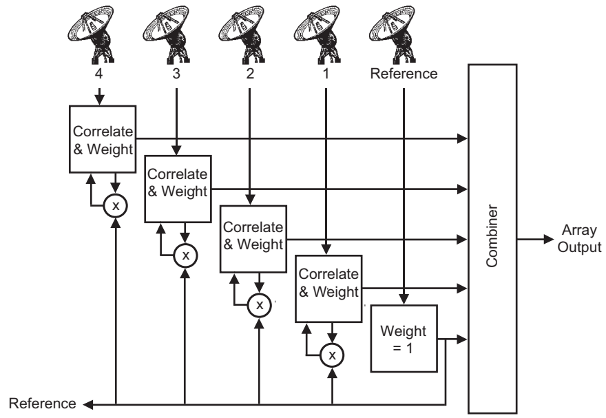
Fig. 8-1. Diagram for the Simple method of combining.
