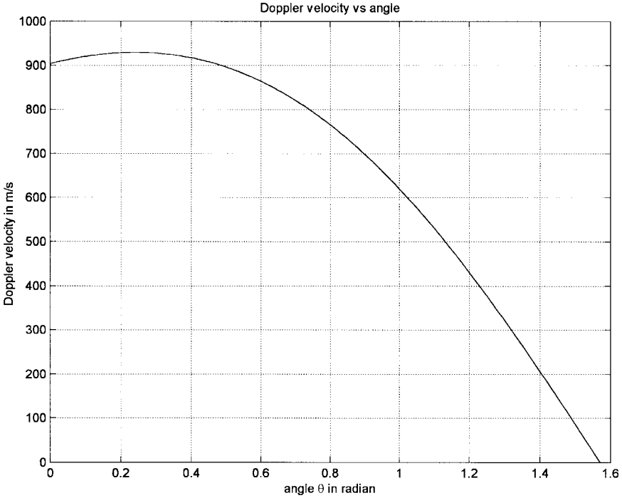
FIGURE 3.4 Velocity component toward the user versus angle \theta .
