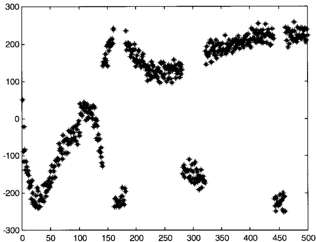
FIGURE 8.4 Outputs from conventional tracking method of sv17.
