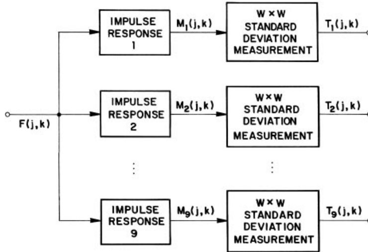
FIGURE 16.6-8. Laws microstructure texture feature extraction method.
