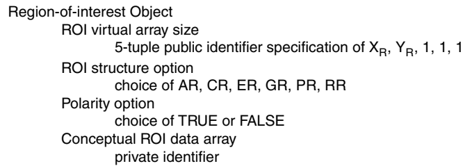
FIGURE 20.2-6. Region-of-interest object tree structure.
