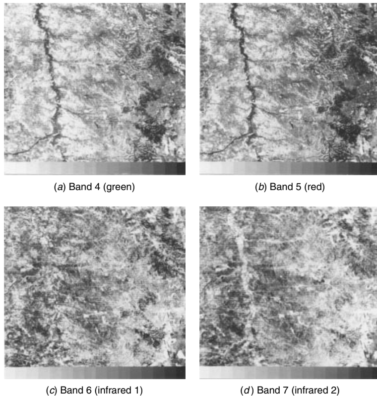
FIGURE 10.6-1. Multispectral images.
