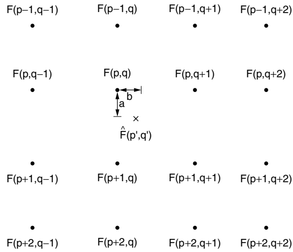
FIGURE 13.5-2. Bicubic interpolation.
