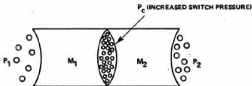
Fig. 10. Two Bodies at Moment of Collision
