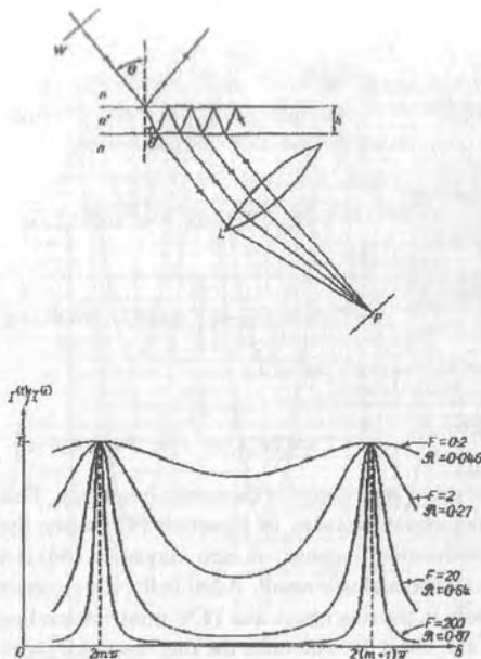
Figure 10. (a) Formation of multiple beam fringes in a parallel plate of index of refraction n' , focused to give the transmitted intensity (power density) I . (b) The Airy function - a plot of the ratio of the transmitted and incident intensities as a function of the propagation path-produced phase difference \delta = 4\pi n' \cos \theta / \lambda_0 . [Ref. Born and Wolf, pp. 326-7. Script R is the power reflection coefficient r' and F = 4R/(1-R)^2 .]
