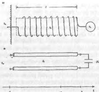
Figure 7. A slow-wave helical transmission line resonator (a Tesla coil).
