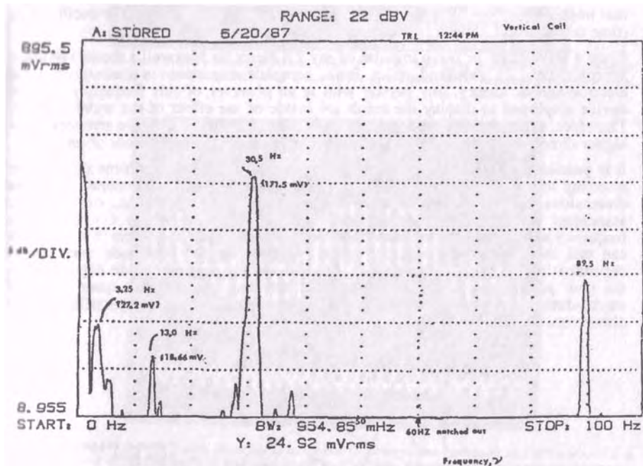
figure 4. In the 0 to 100 Hz range with 60 Hz notch filters to notch out the 60 Hz, we see the spurious side bands of 30.5 Hz and 89.5 Hz from the center band of 70 to 76 Hz for Project ELF. The 30 Hz signal is nearly always larger than the 89.5 signal since it lies near one of the Earth's rotational resonant frequencies. In earlier measurements there were also some effects of coil roll-off.
