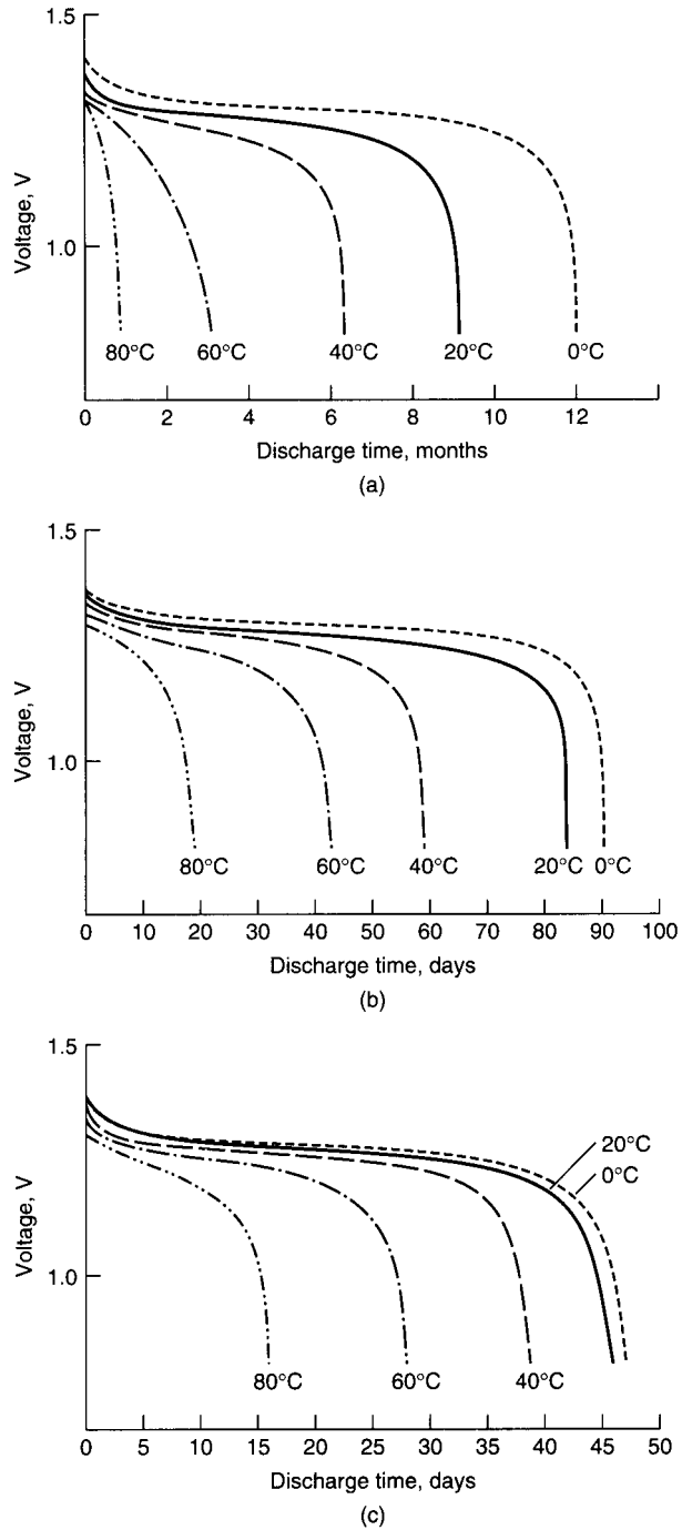
FIGURE 28.37 Performance of memory-backup batteries. Charge— C/30 for 48 h at 20^{\circ}\text{C} . Discharge rate: (a) C/10,000 ; (b) C/2000 ; (c) C/1000 .
