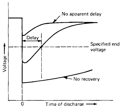
FIGURE 3.25 Voltage delay
