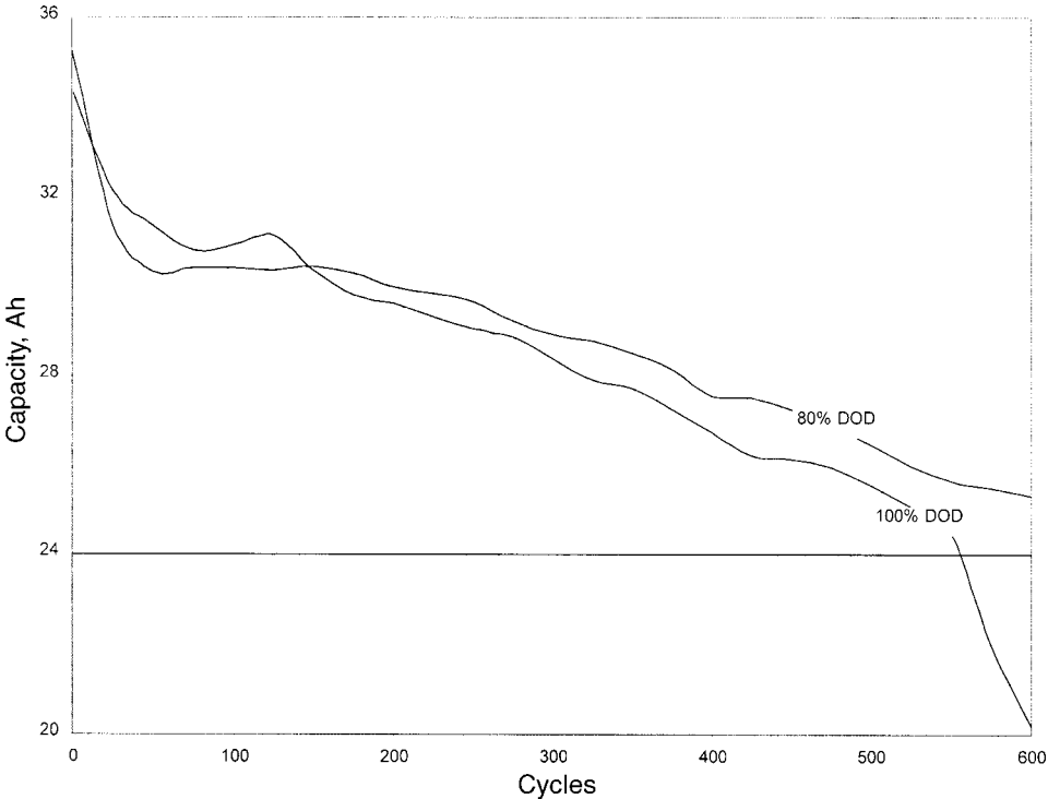
FIGURE 31.14 Cycle life of 12 V, 30 Ah nickel-zinc battery. 80% DOD testing performed by JBI. (Courtesy of JBI and Evercel Corp.)
