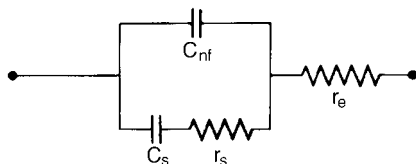
FIGURE 2.29 Equivalent circuit for a cell where the cell impedance is kinetically controlled and is localized at the working electrode by using a large, unpolarized counterelectrode. C_{nf} —nonfaradic capacitance; C_s , r_s —faradic components of impedance; r_e —electrolyte resistance.
