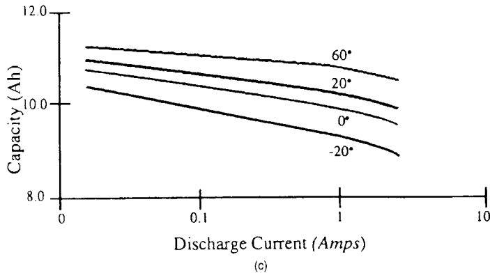
FIGURE 14.55 Discharge characteristics of spiral-wound Li/MnO 2 D-size battery. (a) Discharge curve at 2 amp rate at 3 temperatures; (b) start-up characteristic after 2-weeks storage at 70°C. (c) Capacity as a function of discharge rate at 4 temperatures. (d) Operating voltage vs discharge rate at 4 temperatures. (Source: Manufacturer's Data Sheet.)
