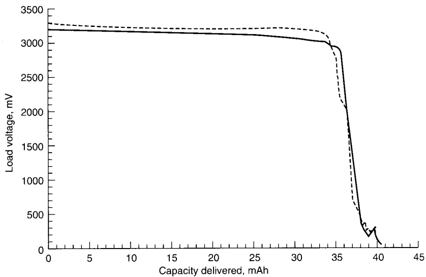
FIGURE 15.24 64.9-k \Omega constant-load discharge of Ag/RbAg 4 I 5 /Me 4 NI 6 batteries after 20 years of storage at 25°C. Discharge temperature: solid curve—25°C; dashed curve—60°C. (From Ref. 29.)
