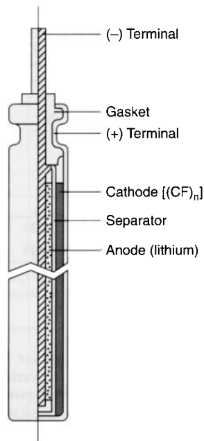
FIGURE 14.62 Cross-sectional view of \text{Li}/(\text{CF})_n pin-type battery. (Courtesy of Panasonic, Division of Matsushita Electric Corp. of America.)
