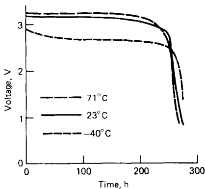
FIGURE 15.21 Discharge of Ag/Me 4 N 5 battery, 21.5-kΩ constant load. (From Topics in Applied Physics , vol. 21, reprinted by permission of the publisher, Springer-Verlag.)
