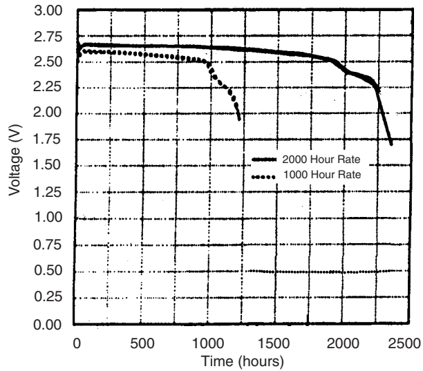
FIGURE 14.75 Typical discharge curves for 1200 Ah Li/(CF) n battery.
