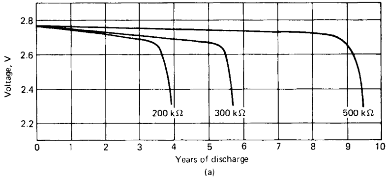
FIGURE 15.15 Projected discharge curves for S19P-20 button watch battery at 25°C. (Courtesy of Catalyst Research Corp.)
