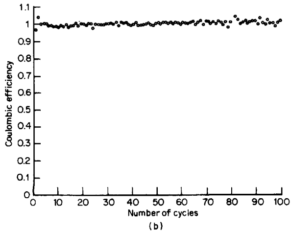
FIGURE 34.33 (a) Discharge/charge behavior of a Li/CuCl 2 prismatic D-size battery in LiAlCl 4 · 6SO 2 electrolyte at 1 mA/cm 2 . (b) Coulombic efficiency of a Li/CuCl 2 battery at 1 mA/cm 2 . (From Yardney Technical Products, Inc.)
