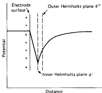
FIGURE 2.14 Potential distribution of positively charged electrode.
