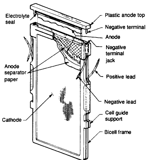
FIGURE 38.24 Zinc/air bicell.
