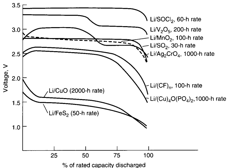
FIGURE 14.4 Typical discharge curves of lithium/solid-cathode batteries.
