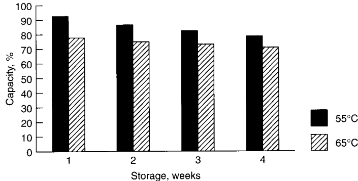
FIGURE 36.14 Capacity retention of mercury-free rechargeable zinc/alkaline/manganese dioxide AA-size batteries at 20°C. (Courtesy of Battery Technologies, Inc.)
