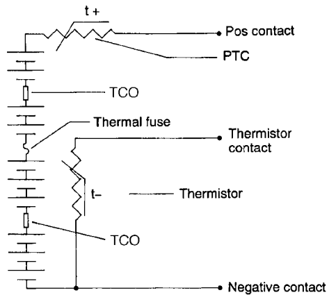
FIGURE 5.16 Protective devices for charge control.
