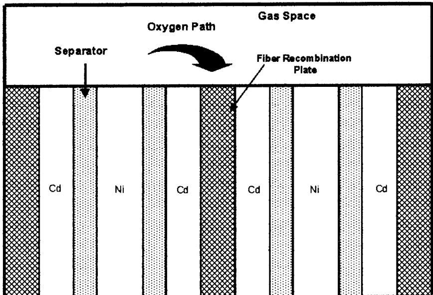
FIGURE 26.13 Electrode structure of fiber nickel-cadmium cell.
