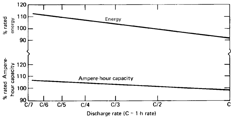
FIGURE 25.14 Capacity as a function of discharge rate. (Courtesy of Westinghouse Electric Corp.)
