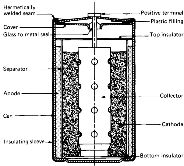
FIGURE 14.16 Cross section of bobbin-type Li/SOCl 2 battery. (From Ref. 23.)
