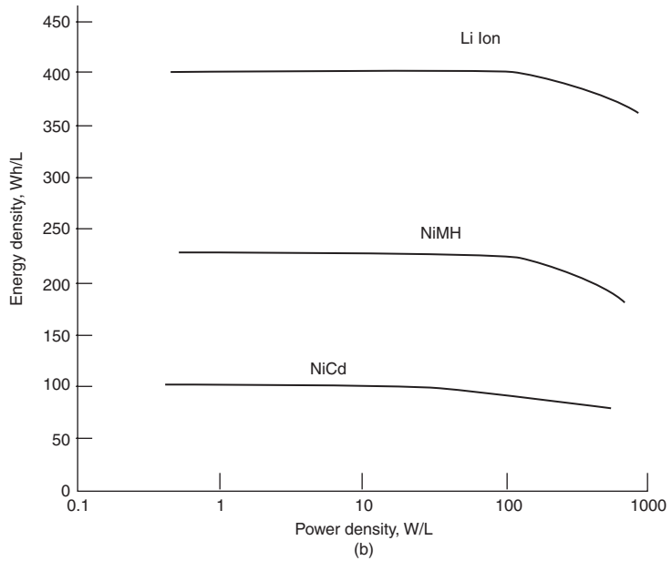
FIGURE 22.4 Comparison of rechargeable 14500 Li ion and AA-size NiMH and NiCd batteries at 20°C. (a) Specific energy vs. power density. (b) Energy density vs. power density.
