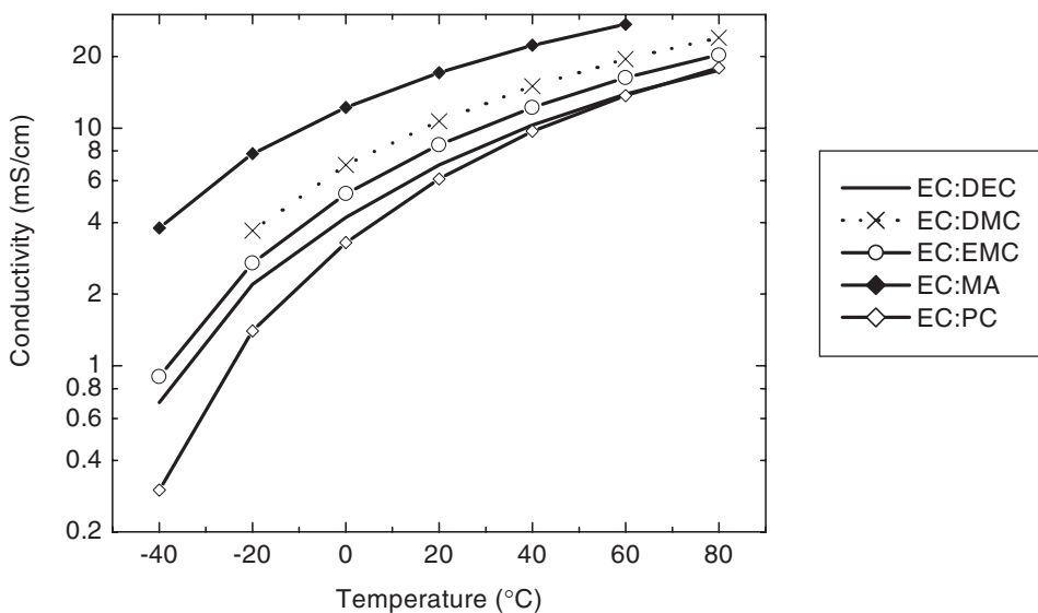
FIGURE 35.24 Conductivity of 1M LiPF 6 solutions in various binary mixtures, 1:1 by weight. (Courtesy of Merck KGaA, Darmstadt, Germany.)
