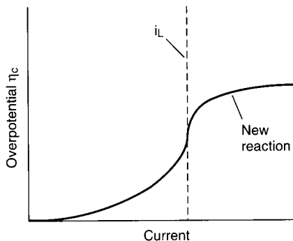
FIGURE 2.16 Plot of overpotential \eta_c vs. current i .
