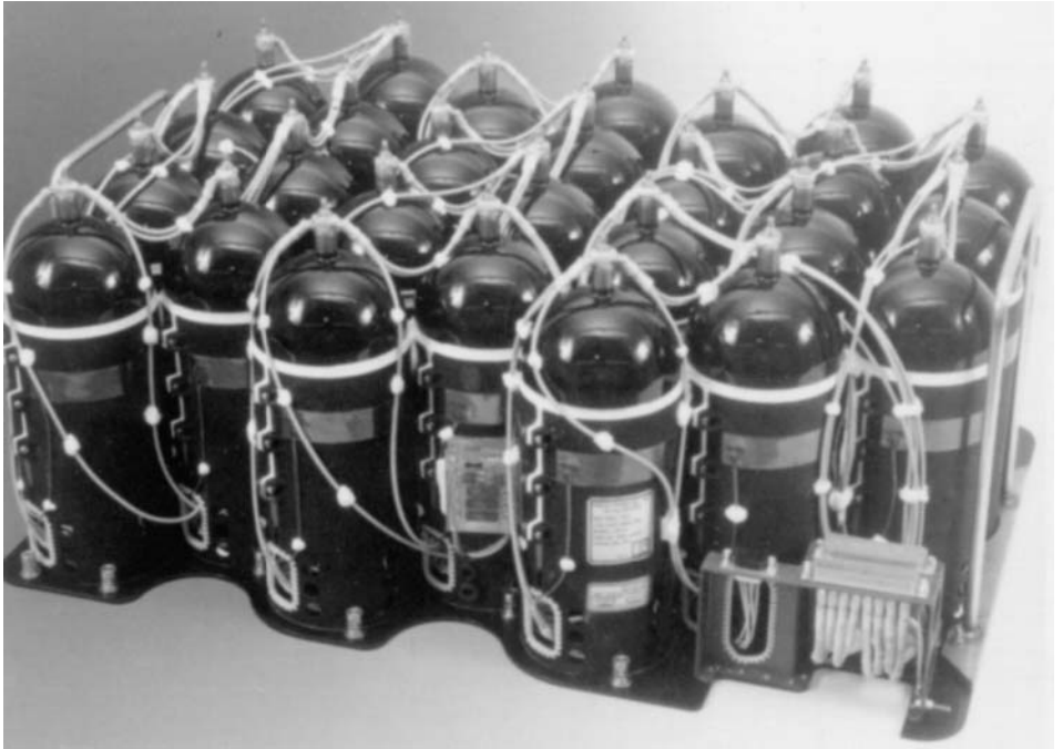
FIGURE 32.7 EUTELSAT II 58-Ah Ni-H 2 battery.
