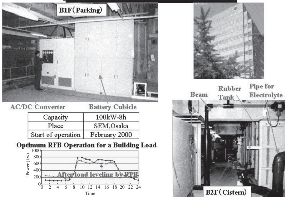
FIGURE 37.5 Application of Vanadium redox battery in an office building.
