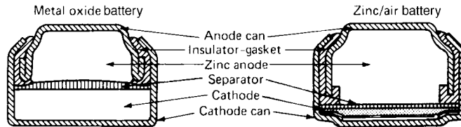
FIGURE 13.2 Cross section of metal oxide and zinc/air button batteries (Courtesy of Duracell, Inc.)
