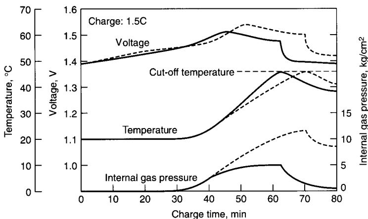
FIGURE 28.33 Comparison of charge characteristics of fast-charge (solid line) battery vs. standard battery (broken line).
