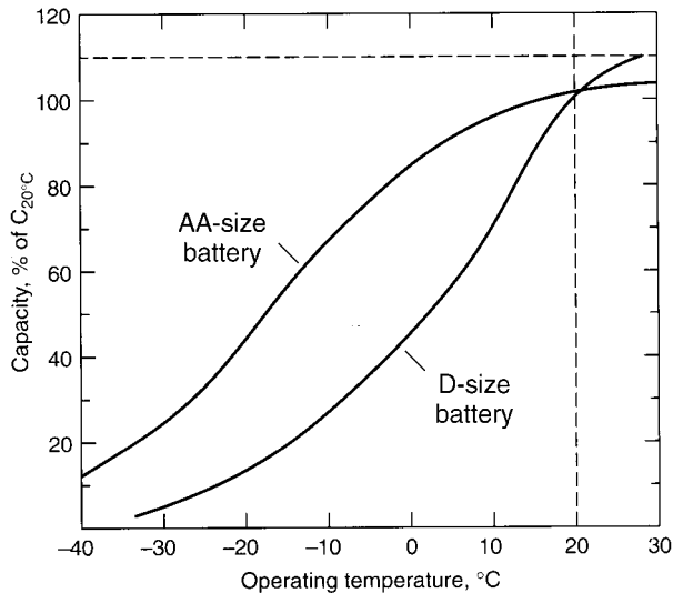
FIGURE 36.12 Comparison of performance of rechargeable zinc/alkaline/manganese dioxide D and AA-size batteries at various temperatures. Discharge at C/20 rate, to 0.9-V end voltage. (Courtesy of Battery Technologies, Inc.)
