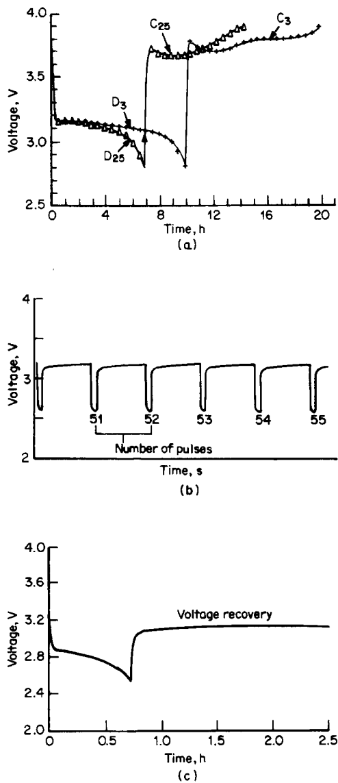
FIGURE 34.32 (a) Discharge/charge behavior of a \text{Li/LiAlCl}_4 \cdot 6\text{SO}_2 C-size battery at 1 \text{ mA/cm}^2 . Voltage limits; 2.8–4.0 V. Line—battery, symbols ( \Delta )—cathode vs. ref. (b) High-rate pulse discharge of a \text{Li/LiAlCl}_4 \cdot 6\text{SO}_2 C-size battery. Pulse rate at 20 \text{ mA/cm}^2 for 20 s. Rest period for 180 s. (c) Discharge characteristics and voltage recovery (without load) of a \text{Li/LiAlCl}_4 \cdot 6\text{SO}_2 C-size battery at -20^\circ\text{C} . Discharge at 3.2 \text{ mA/cm}^2 . (From Yardney Technical Products, Inc.)
