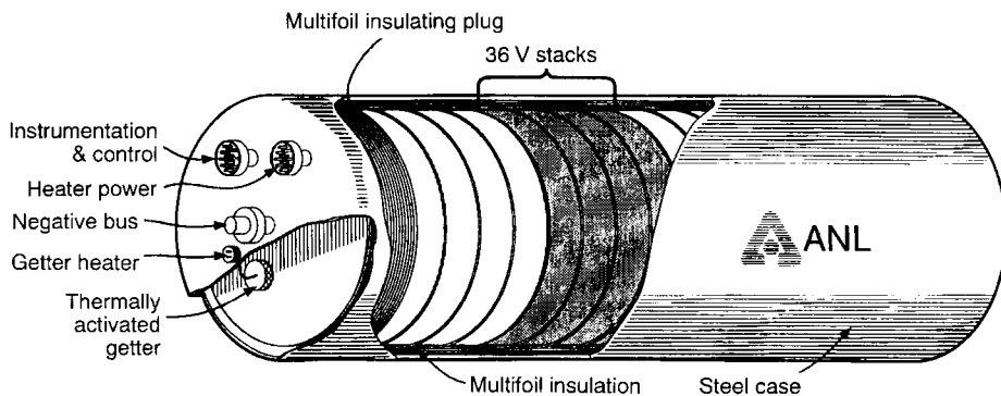
FIGURE 41.17 Artist's concept of thermally insulated electric-vehicle battery module with cutaway showing bipolar Li-Al/FeS, stack, lightweight loosely wrapped multifoil insulation, and thermally activated getter system for controlling heat transfer from module. (Courtesy of Argonne National Laboratory.)
