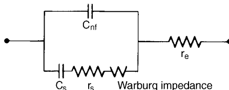
FIGURE 2.32 Equivalent circuit for an electrode process limited by both charge-transfer kinetics and diffusion processes. The diffusion portion of the impedance is represented by the Warburg impedance, the other circuit components are the same as in Fig. 2.29.
