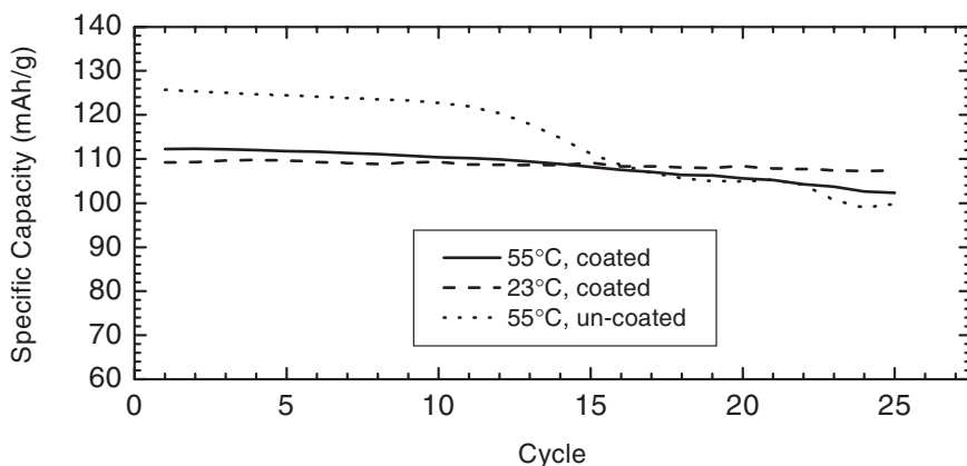
FIGURE 35.15 Specific capacity of \text{LiCo}_2 coated and un-coated spinels cycled at the C/2 rate between 4.2 and 3.5 V at 23°C or 55°C. (Courtesy of Carus Chemical.)
