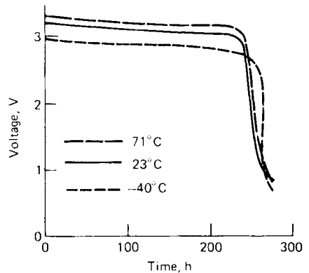
FIGURE 15.22 Discharge of Ag/Me 4 N 9 battery. (From Topics in Applied Physics , vol. 21, reprinted by permission of the publisher, Springer-Verlag.)
