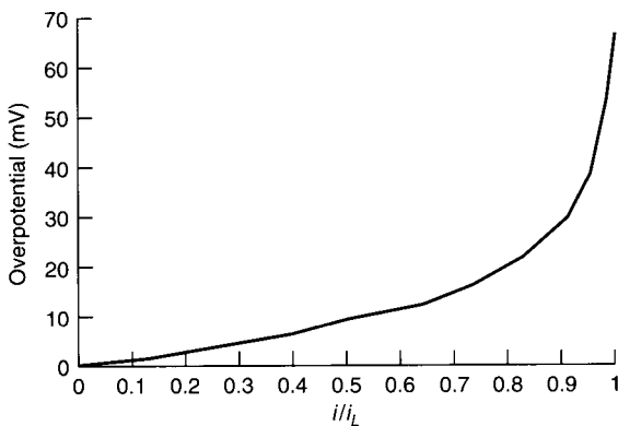
FIGURE 2.17 Magnitude of concentration overpotential as a function of i/i_L , with n = 2 at 25^\circ\text{C} , based on Eq. (2.40).
