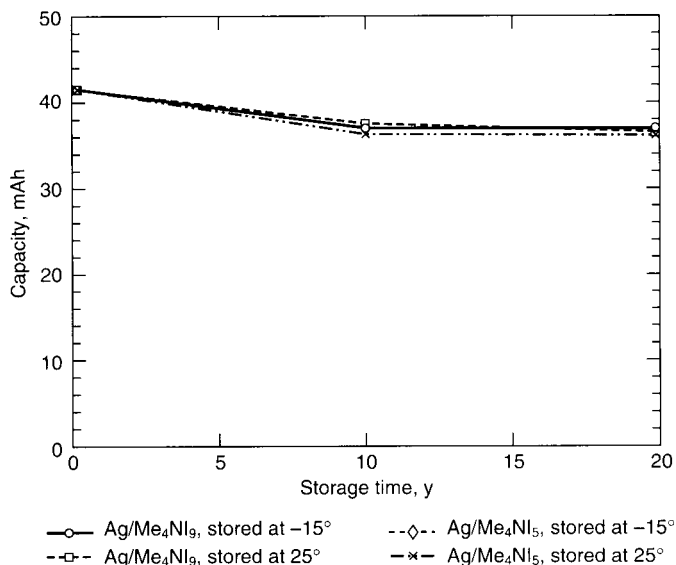
FIGURE 15.25 Capacity of Ag/RbAg 4 I 5 /Me 4 Ni 9 batteries as a function of storage time. (From Ref. 29.)
