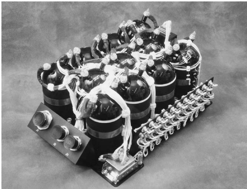
FIGURE 32.10 MIDEX 23-Ah CPV Ni-H 2 battery assembly.
