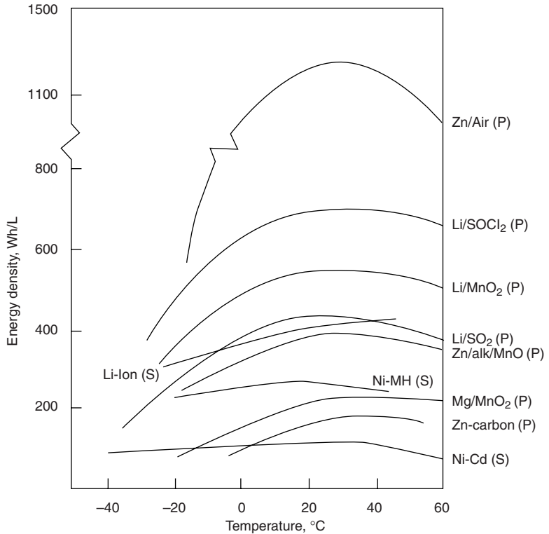
FIGURE 6.6 Effect of temperature of primary (P) and secondary (S) batteries.
