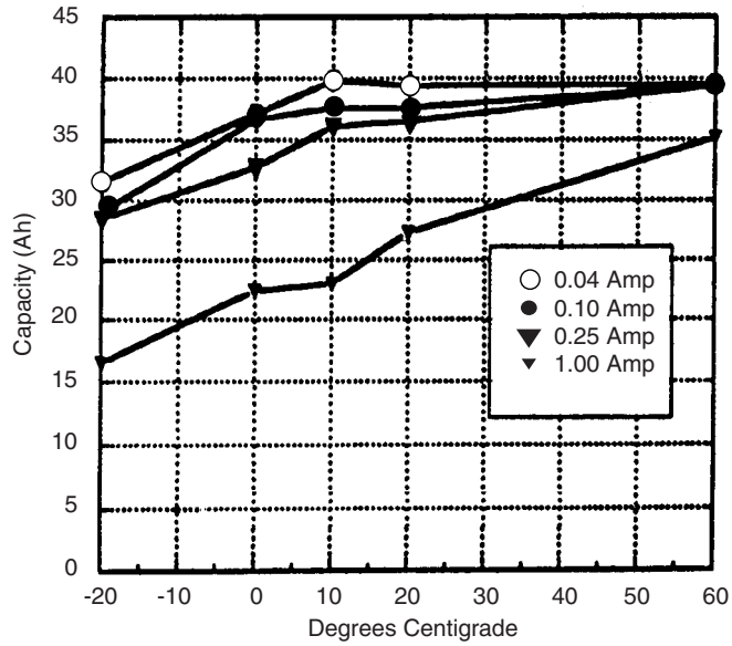
FIGURE 14.74 'DD' Li/(CF) n discharge performance as a function of rate and temperature.
