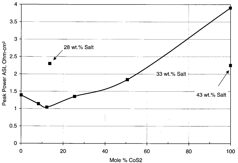
FIGURE 41.12 Peak power ASI evaluated at 80% DOD as a function of mole % \text{CoS}_2 additive. (From Henriksen, et al. 8 )
