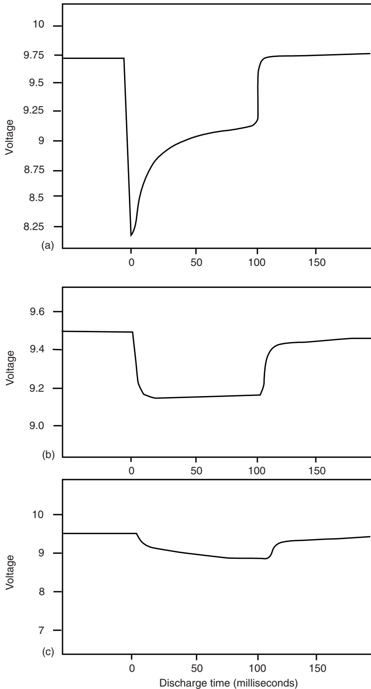
FIGURE 3.15 Discharge characteristics of a 9-volt battery subjected to a 100 ms pulse (smoke detector pulse tests): (a) zinc-carbon battery; (b) and (c) zinc/alkaline/manganese dioxide battery.
