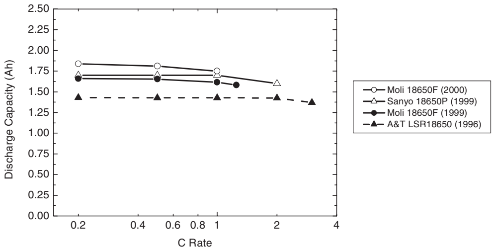
FIGURE 35.40 Comparison of the rate capability at constant current for C/LiCo 2 18650 batteries.
