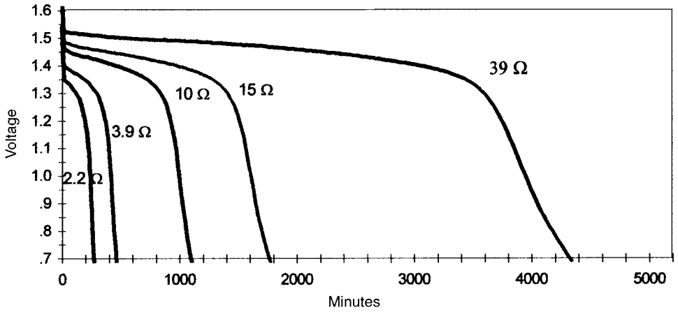
FIGURE 14.81 Constant resistance continuous discharge of Li/FeS 2 “AA”-size batteries at 21°C (Courtesy of Eveready Battery Co, Inc.)
