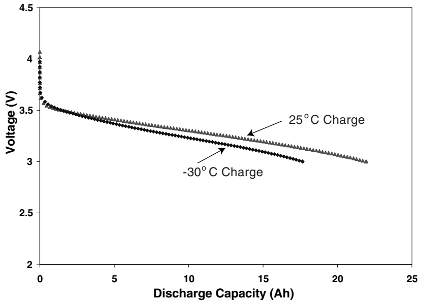
FIGURE 35.79 Discharge of a Yardney 35 Ah prismatic Li-ion cell at -30^{\circ}\text{C} at 2.5 A after charge at 2.5 A at 25^{\circ}\text{C} or -30^{\circ}\text{C} . (Courtesy of JPL.)
