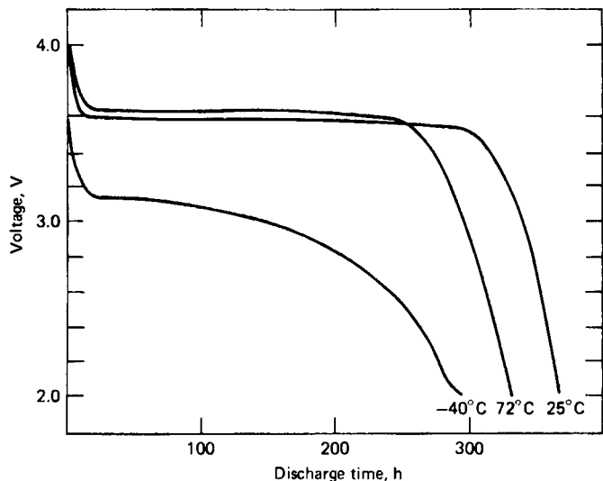
FIGURE 20.16 Typical discharge curves on 1.25 kOhm of Li/SOCl 2 reserve battery, Tadiran model TL-5160. (Courtesy of Tadiran Industries, Ltd).
