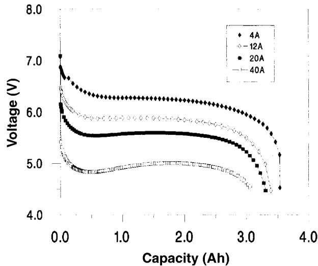
FIGURE 30.12 Voltage-Capacity profiles for high power NiMH cylindrical 3.5 Ah C-size batteries at different rates on continuous discharge.
