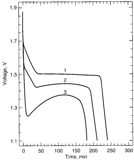
FIGURE 33.5 Typical discharge curves of HR-5 silver zinc battery at C/3 (2-A) rate. Curve 1— 25^{\circ}\text{C} ; curve 2— 0^{\circ}\text{C} ; curve 3— -18^{\circ}\text{C} .
