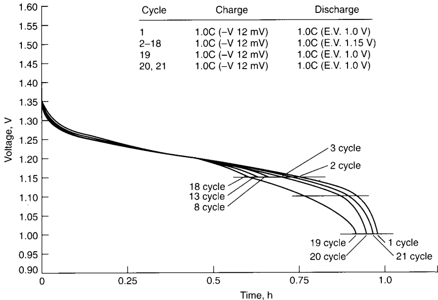
FIGURE 29.13 Voltage depression during cycling of sealed cylindrical nickel-metal hydride battery, 20°C. (Courtesy of Duracell, Inc.)
