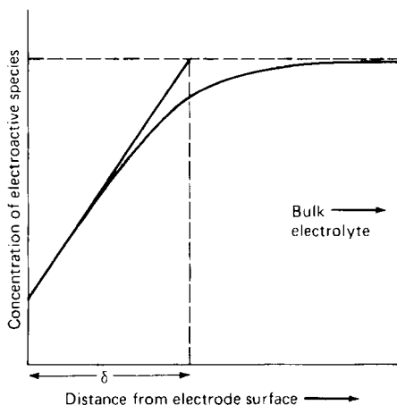
FIGURE 2.15 Boundary-layer thickness at an electrode surface.
