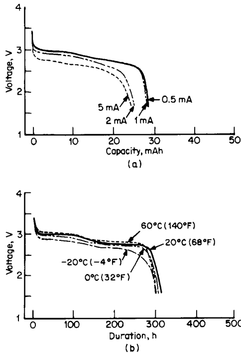
FIGURE 34.41 Discharge characteristics of a LiAl/V 2 O 5 coin-type battery (VL2020 size): (a) discharges at 20°C, (b) discharges at 30 kΩ at various temperatures. (From Panasonic Division of Matsushita Electric Corp. of America.)
