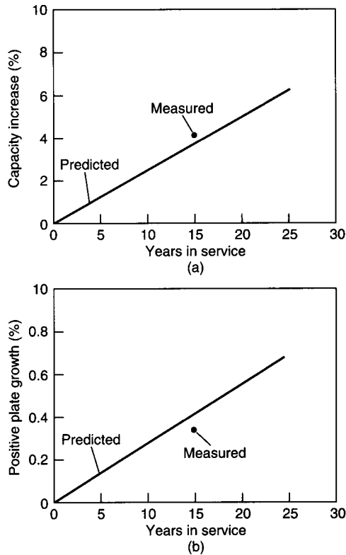
FIGURE 23.37 (a) Capacity after 15 years in service vs. prediction from accelerated testing. (From Bi-agetti. 28 ) (b) Positive-plate growth after 15 years in service vs. prediction from accelerated testing.
