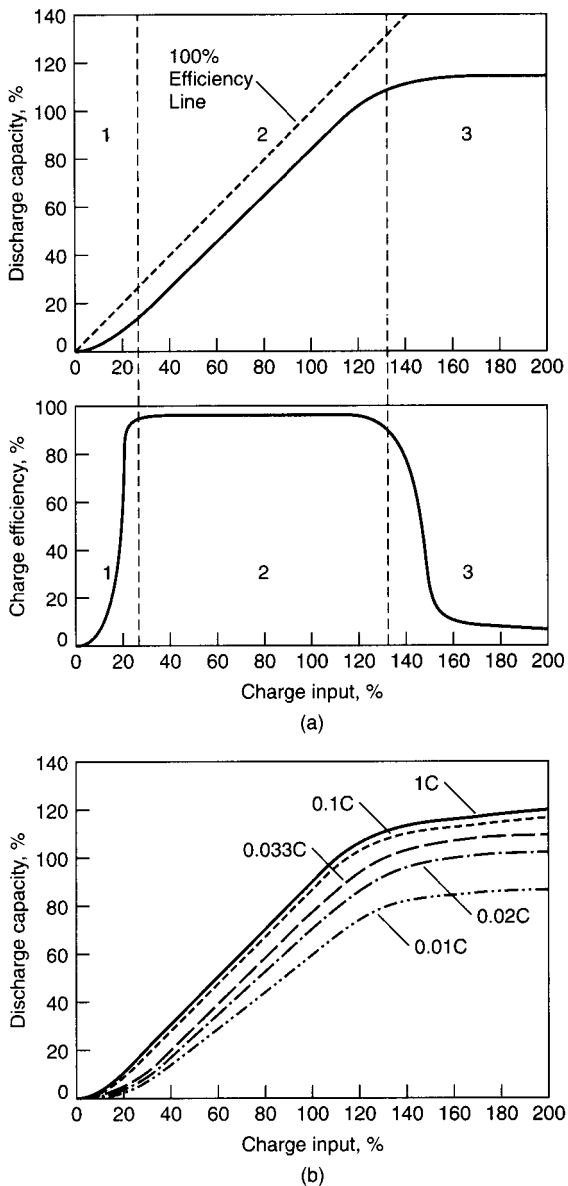
FIGURE 28.27 Charge process of sealed nickel-cadmium batteries. (a) Charge efficiency at 20°C. Charge—0.1C × 16 h; discharge—0.2°C; end voltage—1 V. (b) Charge efficiency vs. charge rate at 20°C.
