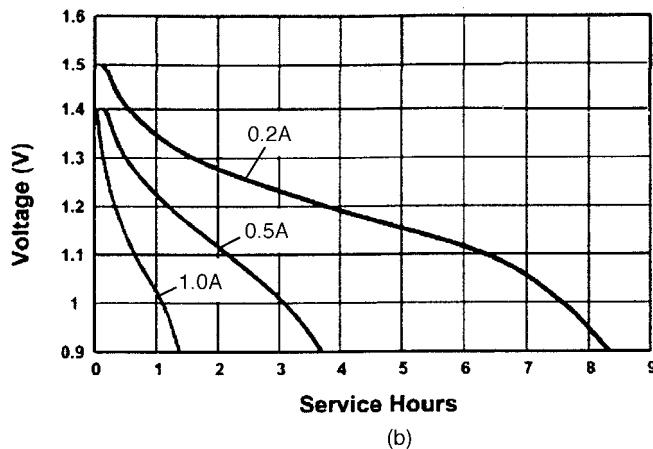
FIGURE 10.22 Performance characteristics of premium zinc/alkaline/manganese dioxide primary batteries AA-size at 20°C. (a) Discharge characteristics at various power drains. (b) Discharge characteristics at various current drains.
