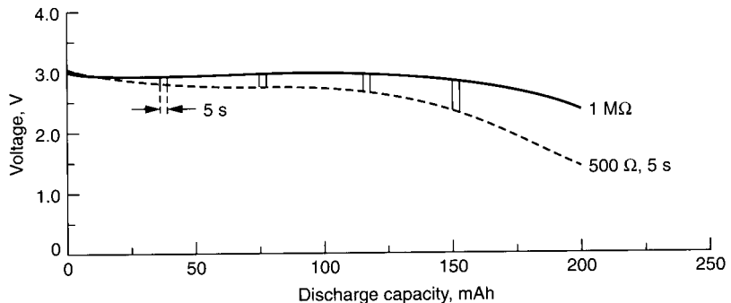
FIGURE 14.44 Pulse characteristics of Li/MnO 2 coin-type battery (190-mAh size) at 20°C. Test conditions: continuous load—1 MΩ ≈ 3 μA; pulse load—500 Ω ≈ 5.5 mA; duration—5 s; pulses—4; time between pulses—3 h. (Courtesy of Duracell, Inc.)
