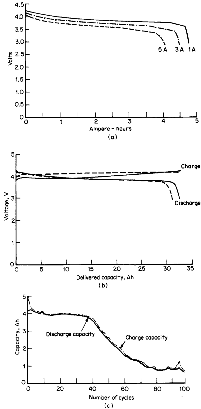
FIGURE 34.19 (a) Discharge characteristics of a 5-Ah \text{Li}/\text{Li}_2\text{CoO}_2 D-size battery at 20^\circ\text{C} . (Delivered specific energy at 1.0 A, 70 Wh/lb.) (b) Effect of charging rates on discharge performance of 30-Ah \text{Li}/\text{Li}_2\text{CoO}_2 battery at 20^\circ\text{C} . - - -, constant potential at 4.20 V [current limit at 5.0 \text{mA}/\text{cm}^2 ( C/2 )]. —, constant current at 1.0 \text{mA}/\text{cm}^2 ( C/10 ). Discharge rate at C/6 . (c) Cycle life characteristics of a \text{Li}/\text{Li}_2\text{CoO}_2 D-size battery. Charge at 300 mA, 4.3 V. Discharge at 3 A, 3.0 V. (From Alliant Technologies.).
