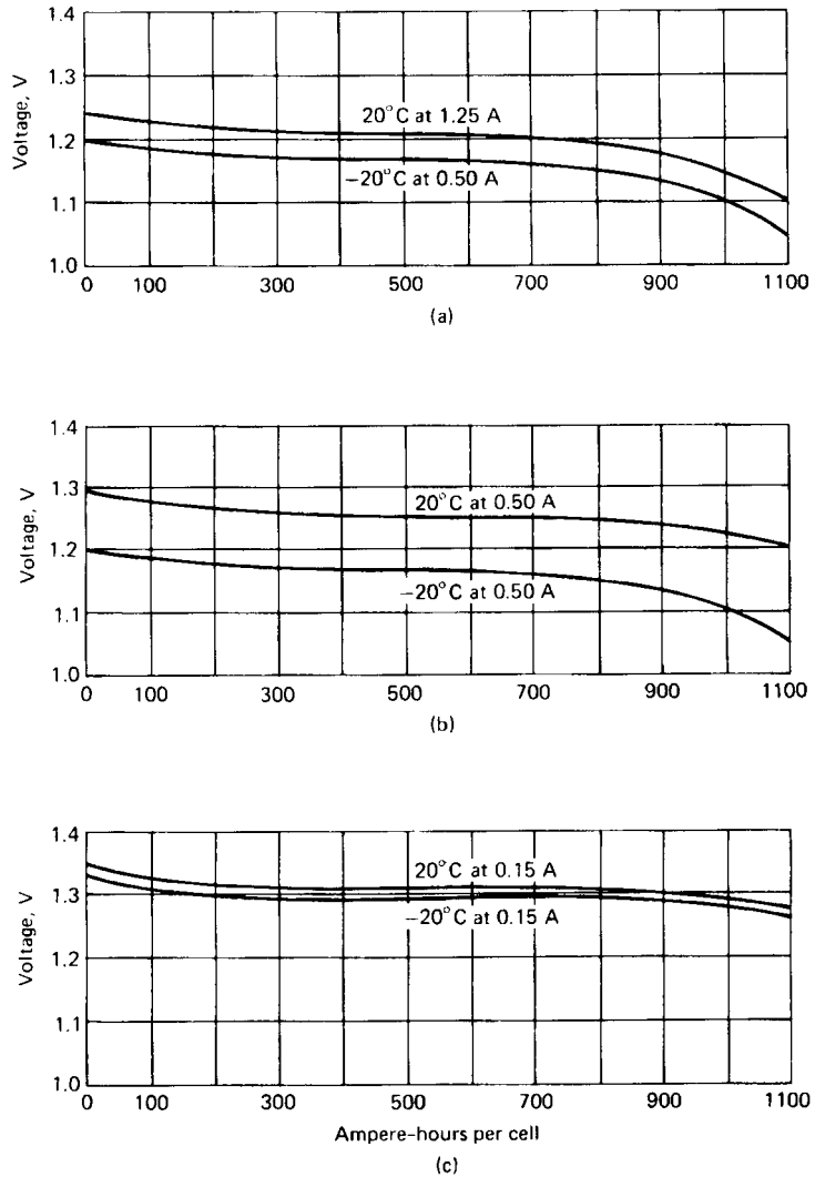
FIGURE 38.14 Typical discharge characteristics of Carbonaire 1100-Ah zinc/air batteries. (a) Maximum continuous rates. (b) Moderate continuous rates. (c) Low continuous rates. (Courtesy of SAFT America, Inc.)
