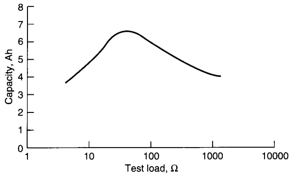
FIGURE 9.8 1LM service life (ampere-hours to 0.8 V) vs. test load. (Courtesy of Rayovac Corporation.)
