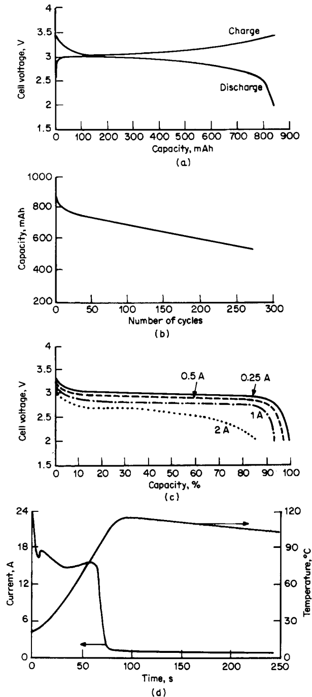
FIGURE 34.16 Performance characteristics of Li/Li 0.3 MnO 2 rechargeable AA-size battery. (a) Charge and discharge curves. I_c = 250 mA; I_d = 250 mA (cycle no. 5). (b) Capacity vs. cycle number. I_c = 60 mA; I_d = 250 mA (100% DOD). (c) Capacity vs. discharge rate. (d) Short-circuit behavior after 50 cycles. (From Tadiran Electronic Industries, Inc.).
