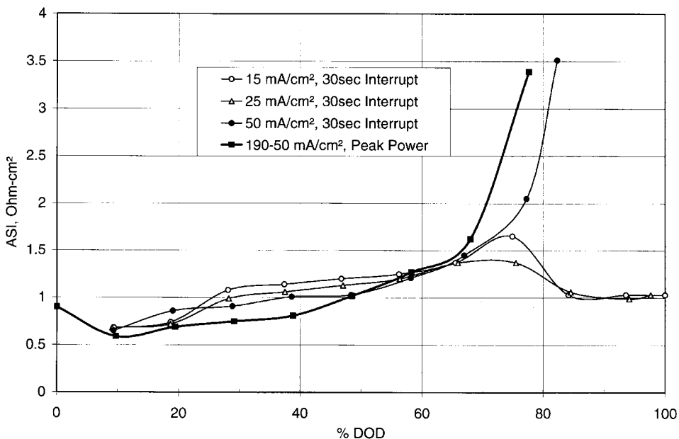
FIGURE 41.9 ASI vs. DOD for a 3-cm diameter cell with FeS 2 positive electrode. ASI determined from 30-second current interrupts at various discharge current rates and also from USABC peak power test. (From Henriksen, et al. 8 )
