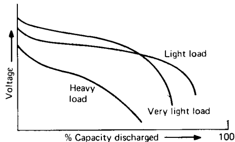
FIGURE 3.24 Effect of self-discharge on battery capacity.
