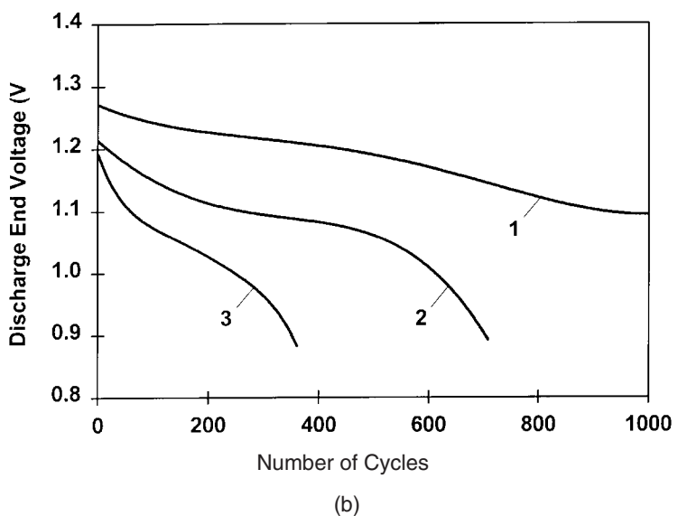
FIGURE 36.7 (a) Discharge characteristics of rechargeable zinc/alkaline/manganese dioxide AA-size batteries after cycling at 20°C. Cells discharged 4h per day at 10 Ω; 1.65 V constant voltage charging overnight. (b) The cycle life of AA-size batteries on a 10 Ω load. Curve 1 discharged for 200 mA, then recharged; curve 2 discharged for 300 mA then recharged; curve 3 Discharged for 400 mA, then recharged. (Courtesy of Battery Technologies, Inc.)
