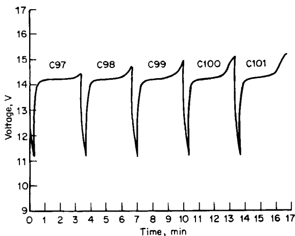
FIGURE 34.35 Discharge/charge behavior of a bipolar Li/CuCl 2 battery (four-cell stack) at 50-mA/cm 2 (total 24 A) discharge for 20 s and 5.56-mA/cm 2 charge for 180 s. Voltage limits: 11.0–16.0 V. (From Yardney Technical Products, Inc.)
