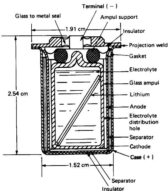
FIGURE 20.3 Cross section of Li/V 2 O 5 reserve cell. Alliant model G2659. (Courtesy of Alliant Techsystems, Inc.)
