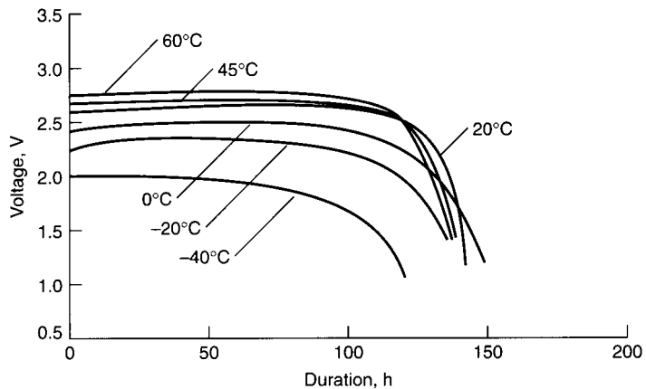
FIGURE 14.69 Typical discharge curves of Li/(CF) n cylindrical battery at various temperatures; rated capacity 1.2 Ah; 300-Ω discharge load. (Courtesy of Panasonic, Division of Matsushita Electric Corp. of America.)
