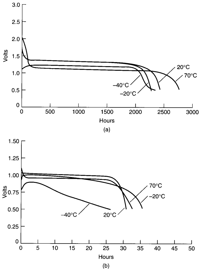
FIGURE 14.93 Performance of high- and low-rate Li/CuO D-size batteries. (a) Discharge at 147 Ω. (b) Discharge at 1.5 Ω.
