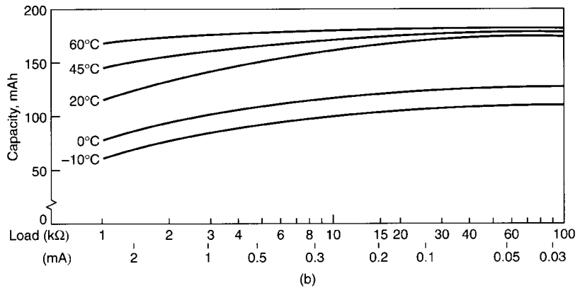
FIGURE 14.66 Discharge characteristics of Li/(CF) n coin-type battery (165-mAh size). (a) Operating voltage vs. discharge load; voltage at 50% discharge. (b) Capacity vs. discharge load; cutoff at 2.0 V. (Courtesy of Panasonic, Division of Matsushita Electric Corp. of America.)
