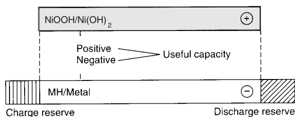
FIGURE 29.1 Schematic representation of electrodes of sealed nickel-metal hydride cell, divided into useful capacity, charge reserve, and discharge reserve. (Courtesy of Duracell, Inc.)
