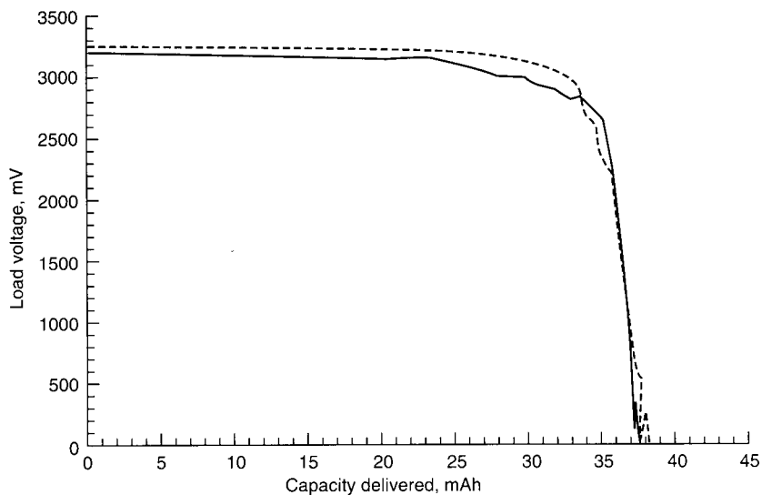
FIGURE 15.23 64.9-k \Omega constant load discharge of Ag/RbAg 4 I 5 /Me 4 NI 6 batteries after 20 years of storage at 25°C. Discharge temperature: solid curve—25°C; dashed curve—60°C. (From Ref. 29.)
