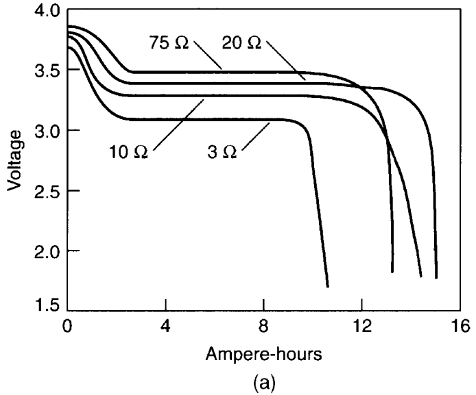
FIGURE 14.36 Performance characteristics of Li/SOCl 2 with BrCl-additive, D-size batteries. (a) Discharge characteristics at 20°C. (Courtesy of Electrochem Industries, Div., Wilson Greatbatch, Ltd.)
