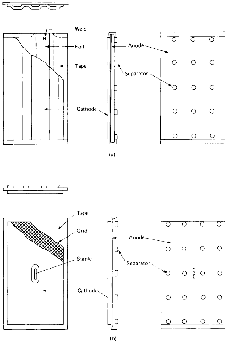
FIGURE 17.5 Duplex electrode assemblies. (a) Silver. (b) Nonsilver.
