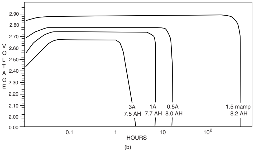
FIGURE 14.9(b) Discharge characteristics of high-rate Li/SO 2 D-size battery at four rates at 23°C. (Courtesy Hawker Eternacell, Inc.).
