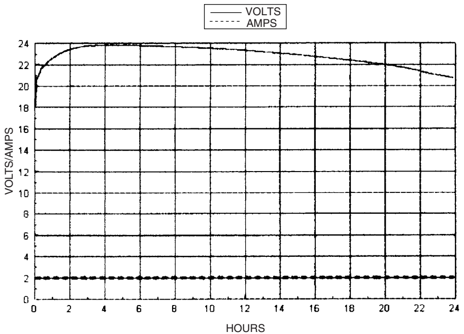
FIGURE 38.38 Sixteen cell SOFAL battery. (a) Constant current 2.0 Ampere discharge.
