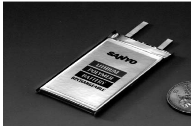
FIGURE 35.88 A 0.57 Ah polymer Li-ion battery. (Courtesy of Sanyo.)
