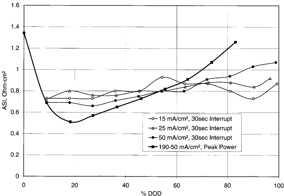
FIGURE 41.10 ASI vs. DOD for a 3-cm diameter cell with 12-mol % CoS 2 additive to the FeS 2 positive electrode. ASI determined from 30-second current interrupts at various discharge current rates and also from USABC peak power test. (From Henriksen, et al. 8 )
