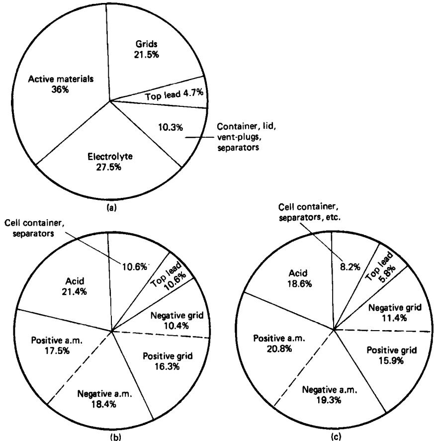
FIGURE 23.9 Weight analysis of typical lead-acid batteries. (a) SLI battery. (b) Tubular industrial battery. (c) Flat-plate traction battery. (From Ref. 10.)
