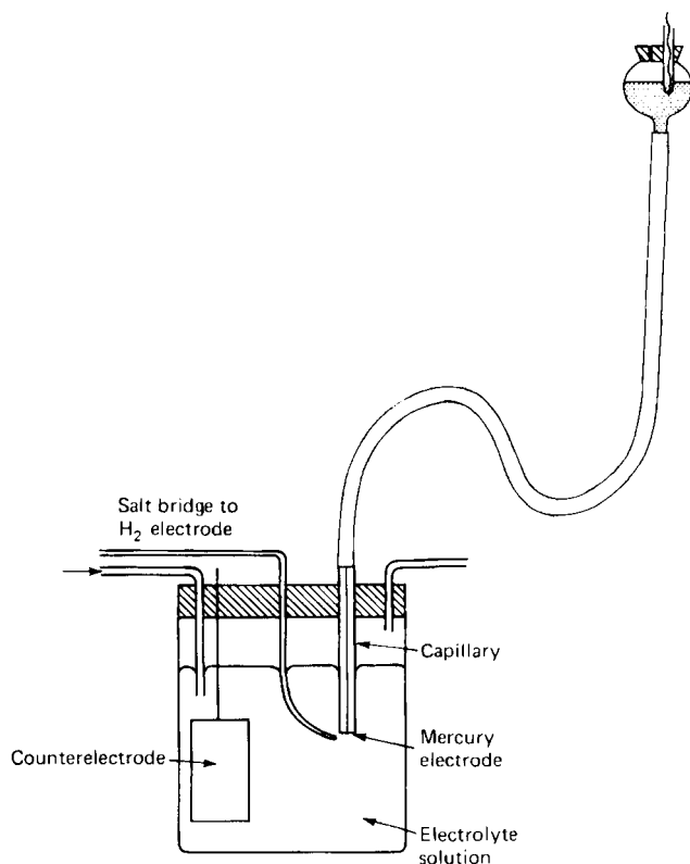
FIGURE 2.7 Experimental arrangement to measure interfacial surface tension at mercury-electrolyte interface.
