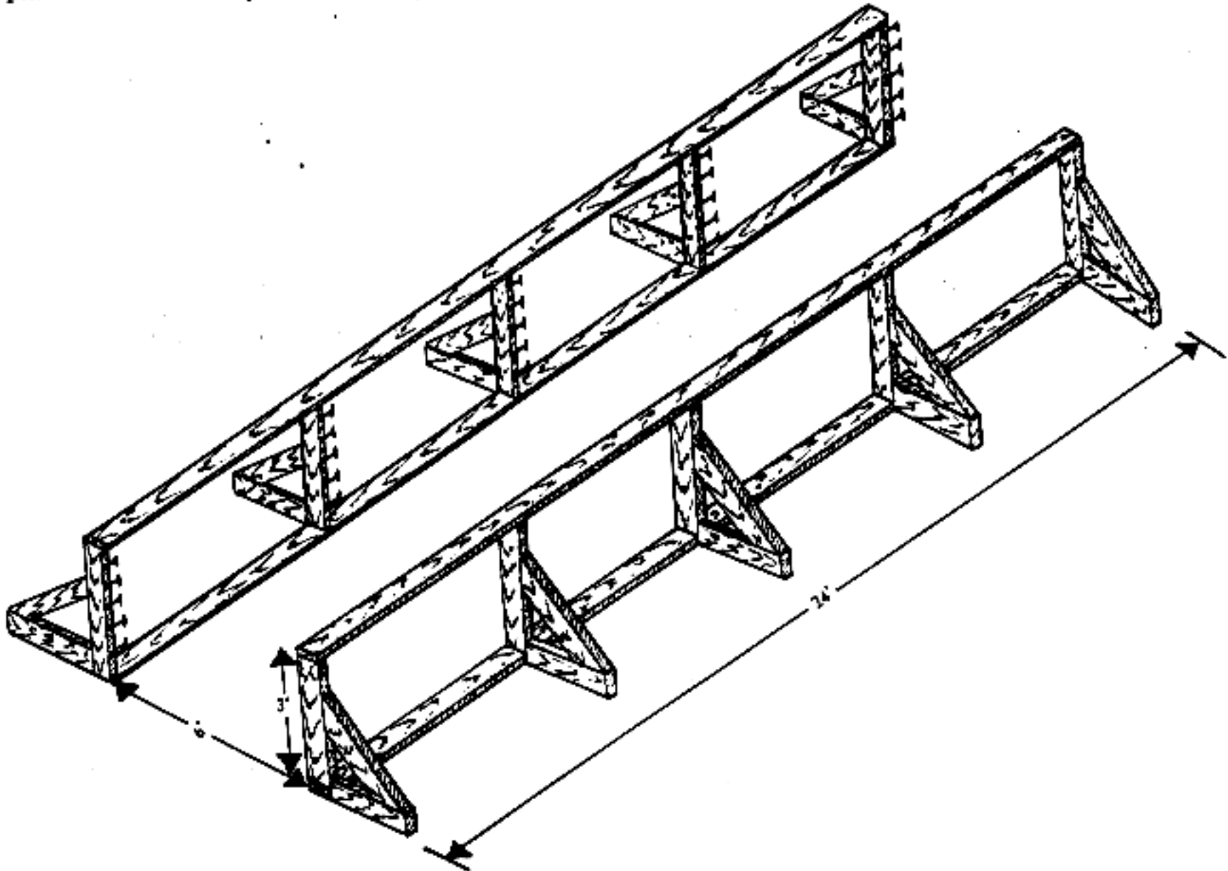
Figure 28. Tripwire training device.
