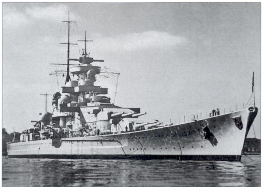
This view shows Gneisenau after her refit, now sporting the raked 'Atlantic' bow, which did little to cure her tendency to ship considerable amounts of water over her fo'c'sle at speed or in heavy seas. The angled funnel cap can just be seen by the base of her mainmast. That this is a pre-war photograph is confirmed by the presence of the ship's crest on the bow. It was removed on the outbreak of war.
