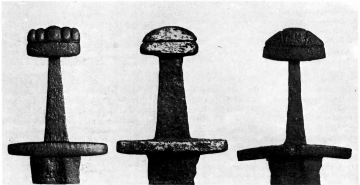
Sword hilts of the 10th and 11th centuries, showing the five-lobed, 'tea cosy' and 'walnut' types of pommels and (at the right) the curved guard of the 11th century.
