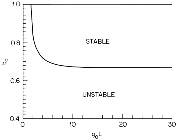
Figure 9.8 Stable and unstable regions of SBS in the presence of feedback. Solid line shows the critical value of the relative Stokes intensity [ b_0 = I_s(0)/I_p(0) ] below which the steady state is unstable. (After Ref. [45].)
