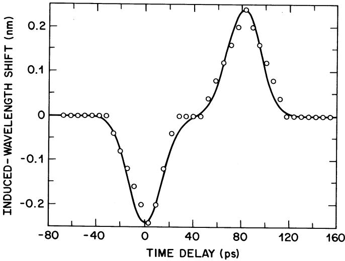
Figure 7.4 XPM-induced wavelength shift of a 0.53\text{-}\mu\text{m} probe pulse as a function of the initial time delay of the 1.06\text{-}\mu\text{m} pump pulse. Open circles show the experimental data while the solid line shows the theoretical prediction. (After Ref. [46].)
