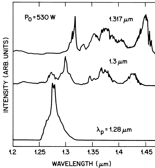
Figure 8.16 Pulse spectra at the output of a 150-m-long fiber when 0.83-ps input pulses are launched with the peak power P_0 = 530 W. The zero-dispersion wavelength of the fiber is 1.317 \mu\text{m} . (After Ref. [176] ©1987 IEEE.)
