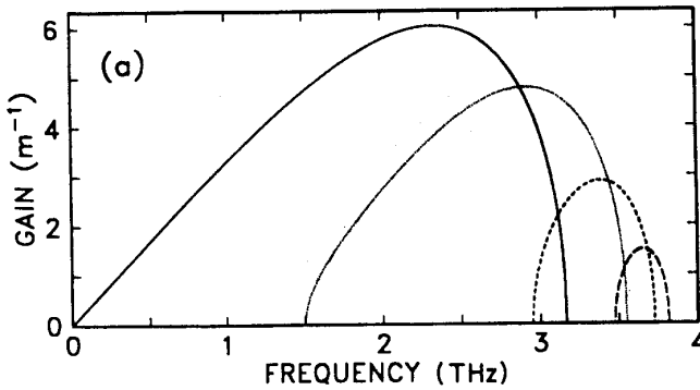
Figure 6.10 Gain spectra of modulation instability in a high-birefringence fiber when input beam is linearly polarized at 45° from the slow axis. Four curves correspond to (smallest to largest) for power levels of 60, 125, 250, and 500 W. (After Ref. [50].)
