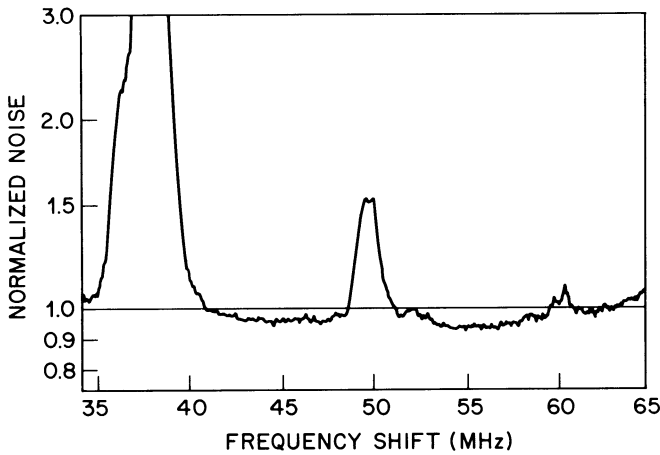
Figure 10.12 Noise spectrum under minimum-noise conditions. Horizontal line shows the quantum-noise level. Reduced noise around 45 and 55 MHz is a manifestation of squeezing in optical fibers occurring as a result of FWM. (After Ref. [103].)
