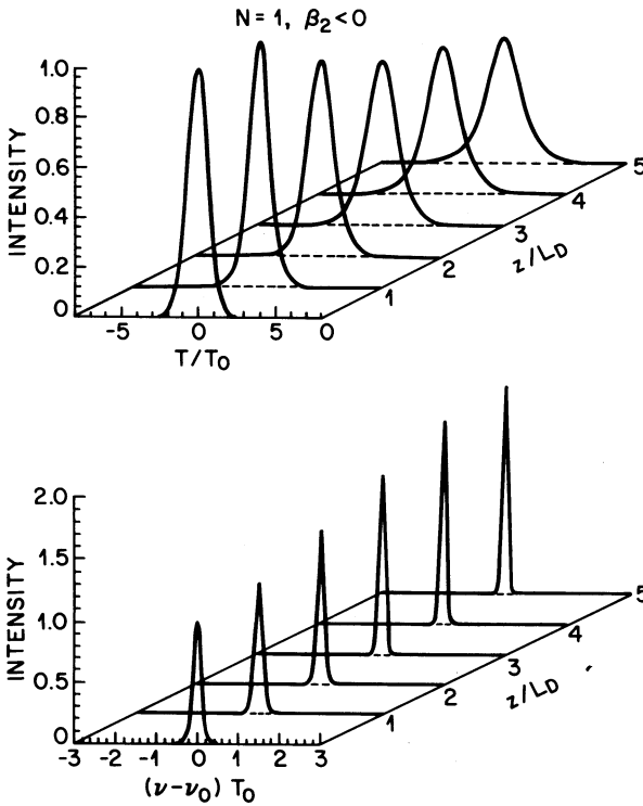
Figure 4.8 Evolution of pulse shapes (upper plot) and optical spectra (lower plot) under conditions identical to those of Fig. 4.7 except that the Gaussian pulse propagates in the anomalous-dispersion regime ( \beta_2 < 0 ).
