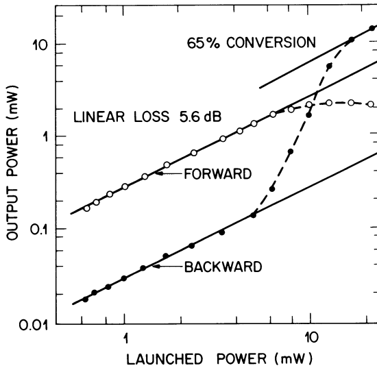
Figure 9.6 Transmitted (forward) and reflected (backward) powers as a function of the input power launched into a 13.6-km-long single-mode fiber. (After Ref. [30].)
