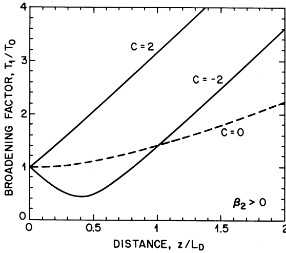
Figure 3.2 Broadening factor for a chirped Gaussian pulse as a function of distance. Dashed curve corresponds to the case of an unchirped Gaussian pulse. For \beta_2 < 0 , the same curves are obtained if the sign of C is reversed.
