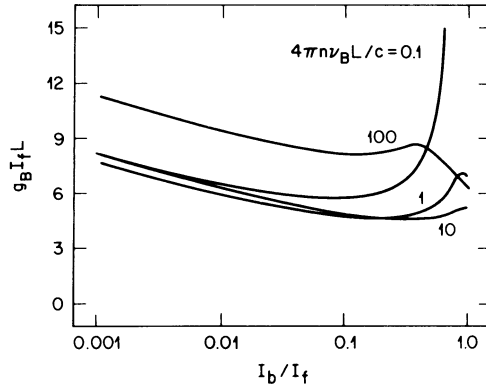
Figure 9.10 Threshold of SBS-induced modulation instability for counterpropagating pump waves of input intensities I_f and I_b . Normalized forward intensity is plotted as a function of I_b/I_f for \Delta\nu_B/\nu_B = 0.06 for several fiber lengths. (After Ref. [50].)
