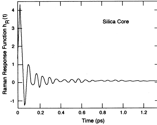
Figure 2.2 Temporal variation of the Raman response function h_R(t) obtained by using the actual Raman-gain spectrum of silica fibers. (After Ref. [16].)
