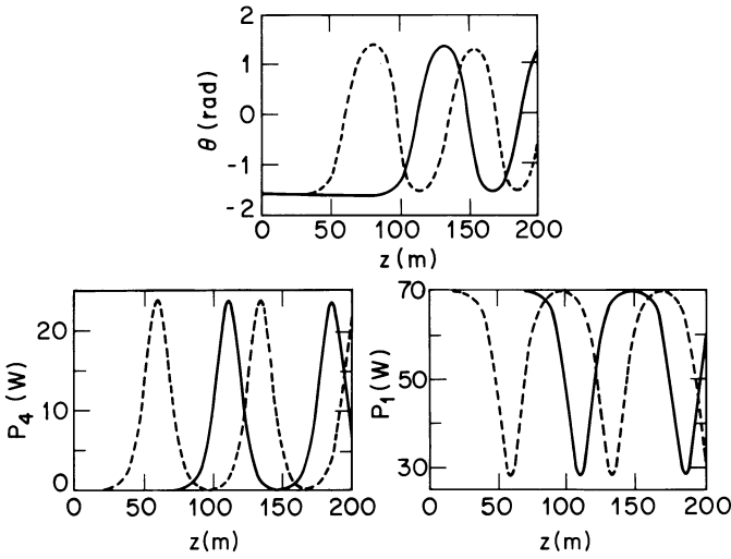
Figure 10.10 Evolution of relative phase \theta , idler power P_4 , and pump power P_1 along fiber length when \kappa = 0 . Input parameters correspond to P_1 = P_2 = 70 W, P_4 = 0.1 \mu\text{W} , and \theta = \pi/2 . Input signal power P_3 = 0.1 \mu\text{W} for solid curves and 6 mW for dashed curves. (After Ref. [70] ©1987 IEEE.)
