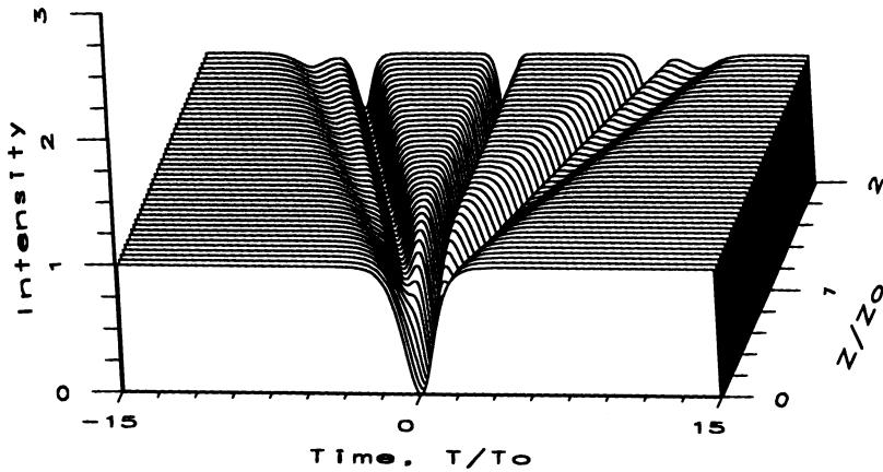
Figure 5.9 Evolution of a third-order dark soliton showing narrowing of the central dip and creation of two pairs of gray solitons.
