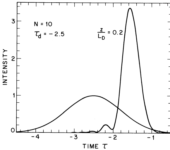
Figure 7.8 XPM-induced pulse compression in the normal-dispersion region of an optical fiber realized using a pump pulse of peak power such that N = 10 . Shape of input pulses is also shown for comparison. (After Ref. [47].)
