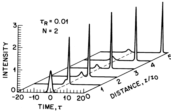
Figure 5.18 Decay of a second-order soliton ( N = 2 ) induced by intrapulse Raman scattering ( \tau_R = 0.01 ).
