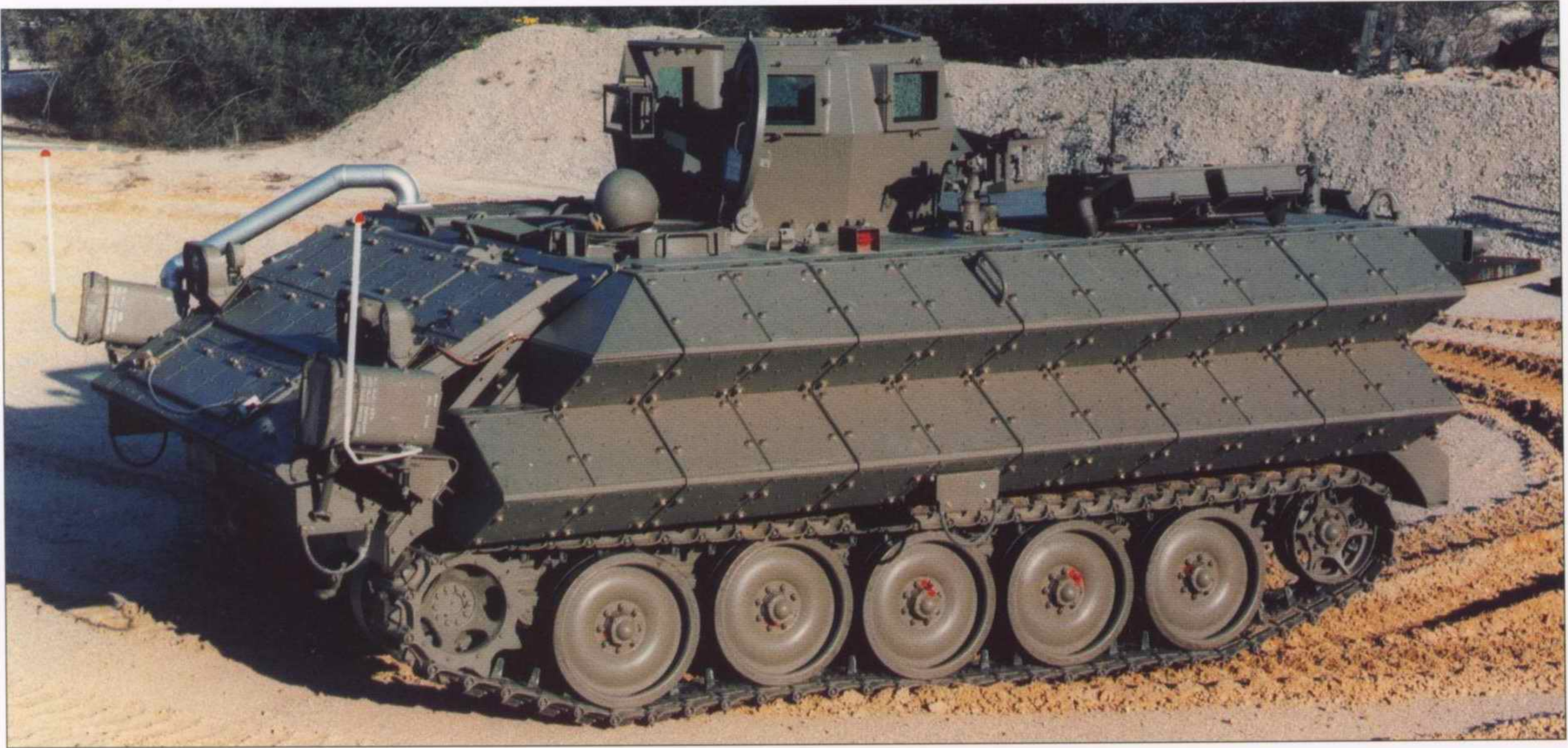
ABOVE The ultimate M113 armour upgrade, the Classical, circa 1997. Lightweight explosive reactive armour tiles offer protection against HEAT warheads. The roof-mounted 'birdcage' protects exposed crewmen against small arms fire. (Rafael)
