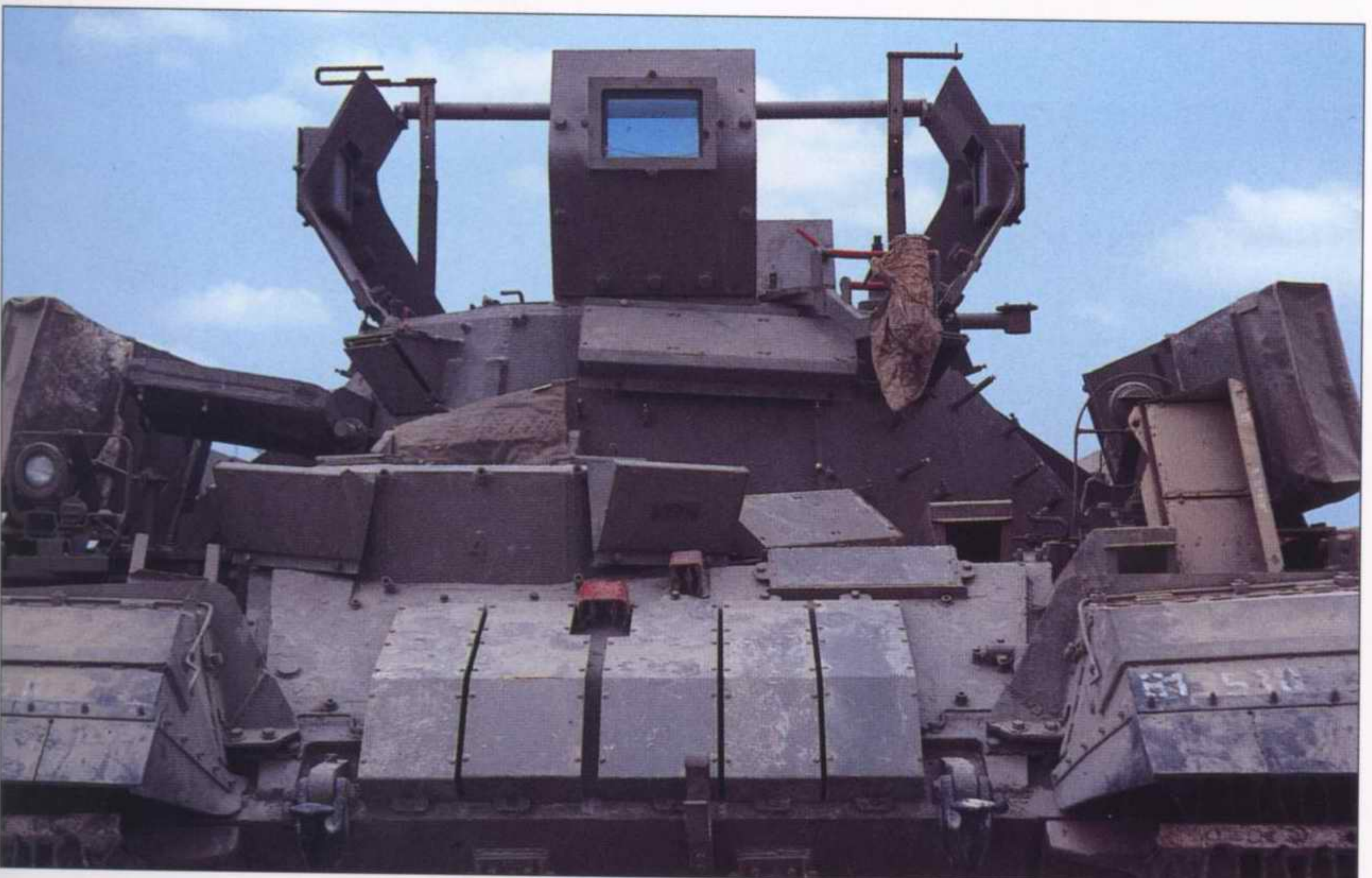
The front of the Nagmachon, close up. Note the cluttered untidy appearance and the ERA blocks on the glacis. The machine has two smoke grenade launchers in situ. There are empty brackets awaiting the other two launchers.
