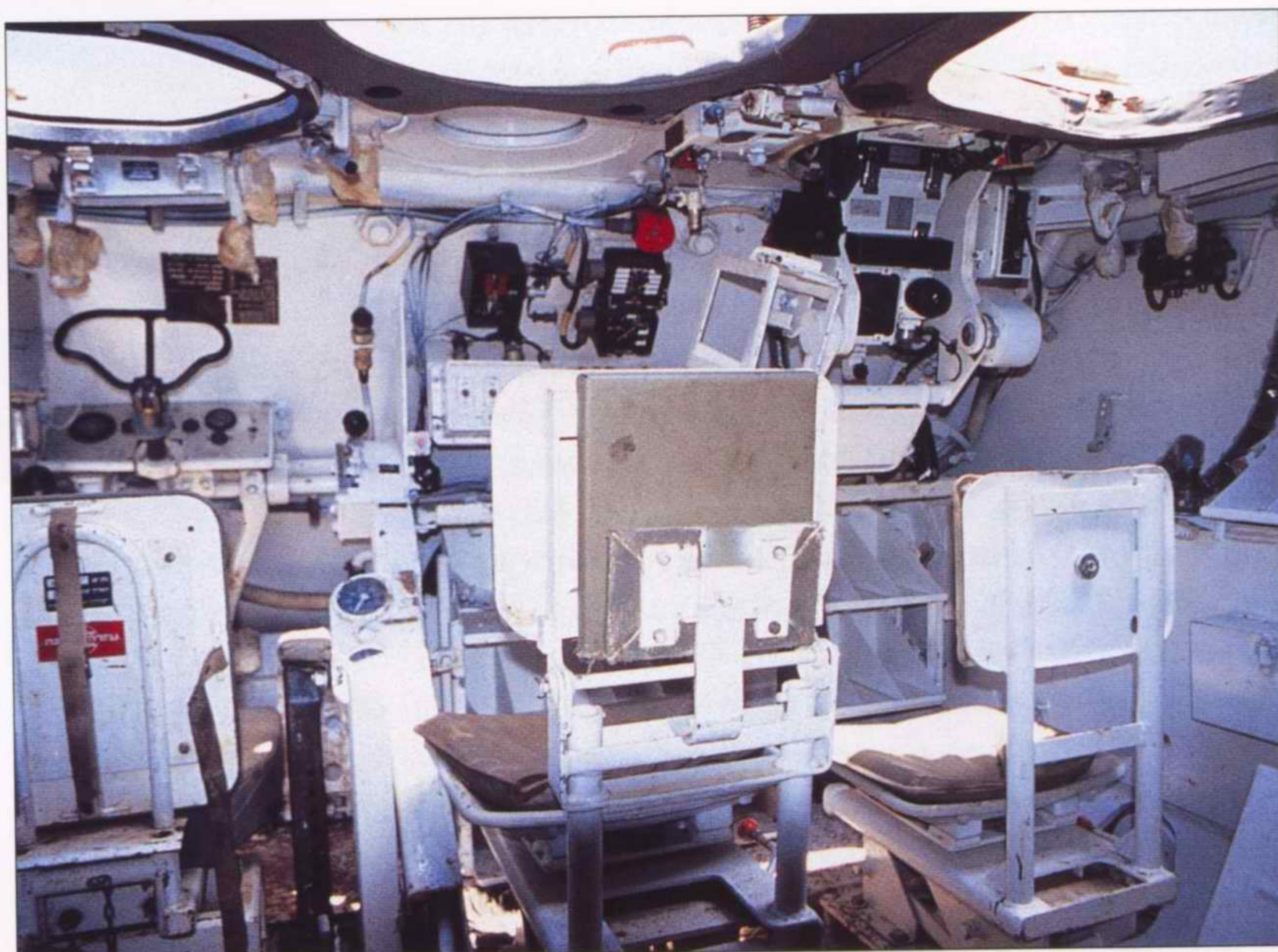
The interior of an Achzarit, photographed on the Golan Heights in 1997. From left to right are the driver's, commander's and gunner's stations.
