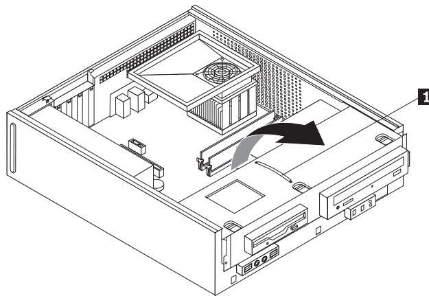
Figure 8. Removing the drive bay assembly
