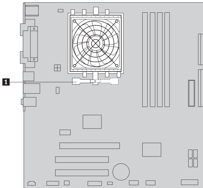
Figure 31. Clamping the heat sink to the plastic retention bracket
