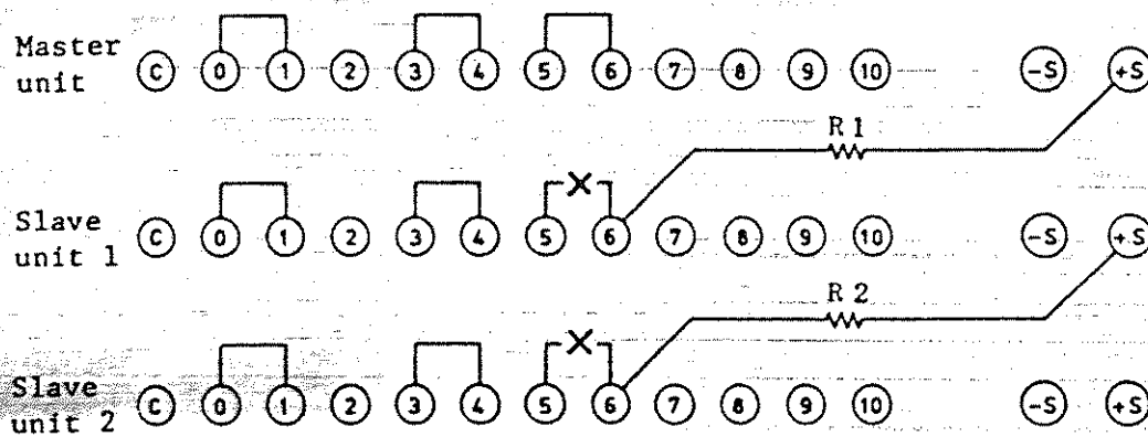
Figure 4-12. Rear terminal connections
