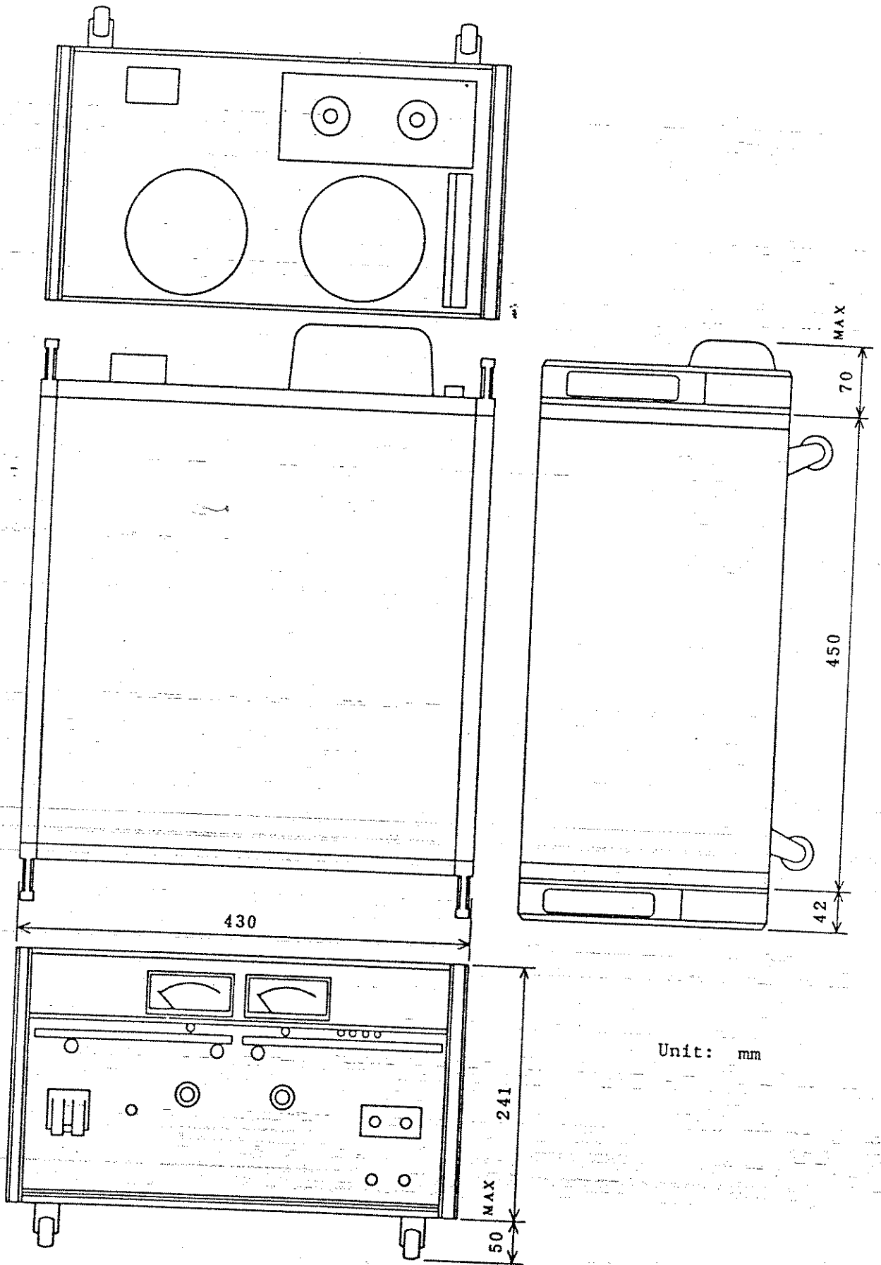
Figure 1-1. Mechanical Outline Drawing
