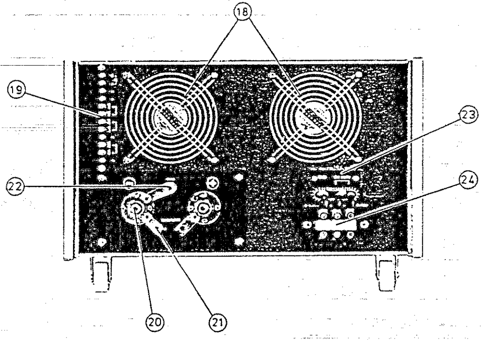
Figure 2-6. Front and Rear Panel
