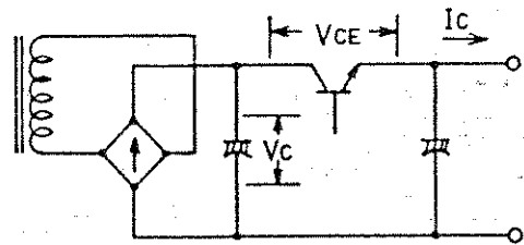
Figure 5-1 Series-controlled power supply
