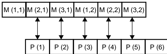
Figure 4-1 Storage Representation of an EQUIVALENCE Statement
