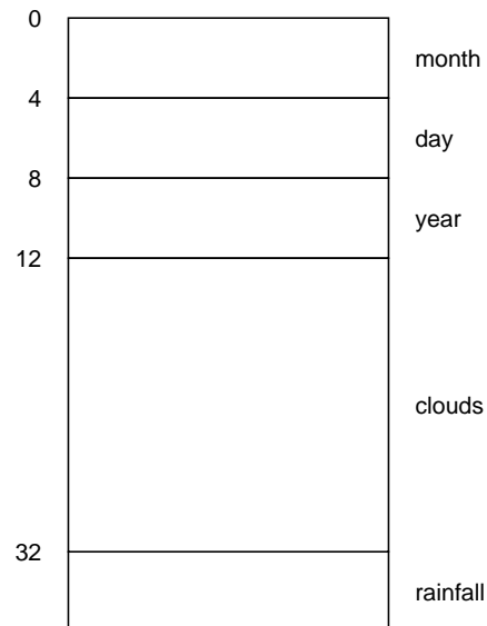
Figure 4-3 Logical Representation of a STRUCTURE Statement
