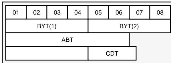
Figure 4-2 Logical Representation of an EQUIVALENCE Statement
