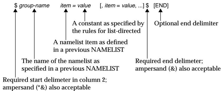
Figure 8-1 Namelist Input Data Rules
