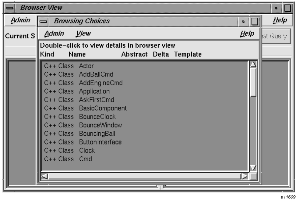
Figure 7-1 Browsing Windows
