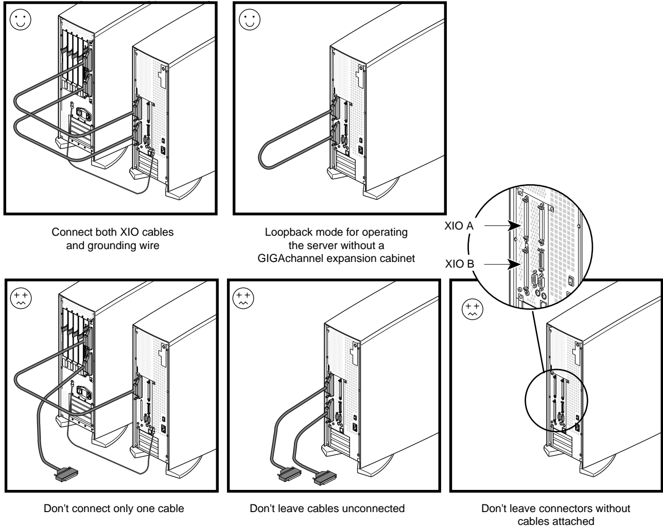
Figure 1 Correct and Incorrect XIO Connector Cabling for Origin200 GIGAchannel
