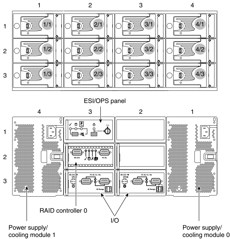
Figure 1-20 Module Locations and Bay Numbering: Rackmount Enclosure
