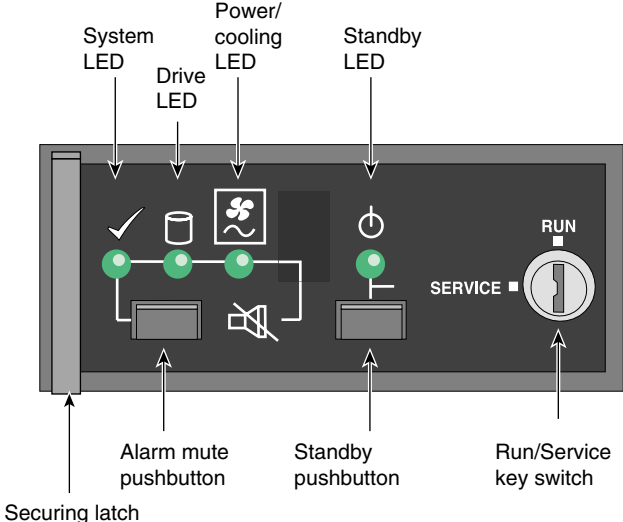
Figure 1-10 ESI/Ops Panel Indicators and Switches: Rackmount Enclosure
