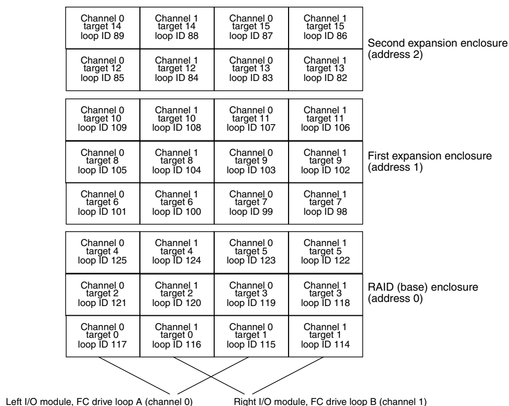
Figure 4-3 I/O Modules, Channels, and Loops: Rackmount Enclosure
