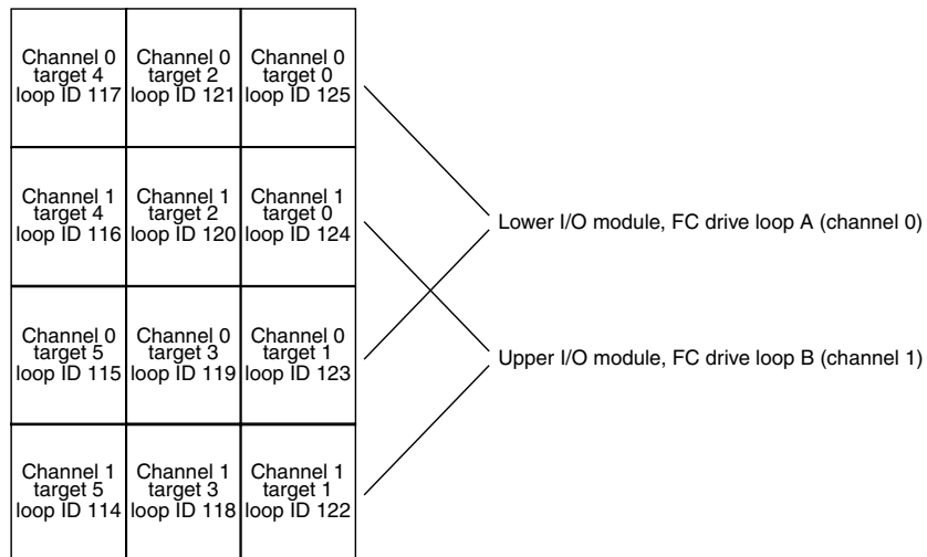
Figure 4-2 I/O Modules, Channels, and Loops: Tower
