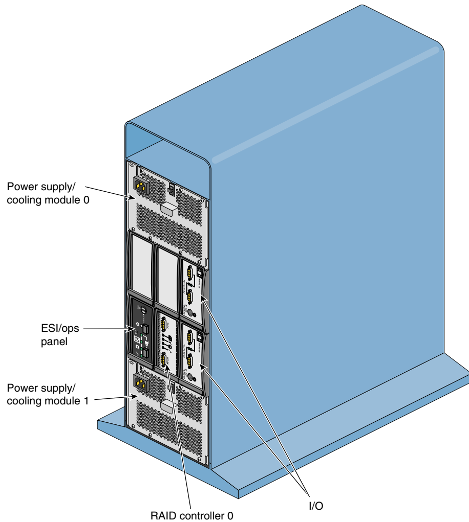
Figure 1-7 Tower, Rear View
