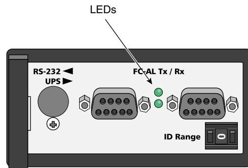
Figure 1-16 I/O Module Panel Features, Rackmount Enclosure
