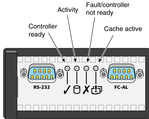
Figure 1-13 RAID Controller Panel Features: Rackmount Enclosure
