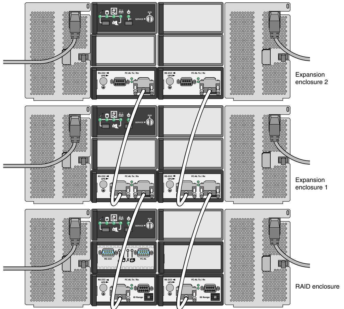
Figure 1-5 Expansion Enclosure Cabling
