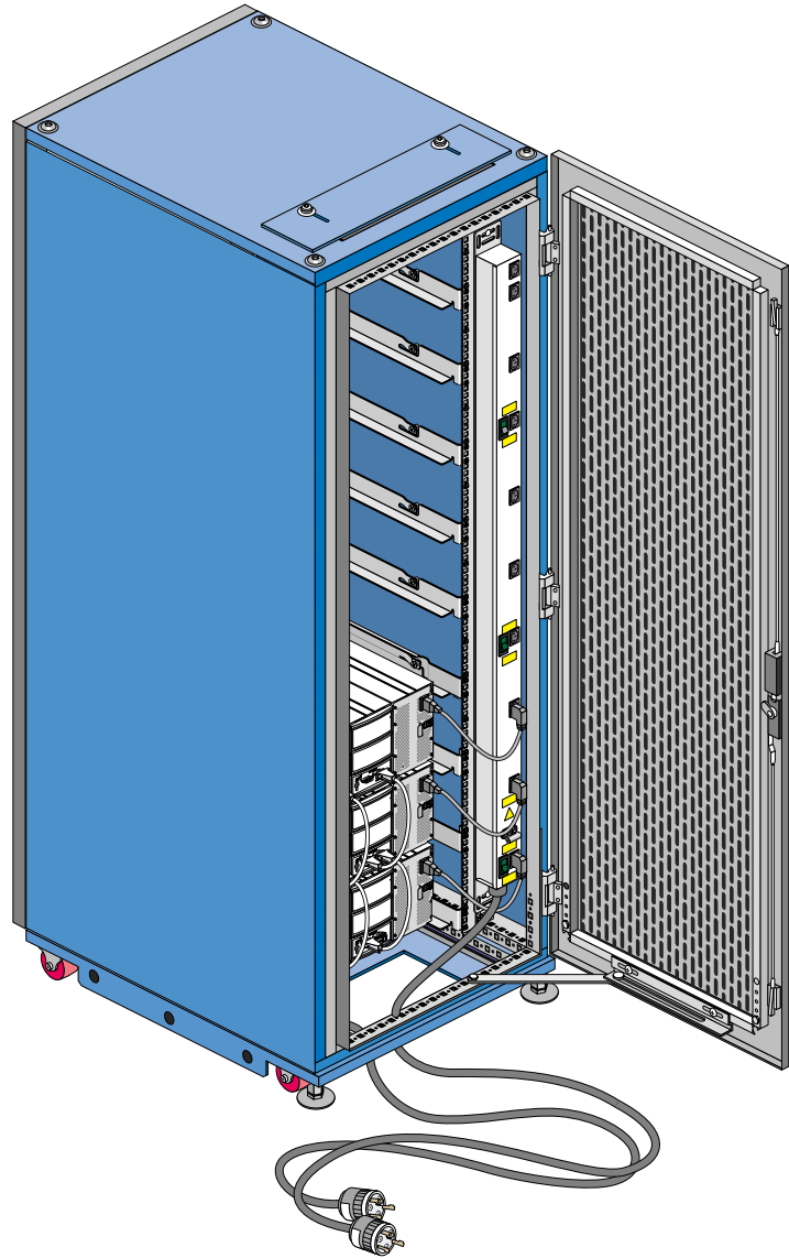
Figure 1-4 SGI TP 9100 Rack, Rear View, Example
