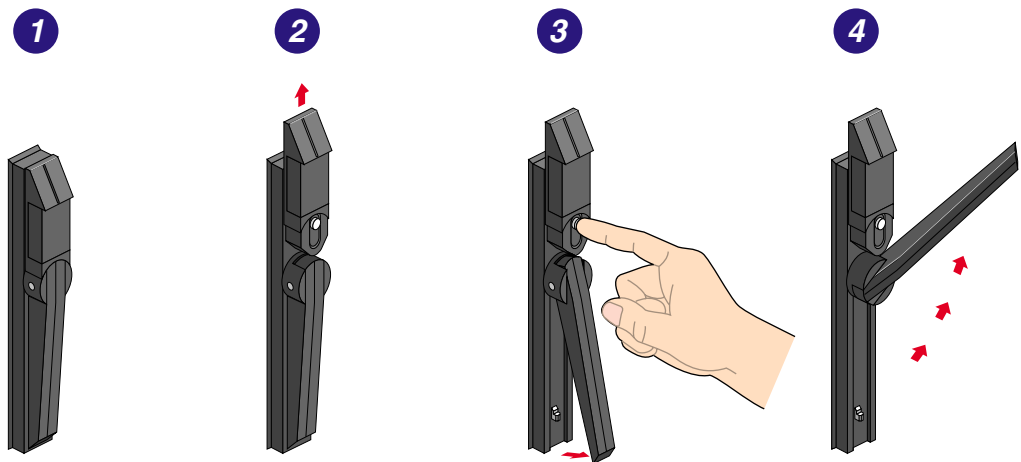
Figure 1-22 Opening the Rack Rear Door: Latch
