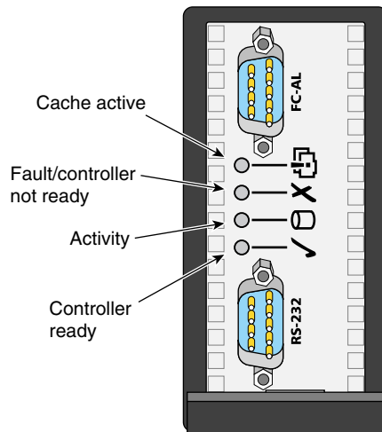
Figure 1-14 RAID Controller Panel Features: Tower
