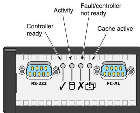
Figure 5-6 RAID Controller Panel LEDs: Rackmount Enclosure
