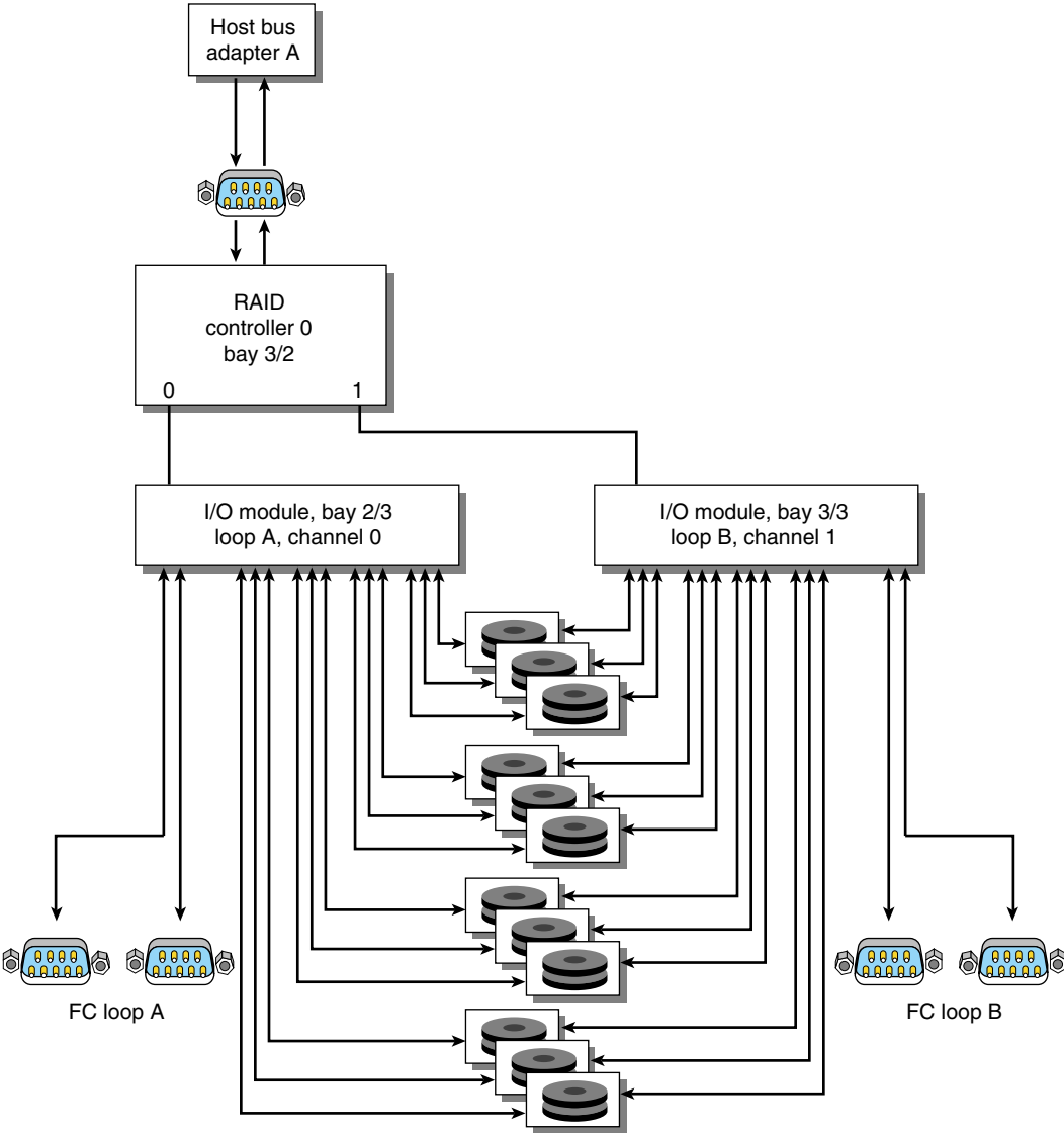
Figure 4-4 Single-Controller/Point-to-Point/Single-Host Example
