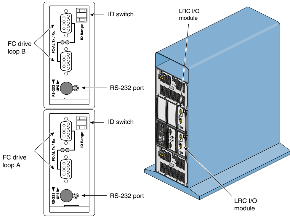
Figure 1-17 I/O Module Panel Features and Location, Tower
