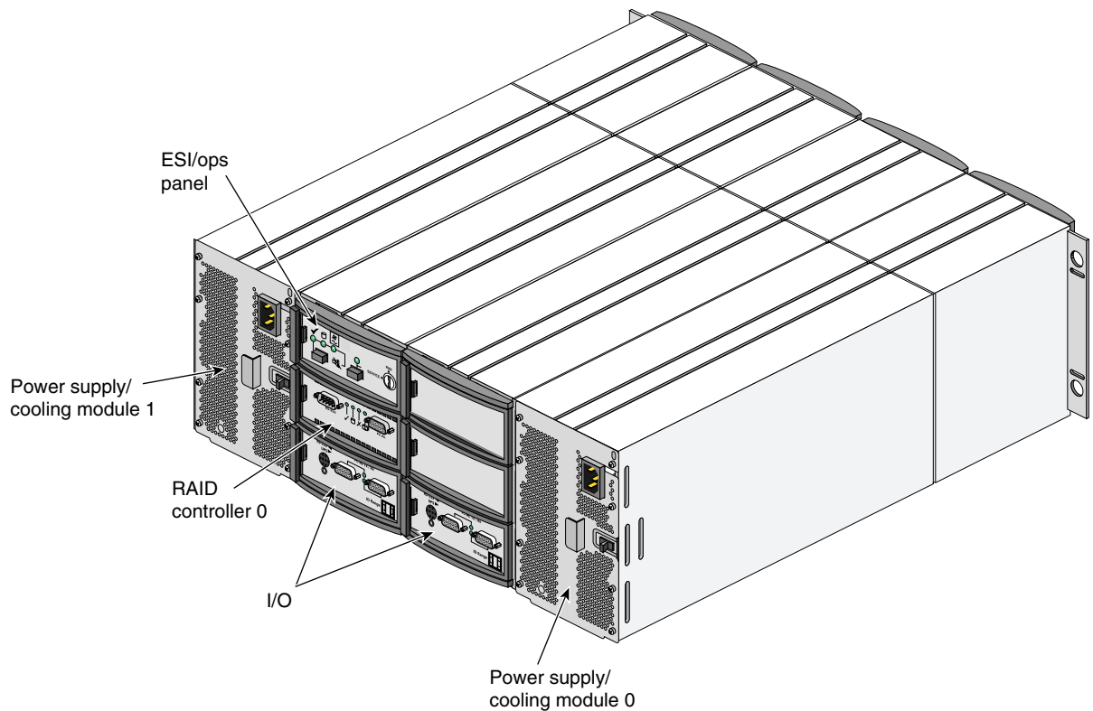
Figure 1-2 Rackmount Enclosure (RAID, or Base), Rear View
