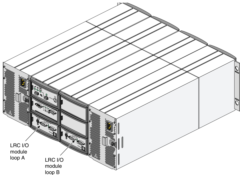
Figure 1-15 I/O Module Location, Rackmountable Enclosure
