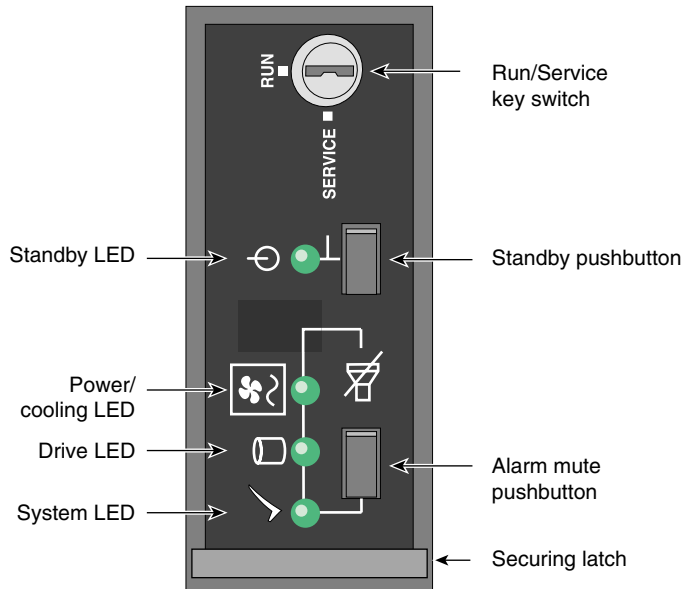
Figure 1-11 ESI/Ops Panel Indicators and Switches: Tower
