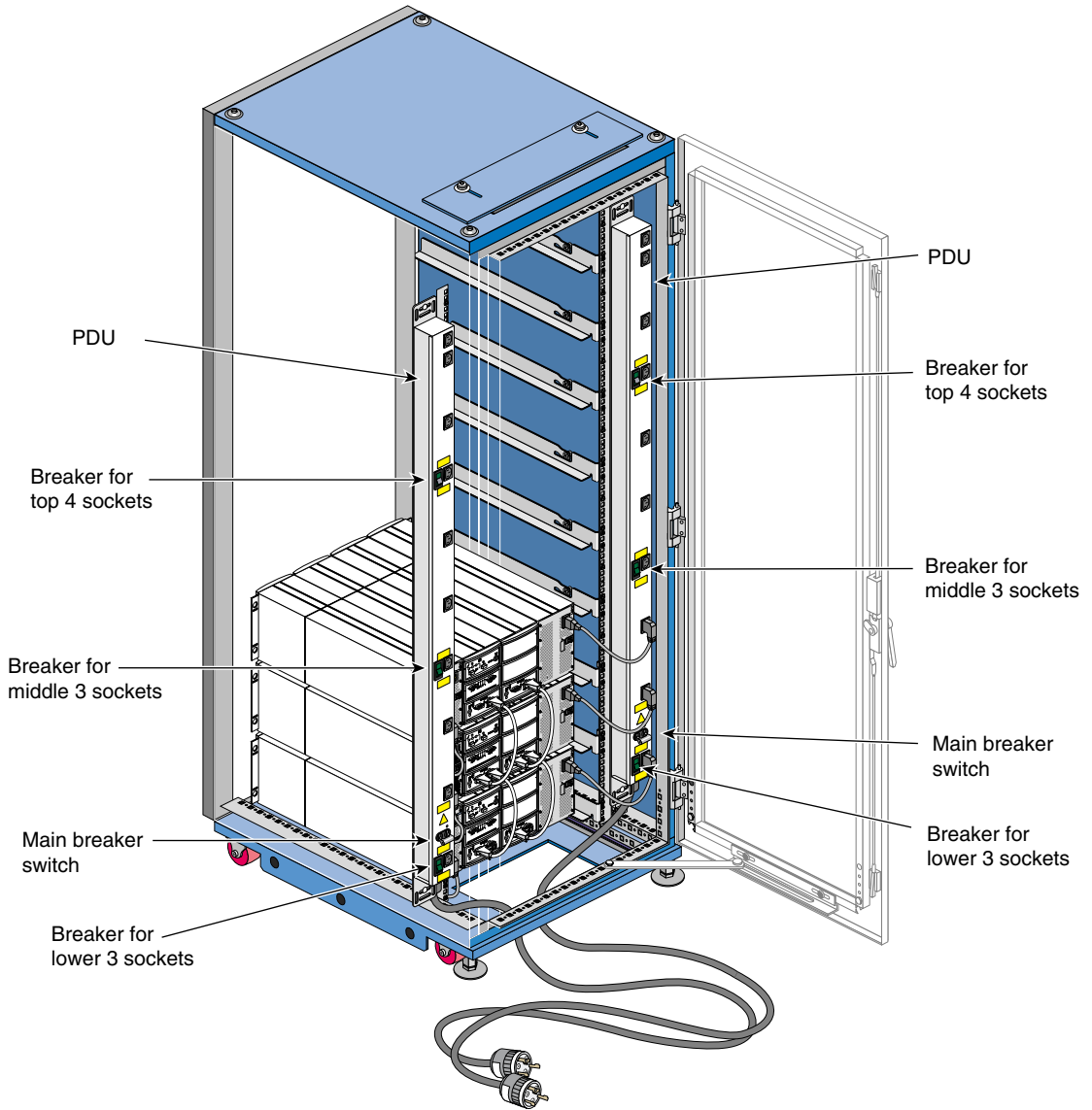
Figure 2-4 Rack Power Cabling
