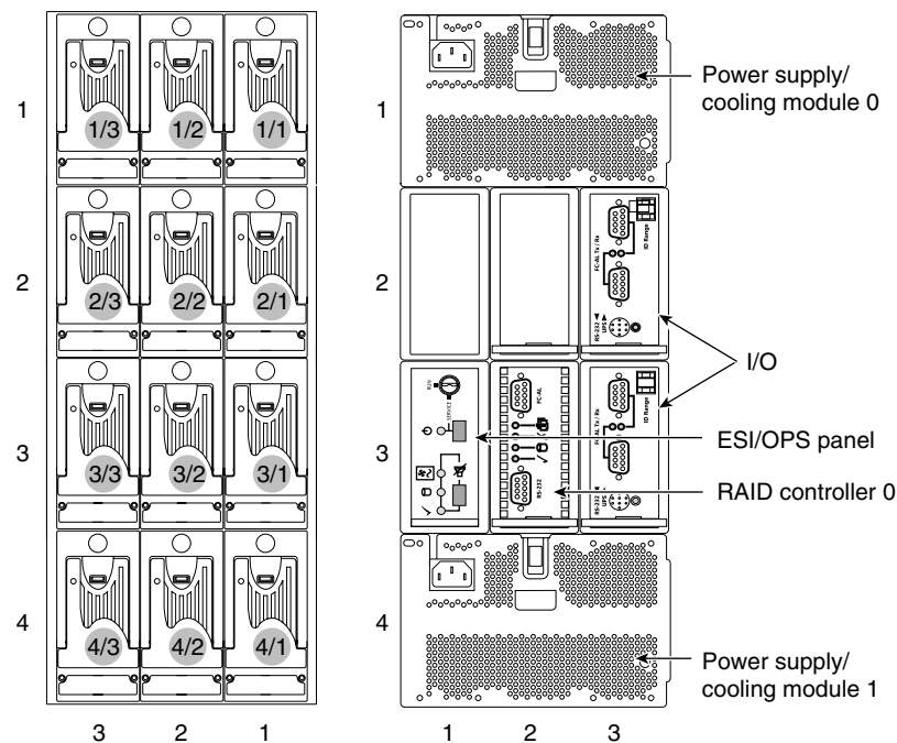
Figure 1-21 Module Locations and Bay Numbering: Tower
