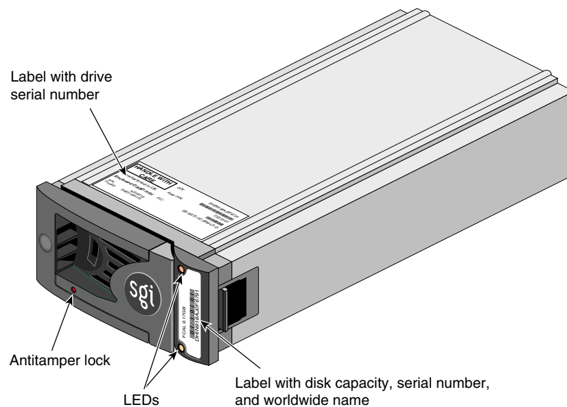
Figure 1-18 Disk Drive Module
