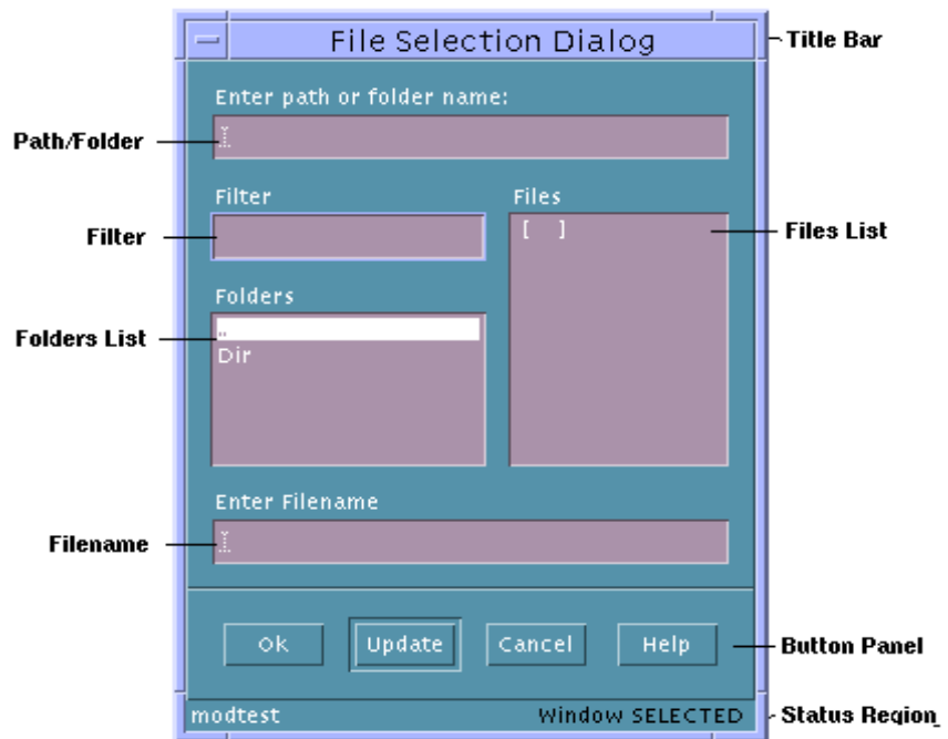
File Selection Dialog Object
