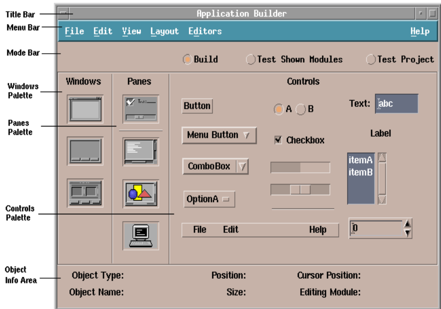
Figure 1-1 Application Builder primary window
