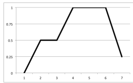
Figure 1: 1D piecewise-linear function.
