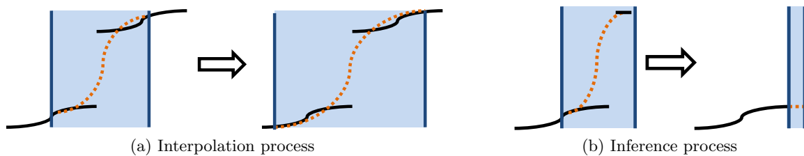
Figure 5: The transition process adaptively determines a trajectory in the low-dimensional space through interpolation. (a) The transition process decides an interval to interpolate a trajectory for transiting the two segments. If the interpolation process fails to find a smooth transition within the interval, the transition process expands the interval and performs interpolation again to find a smooth trajectory. (b) In the case that the process fails to find a smooth trajectory within the length limits, it will ignore the consecutive segment and infers a trajectory based on only the previous motion segment.
