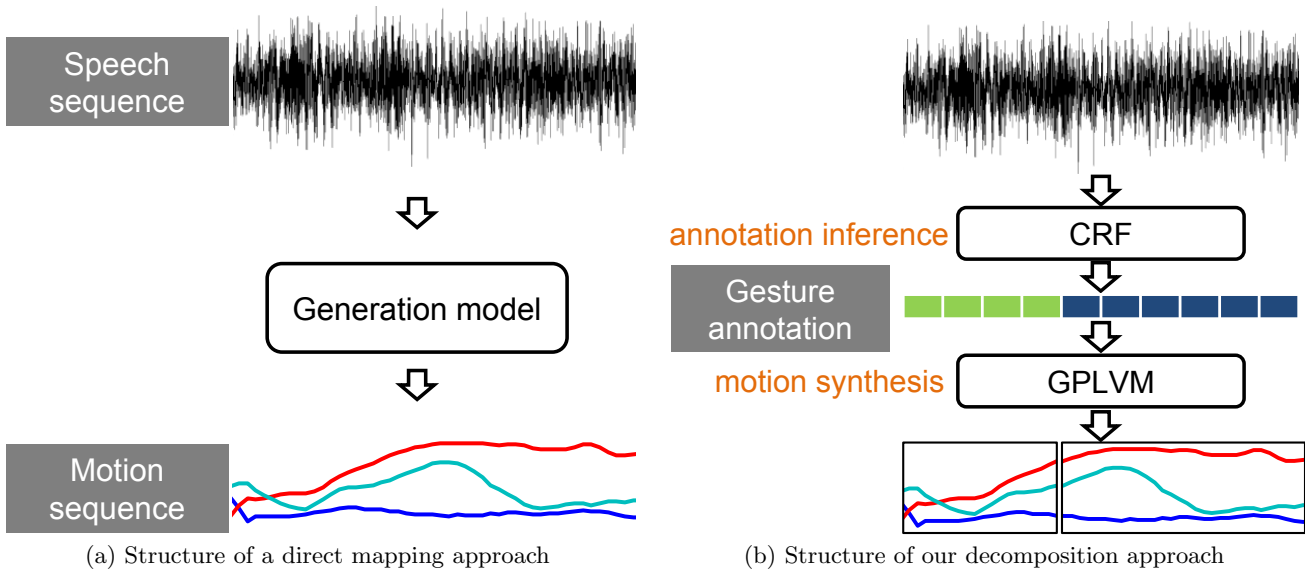
Figure 1: Decomposing the mapping process. (a) The direct mapping approach learns a complex model to generate gesture animations directly from speech sequences. (b) Our approach decomposes the task into speech-annotation inference (with CRFs) and motion synthesis (with GPLVMs). CRFs infer gesture annotations from input speech signals, and GPLVMs synthesize gesture animations with the inferred gesture annotations.
