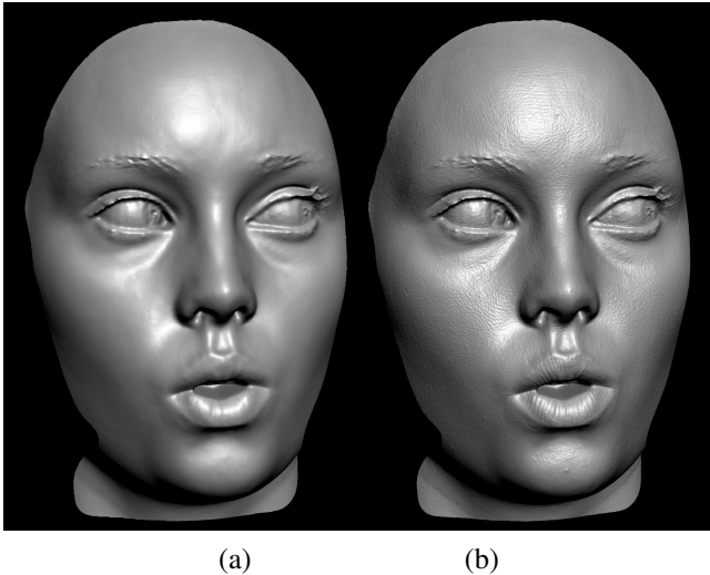
Figure 6: (a) Facial geometry obtained from the diffuse (or subsurface) component of the reflection. (b) Far more detailed facial geometry obtained by embossing the specular normal map onto the diffuse geometry.
