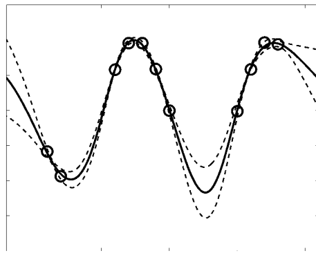
Figure 3. The raw input-output training data, with mean Bayesian MLP predictions (solid curve) and standard error bars (dashed curves). Note how the error bars increase away from the data.
