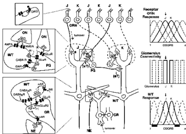
Figure 1. Basic circuit for the olfactory bulb. Abbreviations (left, molecular components): OR, olfactory receptor; ON, olfactory nerve; AMPA, 2-amino-5-phosphonovaleic acid; NMDA, N -methyl-D-aspartate; M/T, mitral/tufted cell; PG, periglomerular cell; GluR, ionotropic glutamate receptor; GABA R, \gamma -aminobutyric acid receptor; DAR, dopamine receptor; NE, norepinephrine; \alpha AR, \alpha -adrenoreceptor; mGluR2, metabotropic glutamate receptor; GR, granule cell. Middle (synaptic circuit): ORN, olfactory receptor neuron; J, K, ORN subsets; e, excitatory; i, inhibitory. Right (structure-function relations) top: overlapping response spectra of ORNs to a range of odors (1 – n); middle: connectivity of subsets to individual glomeruli; bottom: response spectra of M/T cells show less overlap because of lateral inhibition (black bars below abscissa).
