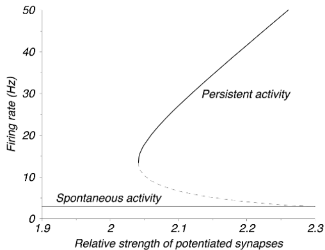
Figure 3. Bifurcation diagram: regions in potentiation-rate plane for stable stationary states of spontaneous activity and selective delay activity. Solid curves denote rates in stable states versus potentiation. Dashed curves indicate a stationary, unstable state, with separating basins of attraction of the two solutions (when both exist). For low potentiation ( <2.05 ), there is only spontaneous activity. For intermediate potentiation ( \geq 2.05 , \leq 2.3 ), there are two stable states. With high potentiation ( \geq 2.3 ), spontaneous activity is unstable (after Brunel, 2000).
