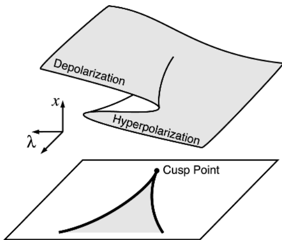
Figure 2. Cusp surface.
