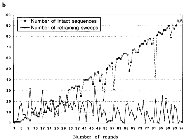
Figure 2. Anticipation model. a , Architecture (adapted from Wang and Yuwono, 1995). Thin solid lines denote modifiable connections, thick dashed lines denote fixed connections, and undirected lines denote bidirectional connections. b , The number of intact sequences and the number of retraining sweeps with respect to the number of training rounds for individual sequences (adapted from Wang and Yuwono, 1996). The 97 sequences denote all the session titles of the 1994 IEEE International Conference on Neural Networks.
