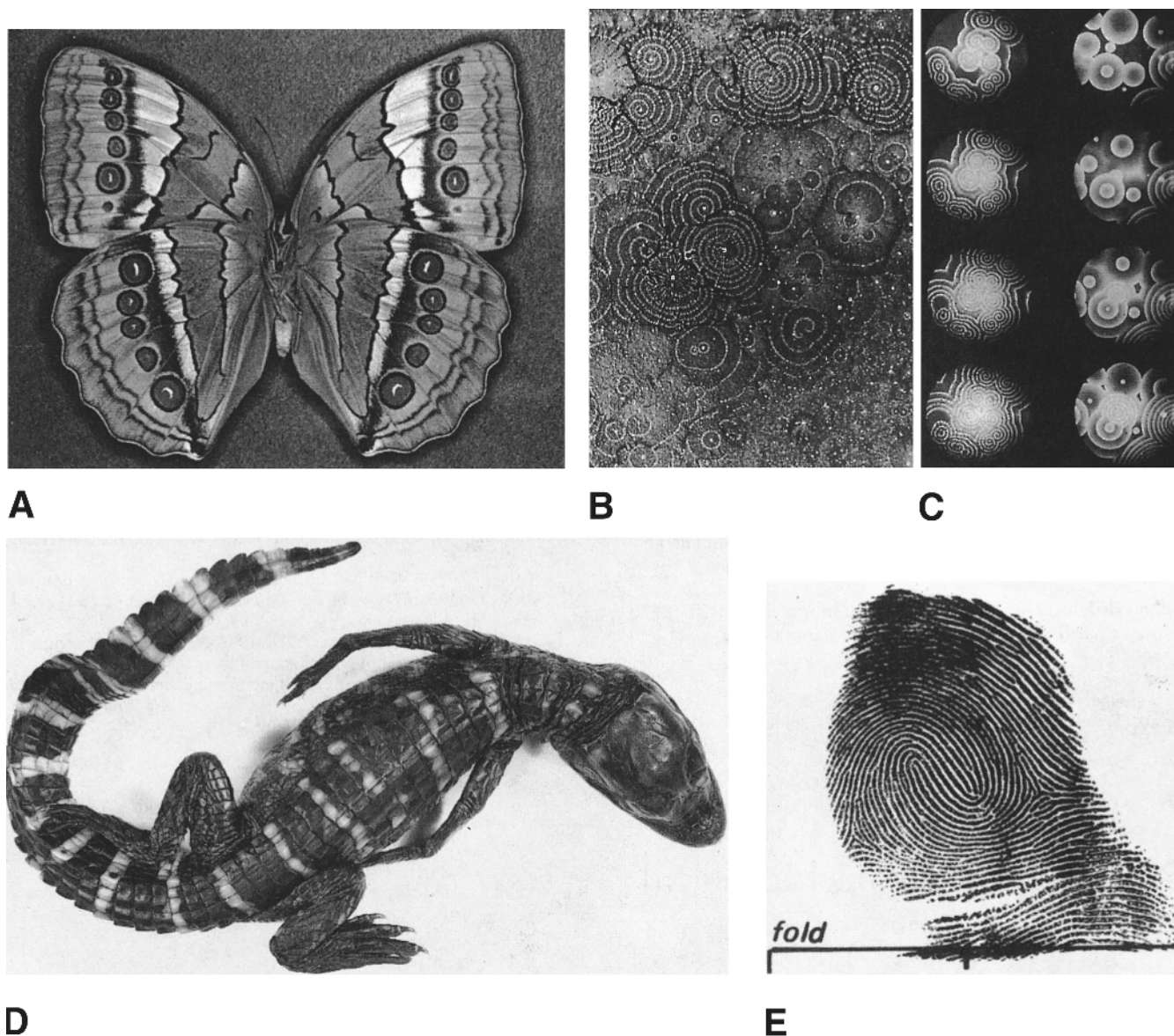
Figure 1. A small sampling of the diverse spatial patterns for which model mechanisms have been proposed. A , The butterfly ( Stichophthalama camadeva ) shown exhibits most of the basic pattern elements observed in butterfly wings. (Photograph courtesy of H. F. Nijhout.) B , Example of moving and stationary bands of amoebae of the slime mold Dictyostelium
