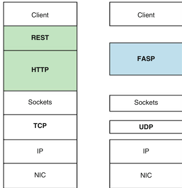
Fig. 14.3 Communication stack
