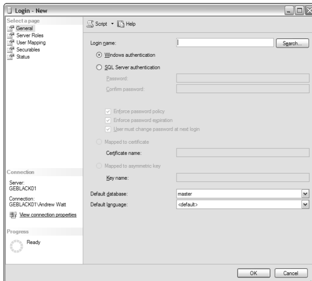
Figure 17-3: The Login – New dialog box.
