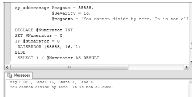
Figure 16-5: Using RAISERROR to produce a custom error message.
