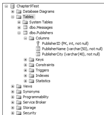
Figure 9-2: The newly created Publishers table.
