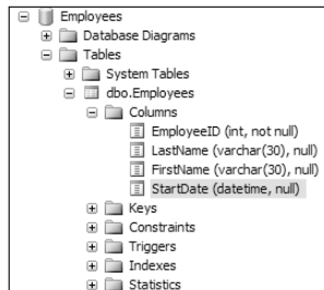
Figure 10-5: The column definitions don't show a DEFAULT constraint.
