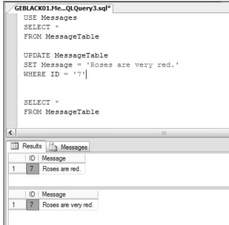
Figure 7-16: Changing the value of a message using an UPDATE statement.
