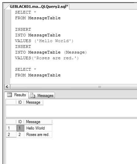
Figure 7-10: Inserting data into a table with an identity column.
