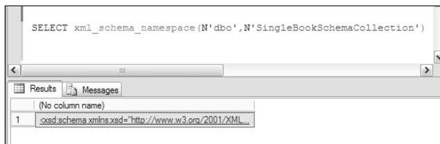
Figure 20-3: Viewing the document(s) in an XML schema collection.
