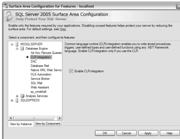
Figure 21-3: The Enable CLR Integration option selected.
