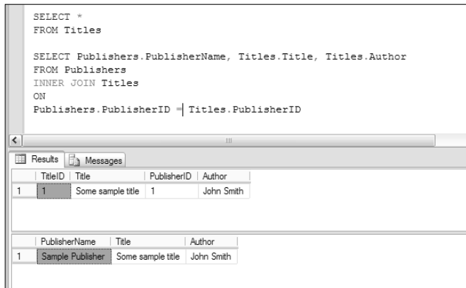
Figure 9-5: Confirming successful creation of the relationship.
