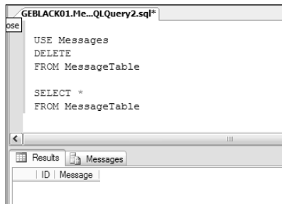
Figure 7-12: Deleting all data from a table.
