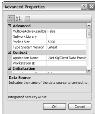
Figure 22-4: The Advanced Properties dialog box.
