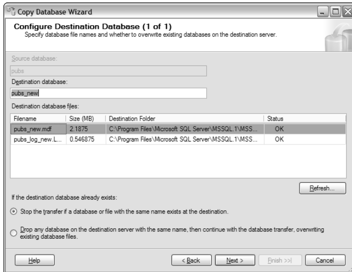
Figure 7-5: The Configure Destination Database screen in the Copy Database Wizard.
