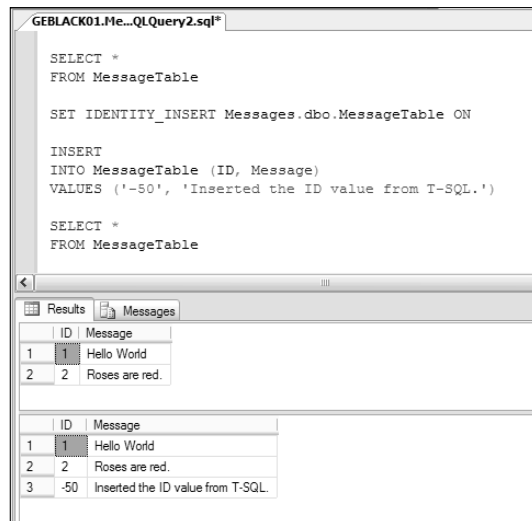
Figure 7-11: Setting IDENTITY_ INSERT to ON to allow insert into an identity column.
