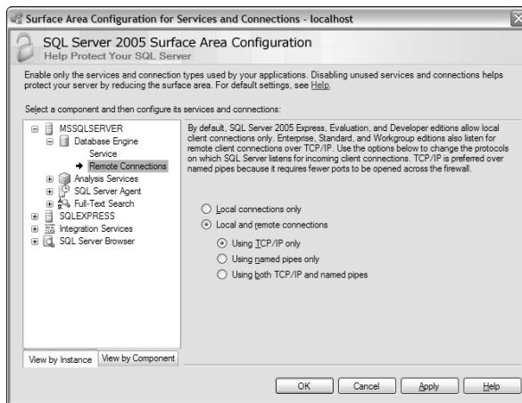
Figure 17-2: The Surface Area Configuration for Services and Connections dialog box, showing where you can specify whether remote connections are allowed.
