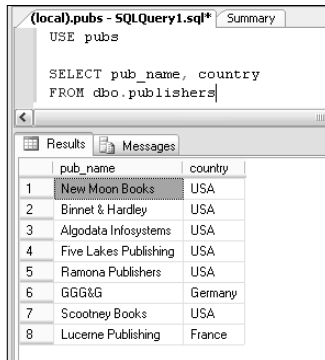
Figure 4-6: Using the SELECT statement to select specified columns from a single table.
