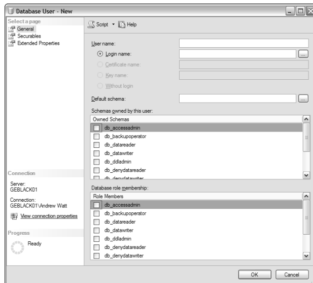
Figure 17-4: The Database User – New dialog box.
