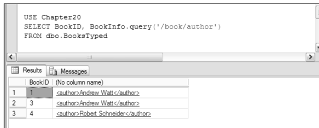
Figure 20-5: Retrieving information in the author element.
