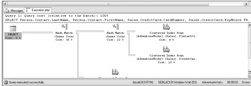
Figure 3-11: An estimated execution plan.
