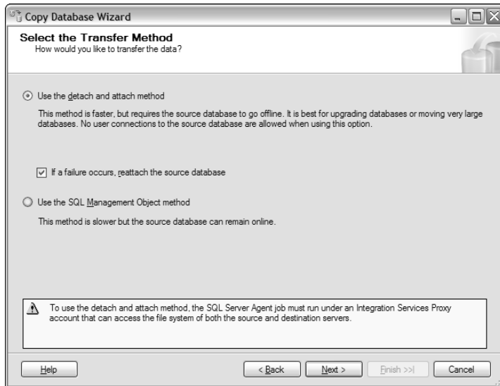
Figure 7-4: The Select the Transfer Method screen in the Copy Database Wizard.
