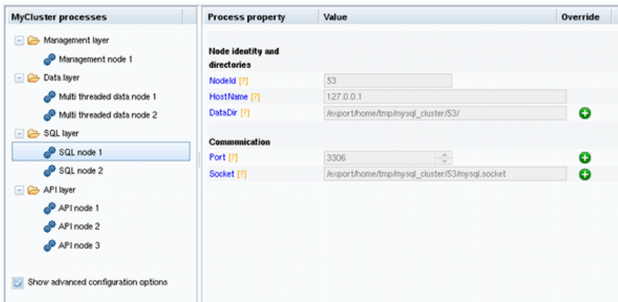
Figure 19.18 Define Attributes Detail With SQL Process Attributes
