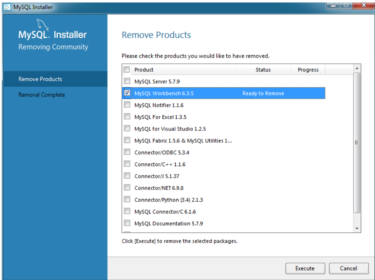
Figure 2.25 MySQL Installer - Removing Products: Select
