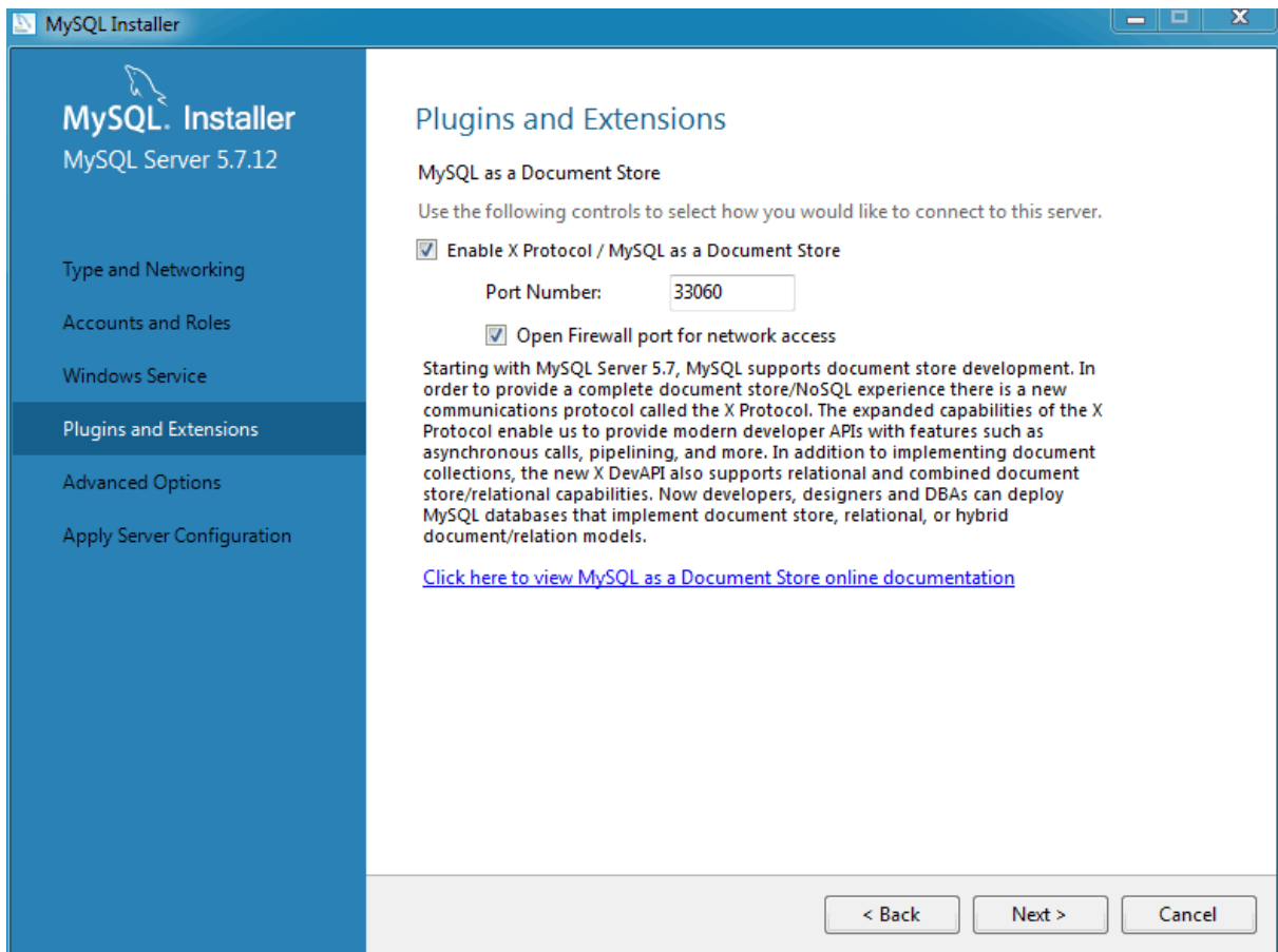
Figure 2.16 MySQL Installer - Plugins and Extensions
