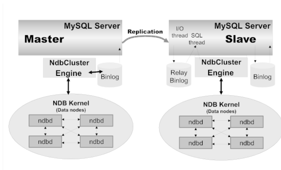
Figure 19.27 MySQL Cluster-to-Cluster Replication Layout
