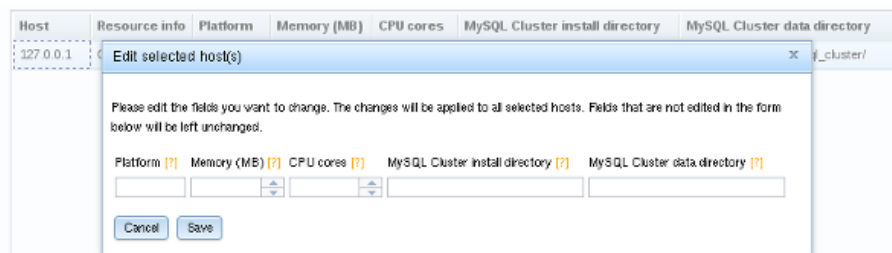
Figure 19.14 MySQL Cluster Auto-Installer Edit Hosts dialog
