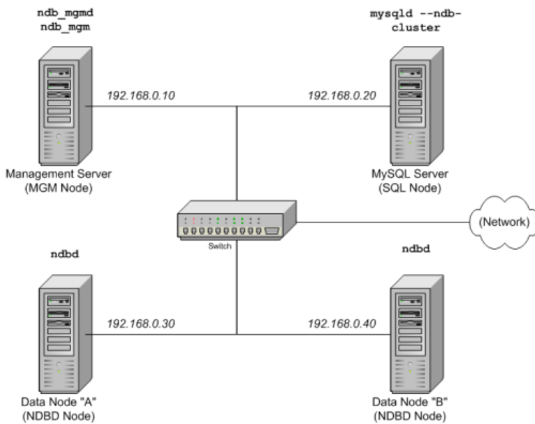
Figure 19.4 MySQL Cluster Multi-Computer Setup
