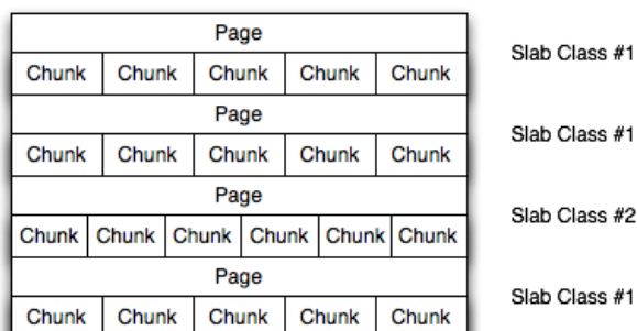
Figure 17.5 Memory Allocation in memcached
