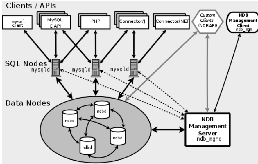
Figure 19.1 MySQL Cluster Components
