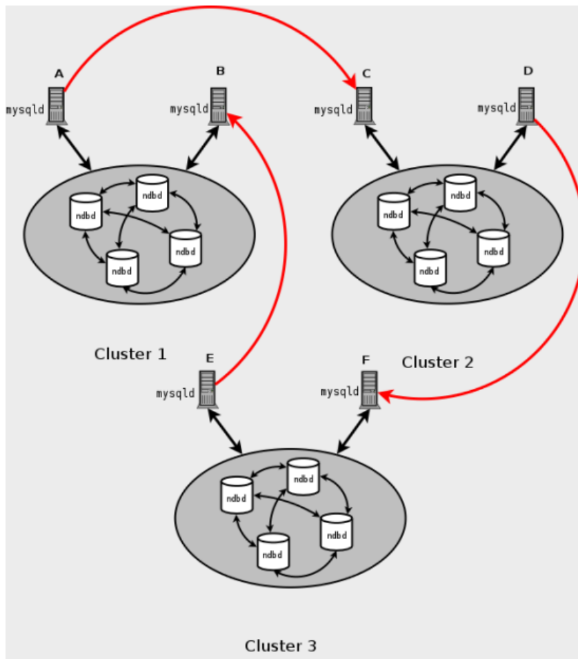
Figure 19.33 MySQL Cluster Circular Replication Where Not All Masters Are Slaves
