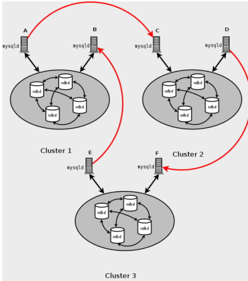
Figure 19.29 MySQL Cluster Circular Replication Where Not All Masters Are Slaves
