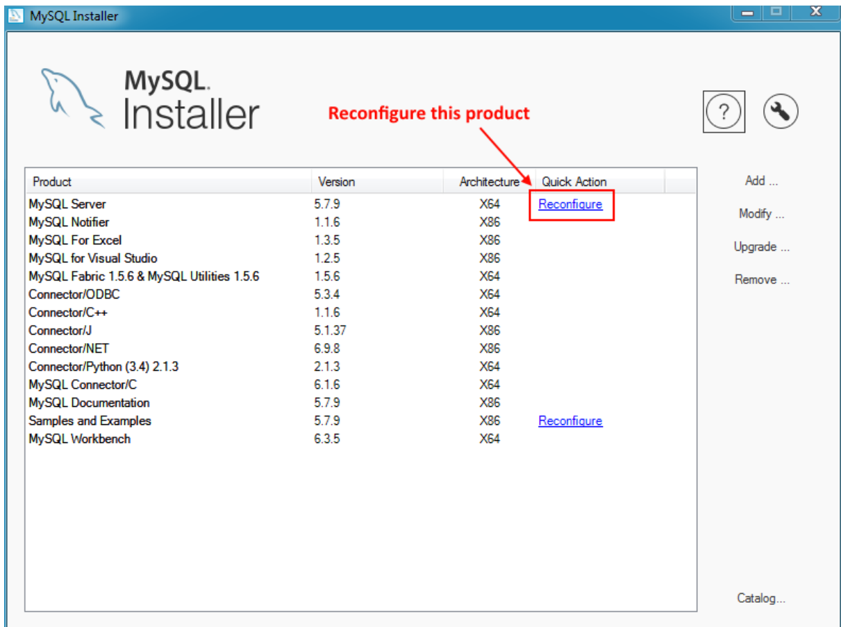
Figure 2.31 MySQL Installer - Reconfigure a MySQL Product
