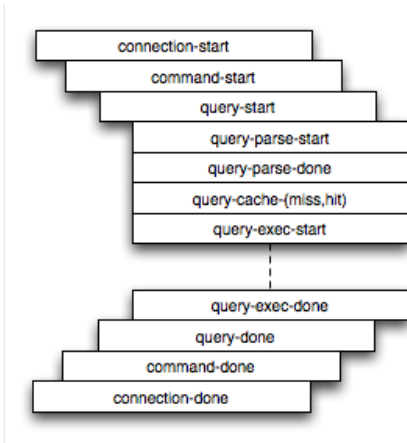
Figure 6.1 The MySQL Architecture Using Pluggable Storage Engines
