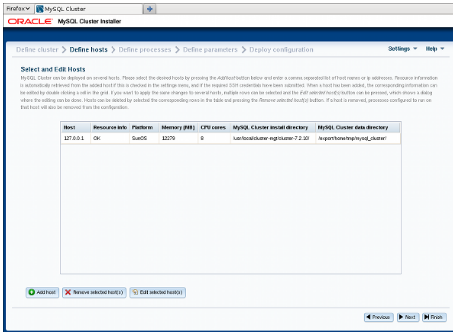
Figure 19.13 MySQL Cluster Define Hosts screen
