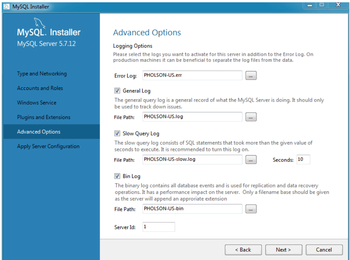
Figure 2.17 MySQL Installer - MySQL Server Configuration: Logging Options
