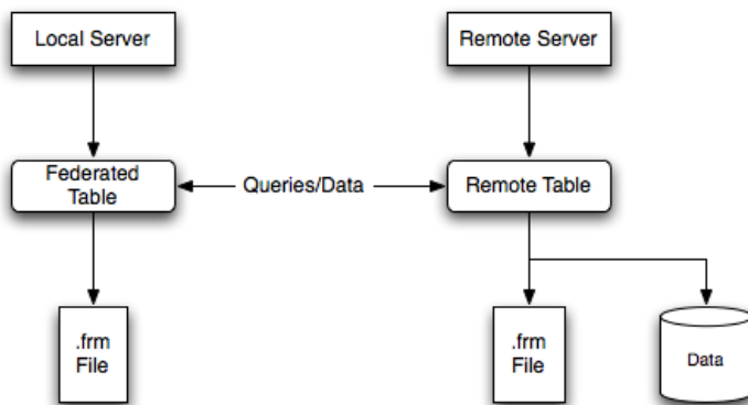
Figure 16.1 FEDERATED Table Structure
