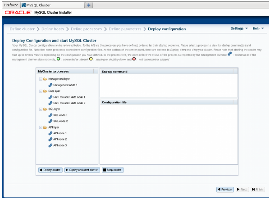
Figure 19.20 MySQL Cluster Auto-Installer Deploy Cluster screen
