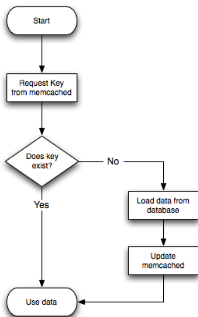
Figure 17.6 Typical memcached Application Flowchart
