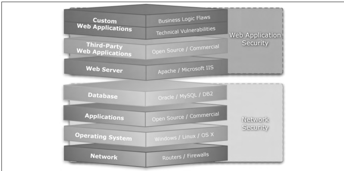
Figure 1.1 Vulnerability Stack
