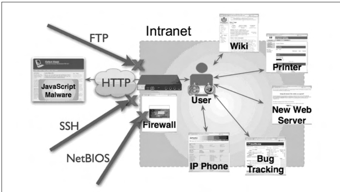
Figure 4.6 Intranet Hacking
