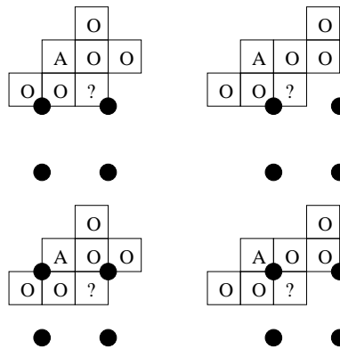
Figure 9: JBIG contexts for progressive transmission. The dark circles are the low resolution pixels, the O s are the high-resolution pixels, the A is a roaming pixel, and the ? is the pixel we want to code/decode. The four context configurations are for the four possible configurations of the high-resolution pixel relative to the low resolution pixel.
