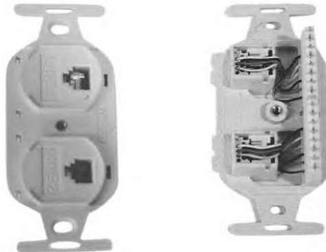
FIXED-DESIGN, DUPLEX, RJ-45 WALL PLATE THAT USES 110 PUNCH-DOWNS
