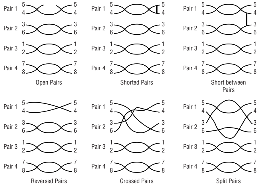
FIGURE 14.2: Common wire-mapping faults
