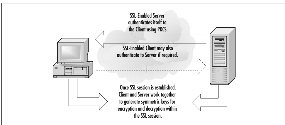
Figure 11.4 SSL Handshake
