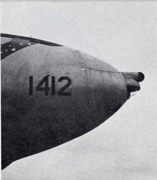
Nose of the B-47E sports the optical dome for the MA-4 horizontal periscopic bombsight. [Robert Loffredo]
