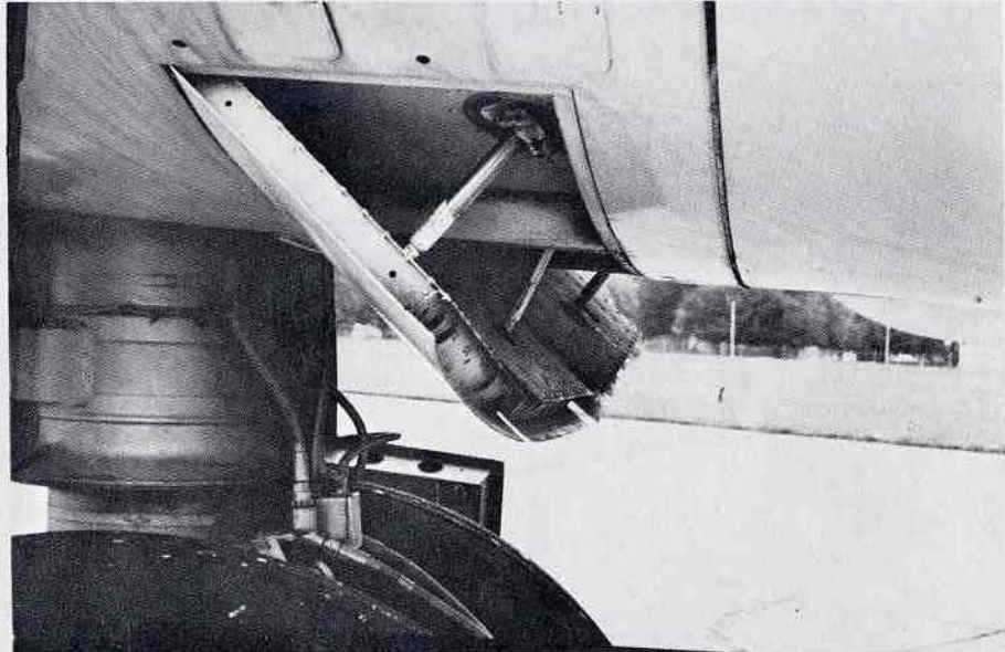
Three spoiler doors in front of the bomb bay were to prevent buffeting in that area. [Robert Loffredo]
