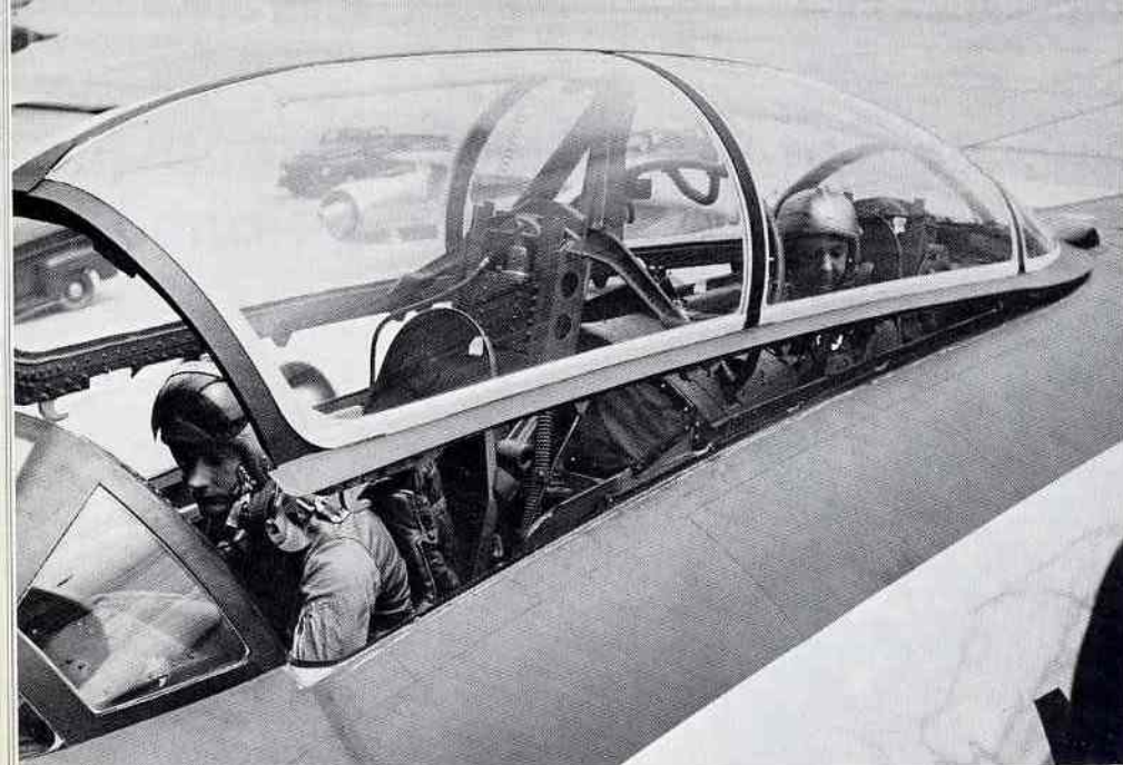
Late model clamshell canopy. Note the visibility problems facing the co-pilot. [Boeing]
