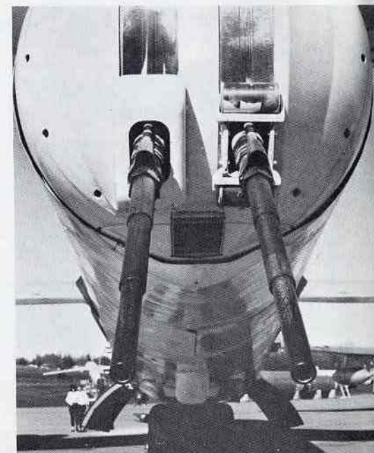
Defensive armament of the B-47 was a pair of tail-mounted M24A-1 20mm cannons. Note that the roller assembly cover is missing on gun at right. [Robert Loffredo]
