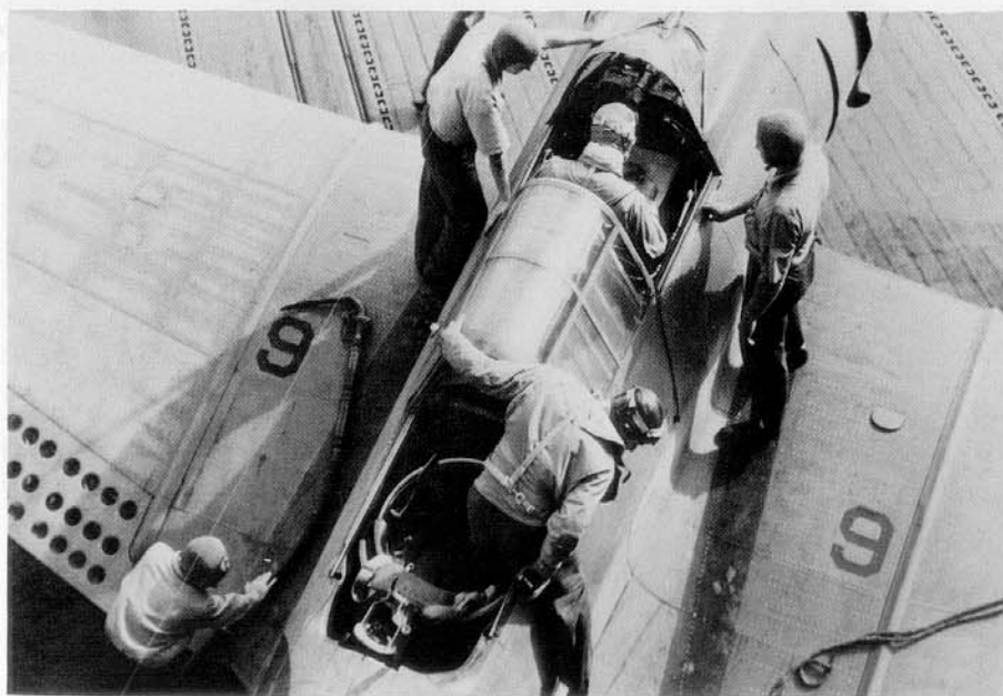
The gunner climbs out of this early SBD-3 while the pilot makes final notes on his chart before getting out. The deck crew is already clambering onto the wings to refuel the Dauntless. Note the double doors covering the trough for the gunner's single .30 caliber machine gun, Enterprise, 31 May 1942. (USN/NARS)
