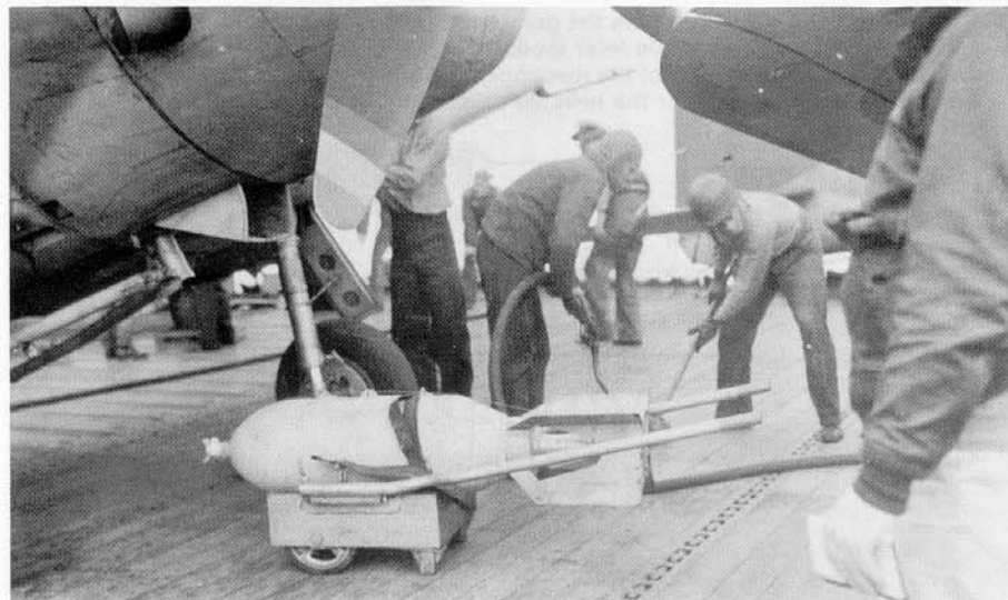
A 500 lb GP bomb sits on its trolley, waiting to be loaded on the bomb crutch of an SBD-3, Ranger, November 1942. (USN/NARS)
