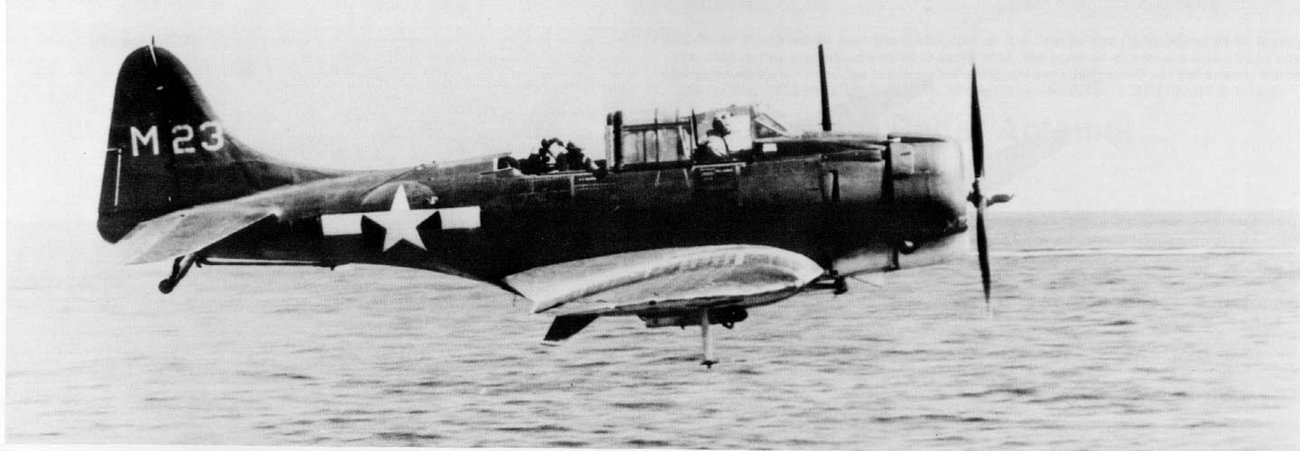
The letter and number code on the tail of this SBD-5, seen just after making a message drop on the Lexington, probably indicates the machine belongs to a land-based Marine unit, 16 April 1944. The tailwheel fairing was removed on many land-based Dauntlesses and even on some carrier-based aircraft. (USN/NARS)
