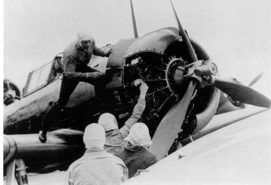
Mechanics work on the Wright R-1820-52 of this SBD-3 on the deck of the Ranger in November of 1942. The composite spinners were removed on all of VS-41's Dauntlesses, exposing the the hub and operating mechanism of the adjustable pitch prop. (USN/NARS)
