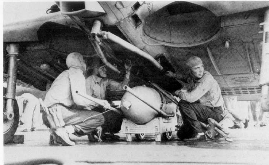
Deck crewmen on Enterprise (above) and Ranger (below) rig 1000 lb GP bombs on SBD-3s. Once the bomb is positioned, the armorers set the fuse and the bomb is hoisted with a handwinch (USN/NHC and USN/NARS)
