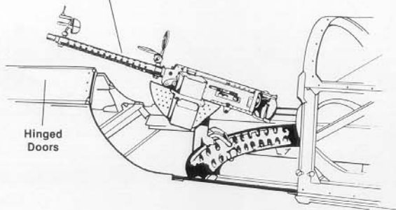
Single .30 Calibre SBD-2
