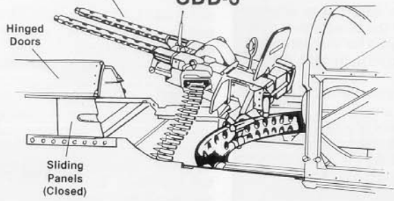
Twin .30 Calibre Field-modified SBD-3
