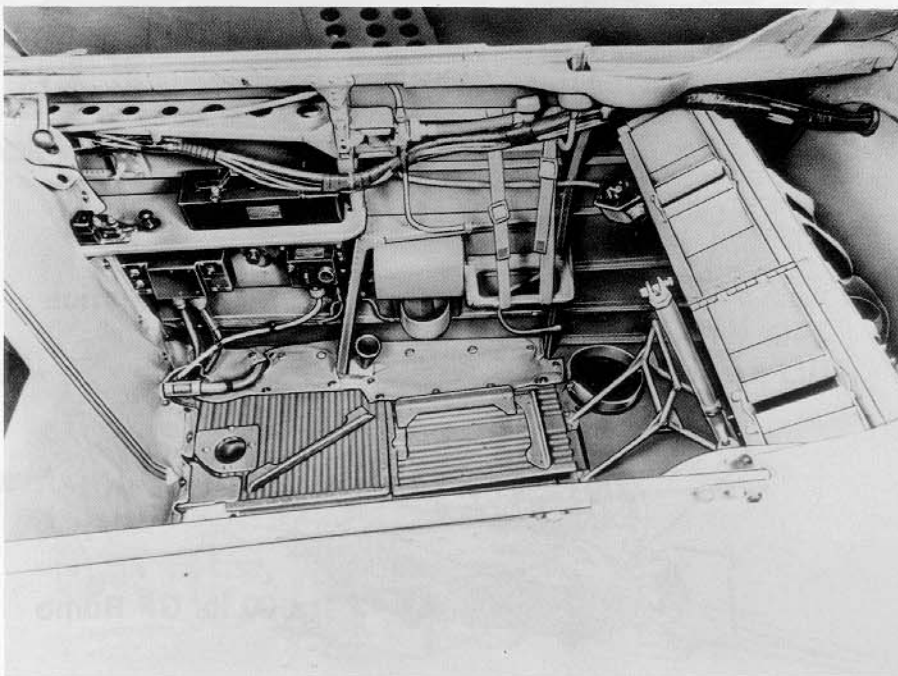
The rear cockpit of an SBD-3, minus the gun turret. (Above) Racks at the front of the rear cockpit held radio equipment. On later models the radar set was installed here as well. (Above Left) The starboard side of the rear cockpit. (Left) The port side of the rear cockpit. To the rear are ammo boxes for the twin .30 caliber gun mount. (USN/NARS)
