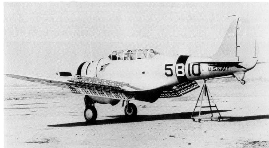
5-B-10 markings on the side of BT-1 (BuNo 0606) indicated the 10th aircraft of Yorktown's VB-5. The cowling, fuselage band and chevron were Black. The tail is Red. The perforated flap/dive brakes were carried over to the SBD. (NASM)
