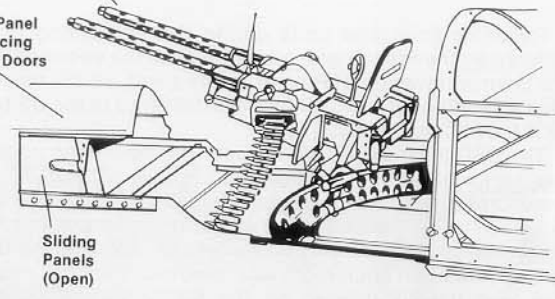
Twin .30 Calibre Late SBD-3
