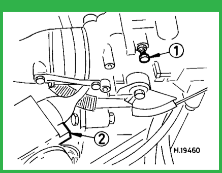
LH2.4-Jetronic
