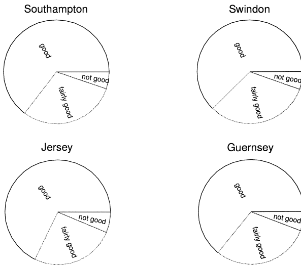
Fig. 103 Examples of pie charts for subjective assessment of health in four regions.
