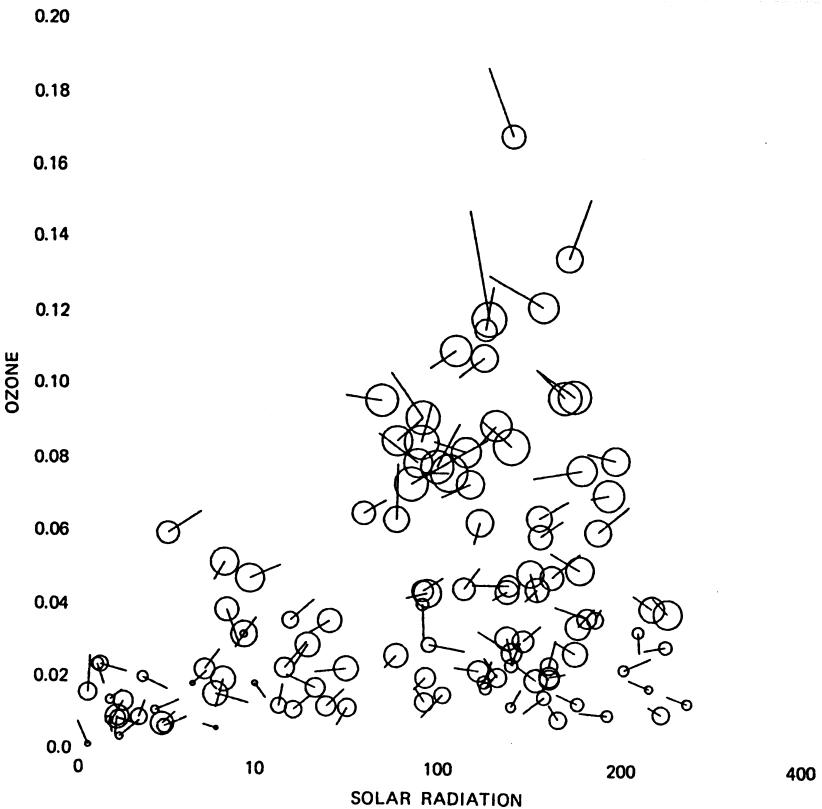
Fig. 146 Weathervane plot.
