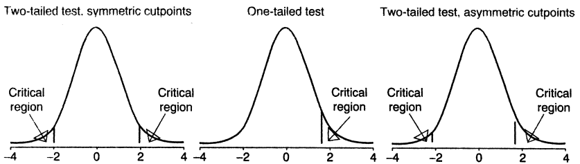
Fig. 48 Critical region.
