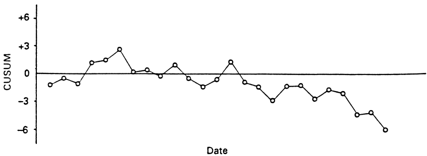
Fig. 49 Cusum chart.
