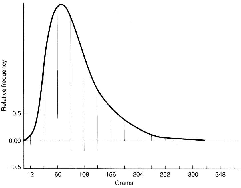
Fig. 71 An example of a hanging rootogram.
