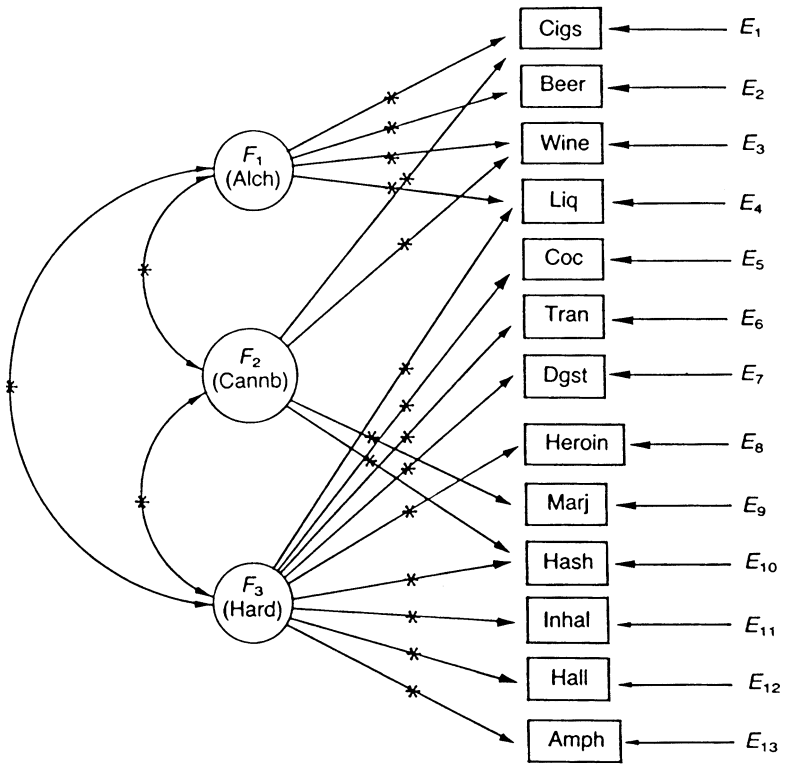
Fig. 102 A path diagram for a correlated three factor model.
