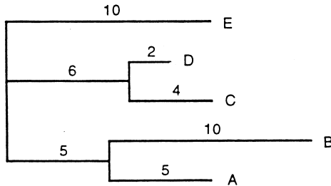
Fig. 2 An example of an additive tree. (Reproduced by permission of Sage Publications from Tree Models of Similarity and Association , 1996, J.E. Corter.)
