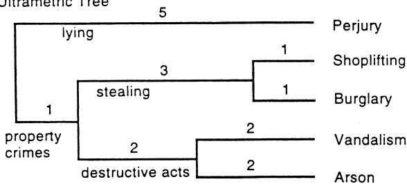
Fig. 138 An example of an ultrametric tree. (Taken from Tree Models of Similarity and Association , 1996, J.E. Corter, by permission of the publishers, Sage.)
