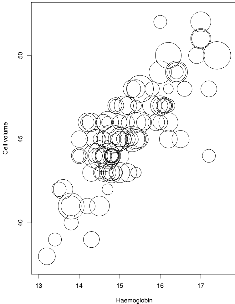
Fig. 24 Bubble plot of haemoglobin concentrates versus cell volume with radii of circles proportional to white blood count.
