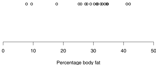
Fig. 117 A rugplot of percentage body fat in a number of individuals.
