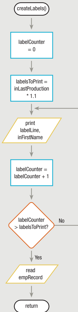
FIGURE 6-14: USING A do until LOOP TO PRINT ONE IDENTIFICATION LABEL, THEN PRINT ENOUGH TO COVER PRODUCTION REQUIREMENTS
