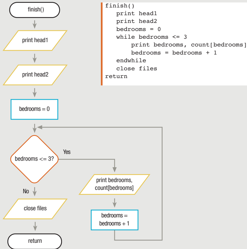
FIGURE 8-12: MODIFIED finish() MODULE THAT USES AN ARRAY
