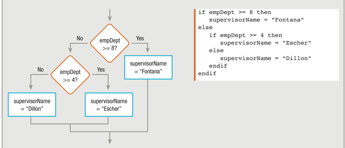
FIGURE 5-32: USING LOW-END VALUES OF RANGES TO DETERMINE EMPLOYEE’S SUPERVISOR
