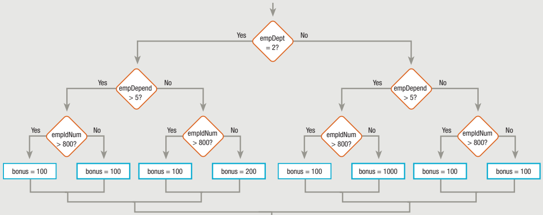
FIGURE C-9: FLOWCHART AND PSEUDOCODE FOR BONUS DECISION, PART 4
