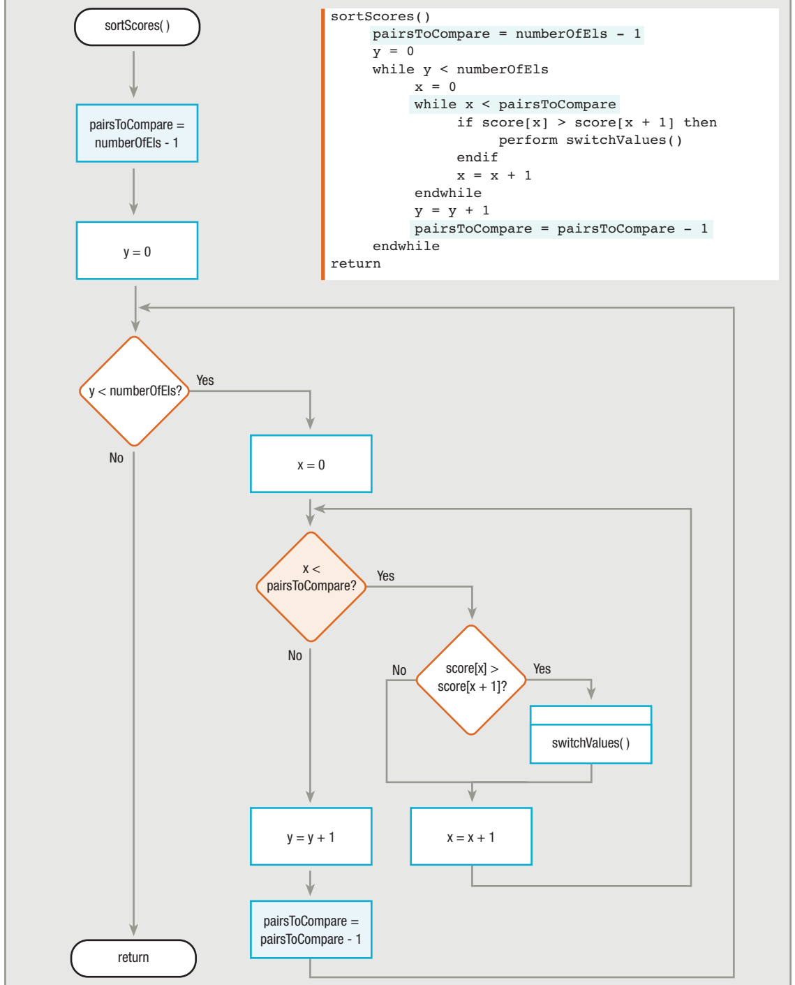
FIGURE 9-12: FLOWCHART AND PSEUDOCODE FOR sortScores() MODULE USING pairsToCompare VARIABLE
