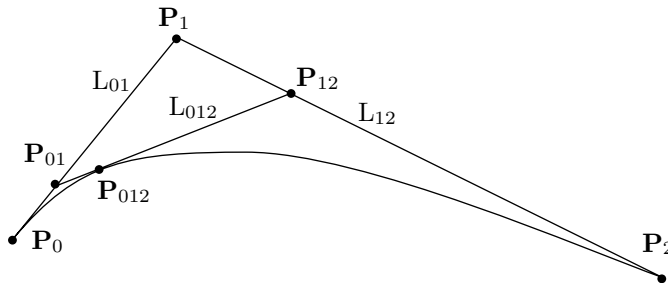
Figure 6.7: Repeated Linear Interpolation.
