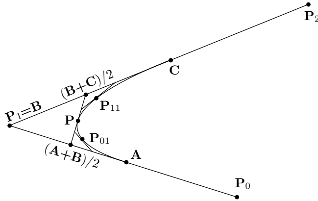
Figure 8.6: Points on the Chaikin Curve.
