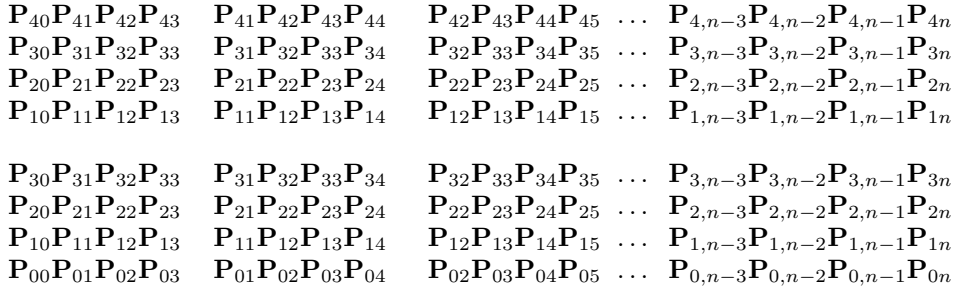
Figure 5.9: Points for a Catmull–Rom Surface Patch.
