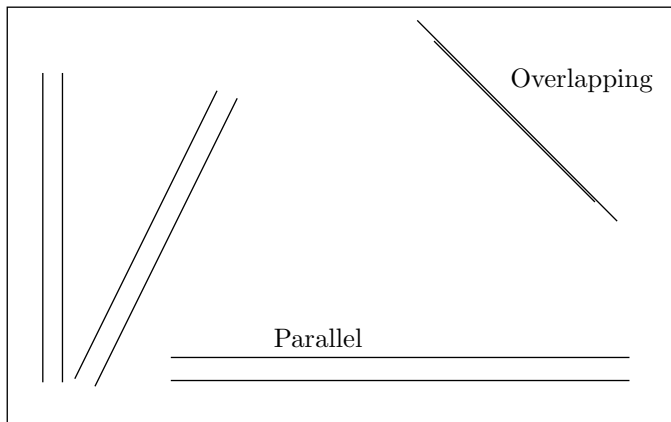
Figure 2.2: Parallel and Overlapped Lines.
