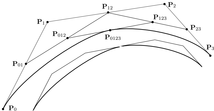
Figure 6.8: Scaffolding for k = 3 .
