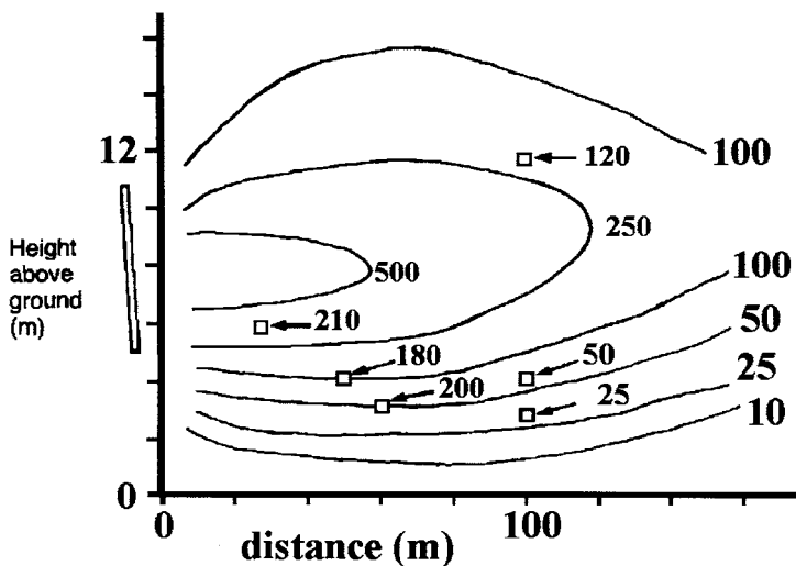
Figure 10.12 Use of elevated platform for special measurements
