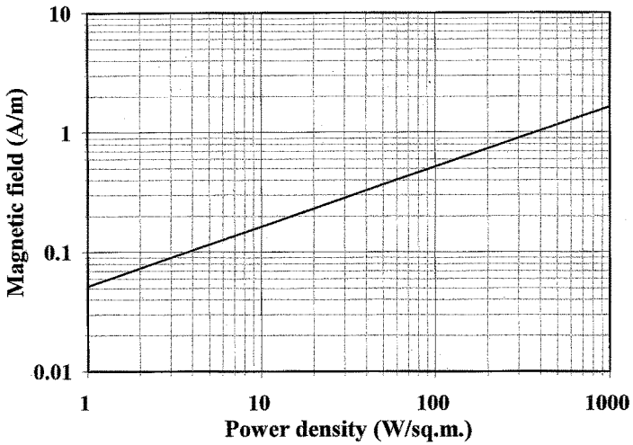
Figure A1.2 Power density values ( Wm^{-2} ) versus magnetic field plane wave values ( Am^{-1} )
