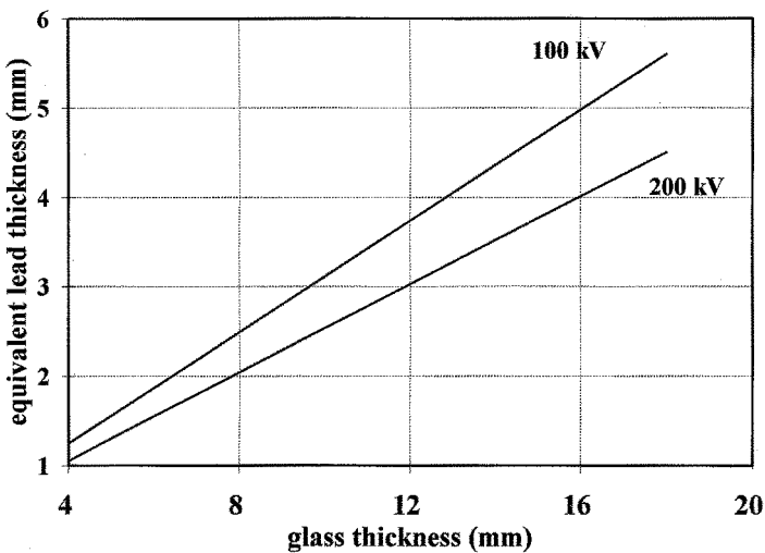
Figure 11.7 Curves for lead-glass shielding material (Courtesy of Pilkington Special Glass, Wales UK)
