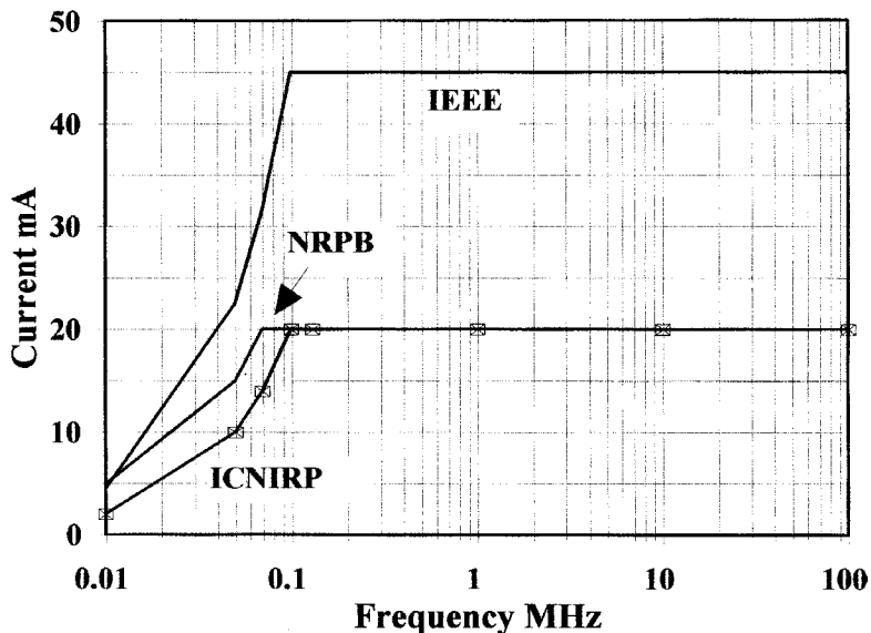
Figure 4.12 Contact current (public)
