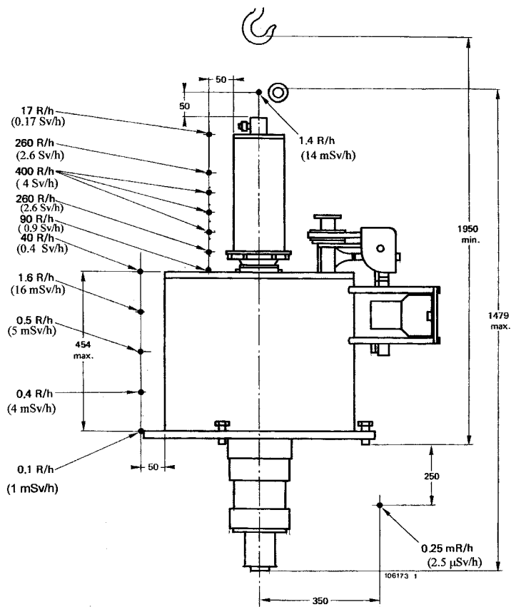
Figure 8.4 Klystron X-ray test results (Courtesy Thomson Tubes Electroniques)
