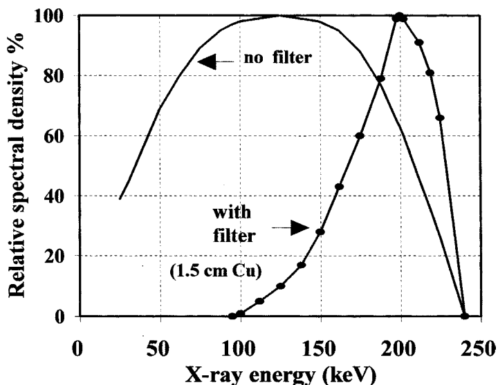
Figure 8.5 Klystron energy distribution (Courtesy Thomson Tubes Electroniques)
