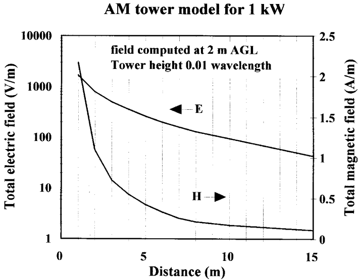
Figure 5.20 AM broadcast model for 1 kW, 0.01λ tower height
