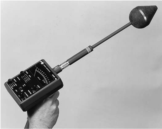
Figure 7.12 GMC Raham 495 meter unit and probe (Courtesy General Microwave Corp.)
