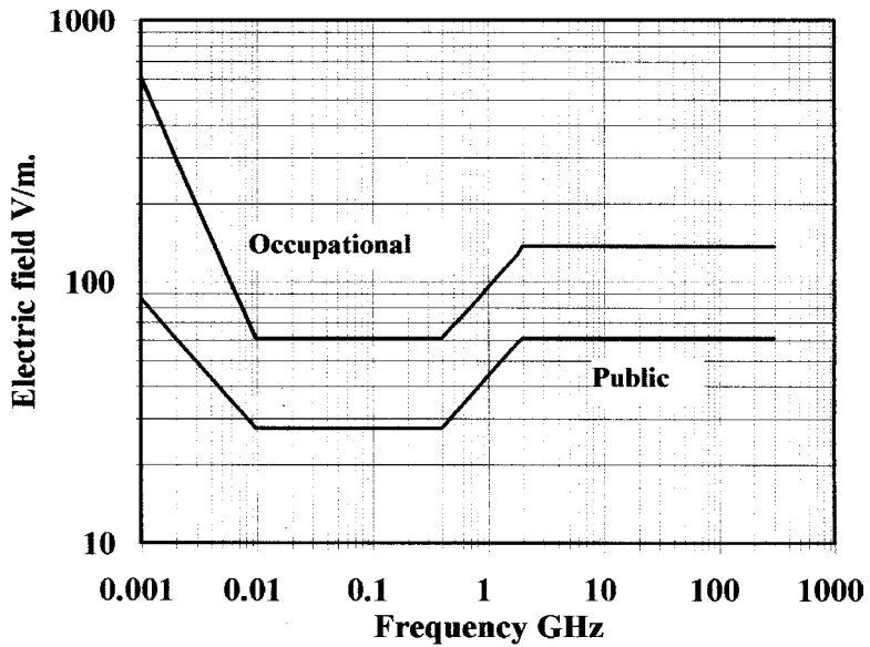
Figure 4.8 ICNIRP98 electric field
