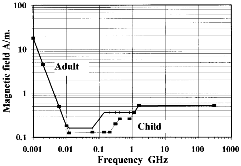
Figure 4.7 NRPB93 magnetic field
