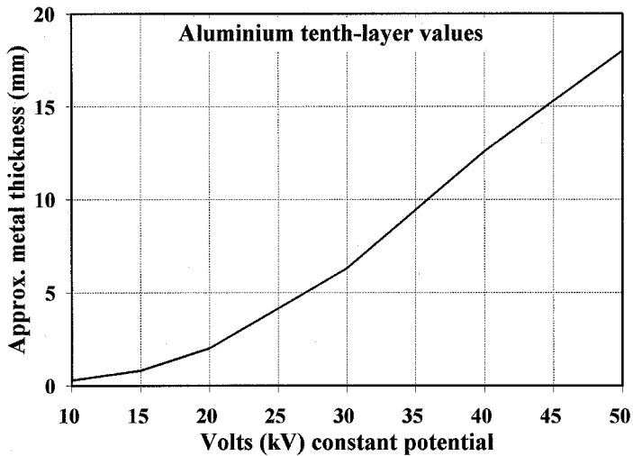
Figure 11.6 Tenth value layer thicknesses for aluminium shielding (Courtesy of BSI London)
