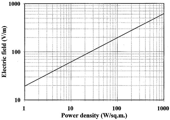
Figure A1.1 Power density values ( Wm^{-2} ) versus electric field plane wave values ( Vm^{-1} )
