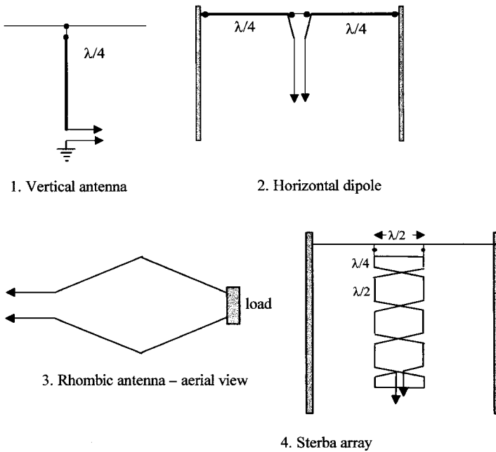
Figure 2.5 Simple HF antennas
