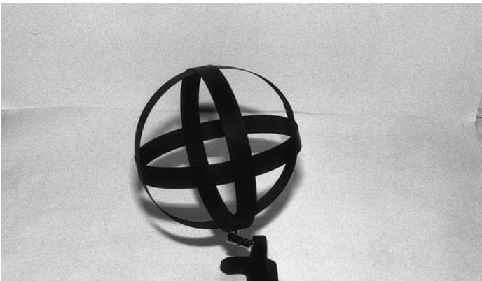
Figure 7.4 Sensor isotropic antennas – magnetic field
