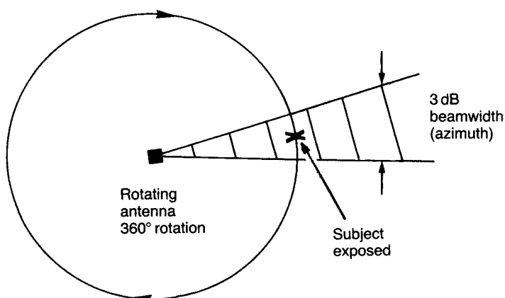
Figure 5.13 Rotating beam power density time-averaging for a subject in the intermediate/far field
