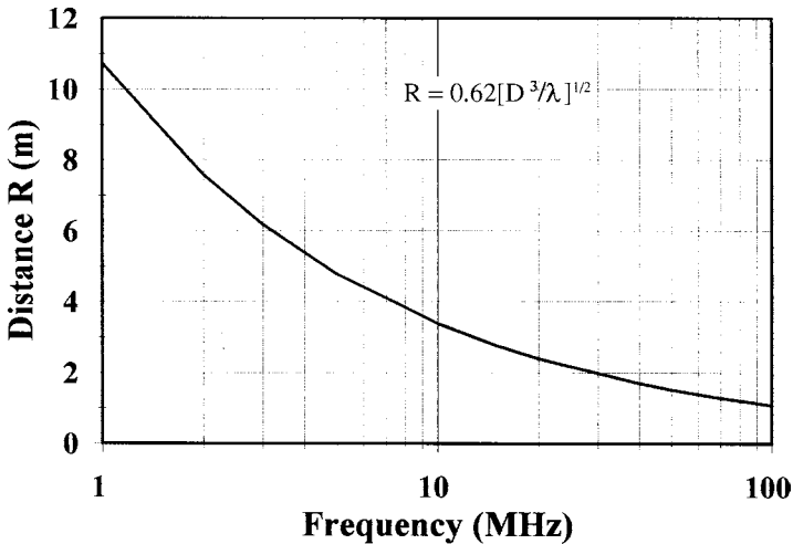
Figure 5.16 Plot of 0.62[D^3/\lambda]^{1/2} versus distance for 1 to 100 MHz
