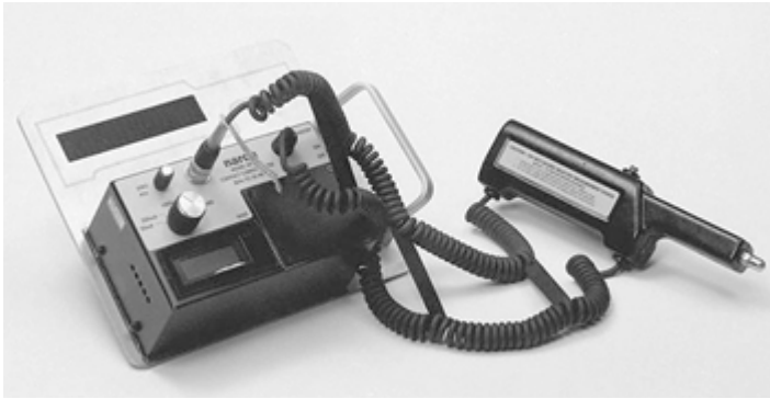
Figure 7.24 Narda model 8870 contact current meter (Courtesy Narda Safety Test Systems)
