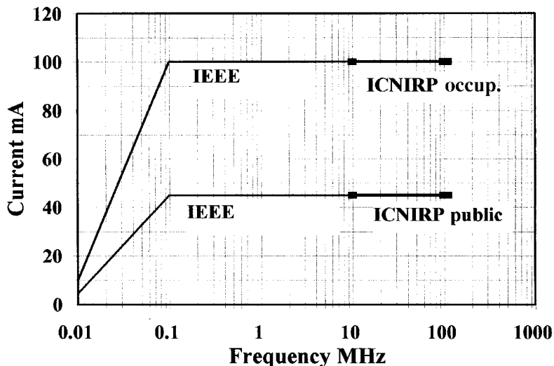
Figure 4.10 Induced body/limb currents
