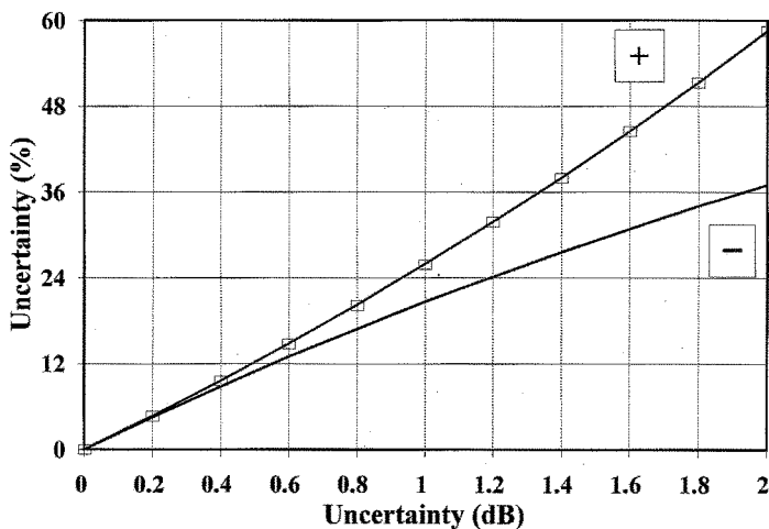
Figure 12.5 Uncertainties of measurement expressed in decibels and percentage for power density
