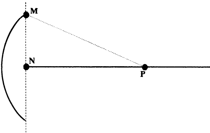
Figure 5.1 Rayleigh distance illustration
