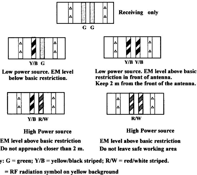
Figure 6.24 Experimental safety markings for rooftop and similar installations
