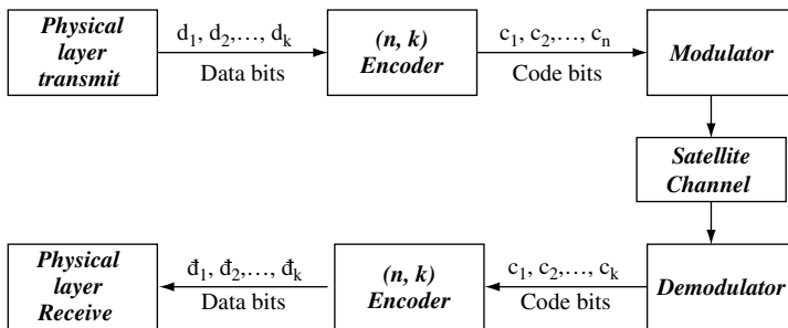
Figure 2.18 Forward error correction (FEC) coding
