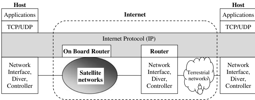
Figure 6.1 Relationship between IP and different network technologies
