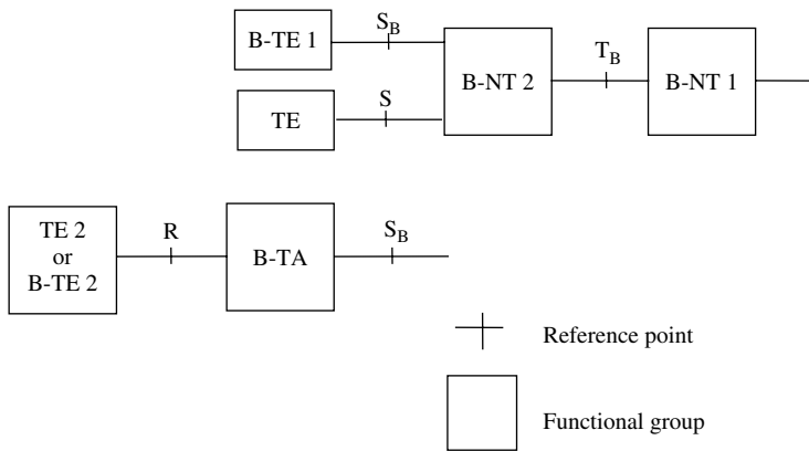
Figure 3.20 B-ISDN reference configuration
