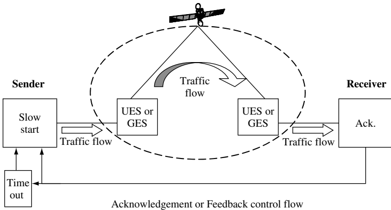
Figure 7.5 Traffic and control flows
