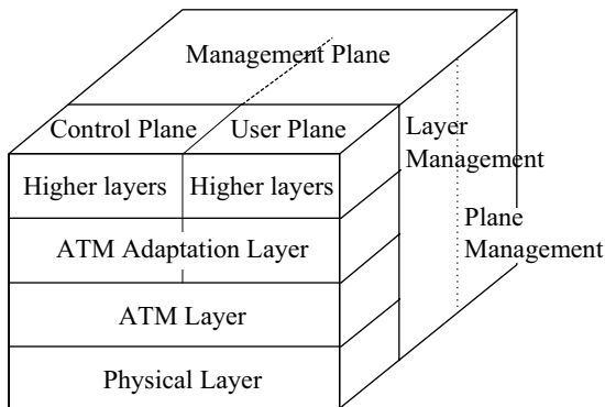
Figure 1.15 B-ISDN ATM reference model
