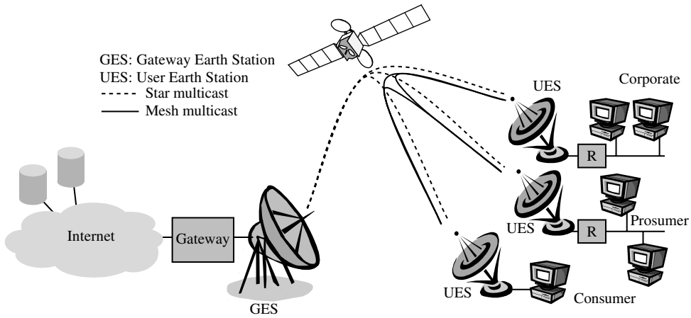
Figure 6.13 The GEOCAST system as an example of star and mesh topologies
