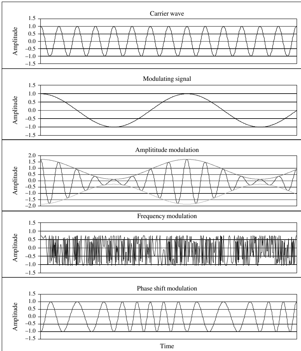
Figure 2.13 Carrier waves, modulating signals and modulated signals
