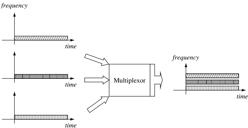
Figure 1.5 Concept of multiplexing in the frequency domain
