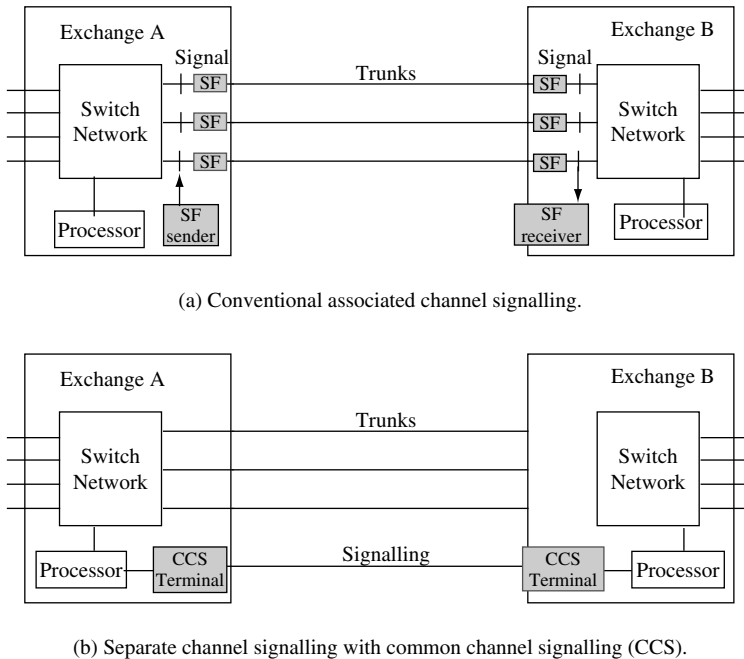
Figure 4.6 Associated and separate signalling
