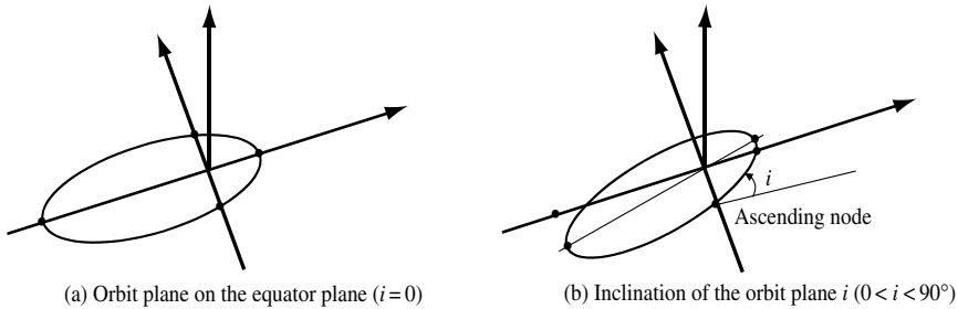
Figure 2.3 Inclination of orbit i
