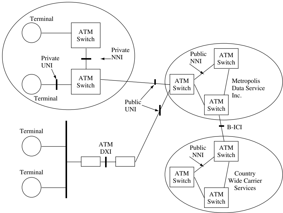
Figure 3.21 ATM interfaces network nodes interconnections
