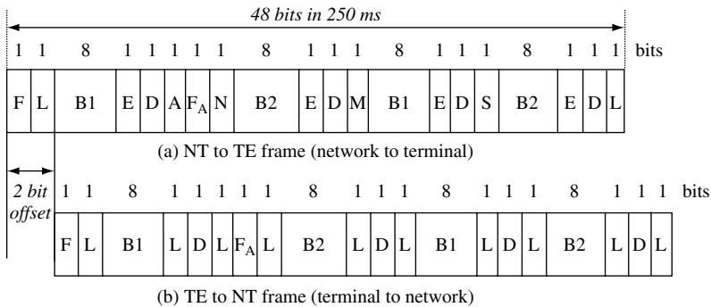
F = Framing bit, F A = Auxiliary framing bit, L = DC balancing, E = Echo of previous D bits, D = D channel, A = Activation bit, M = Multiframing bit, S = Spare bits B1 = B1 channel bits, B2 = B2 channel bits, N = a binary value N = F A (NT to TE)
