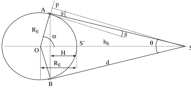
Figure 2.11 Relation between elevation angle and altitude
