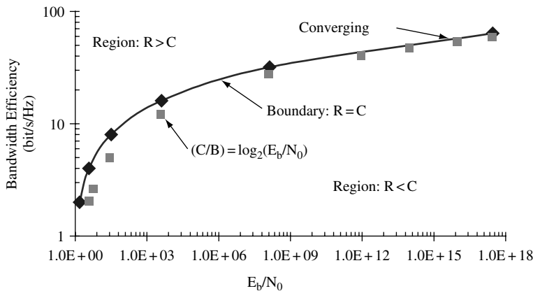
Figure 1.21 The Shannon bandwidth efficiency for large E_b/N_0
