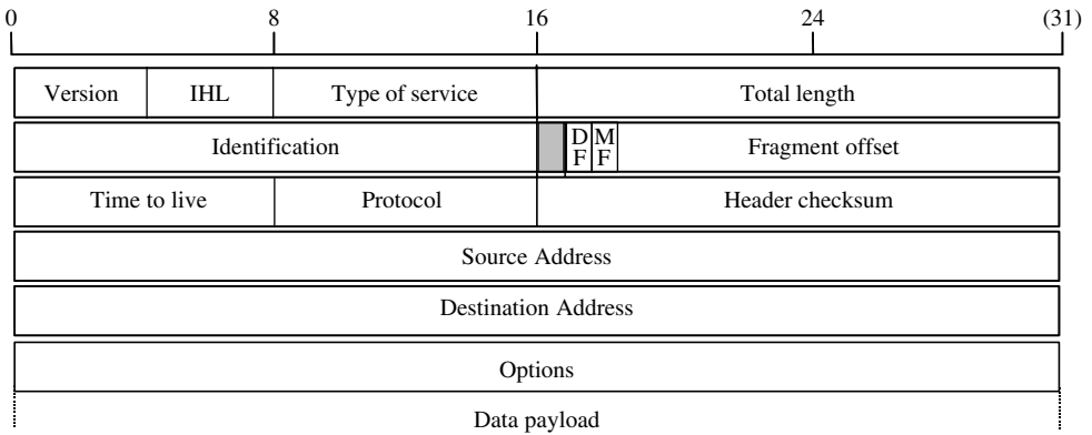
Figure 3.29 IP packet header format
