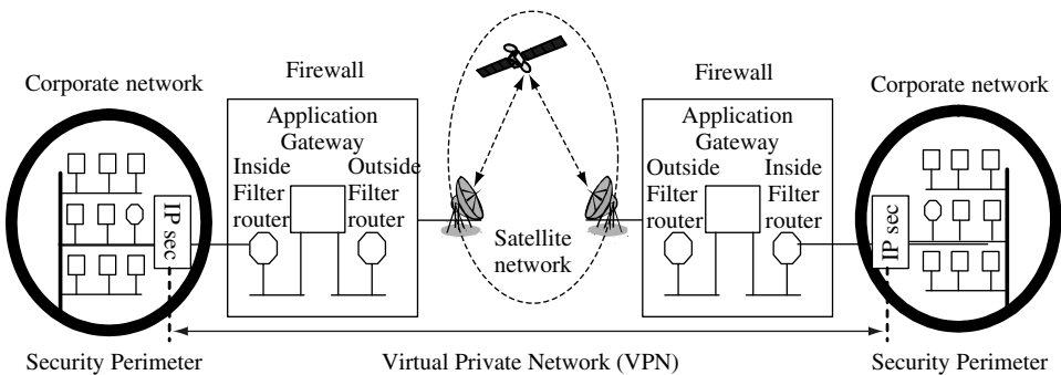
Figure 6.21 Firewall consisting of two routers and one gateway
