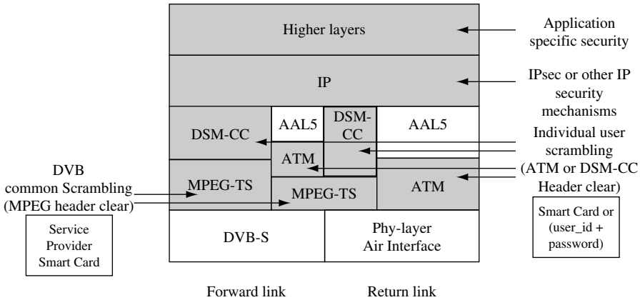
Figure 6.29 IP stack and security in DVB-S and DVB-RCS (© ETSI 2003. © EBU 2003. Further use, modification, redistribution is strictly prohibited. ETSI standards are available from http://www.etsi.org/services_products/freestandard/home.htm and http://pda.etsi.org/pda/ .)
