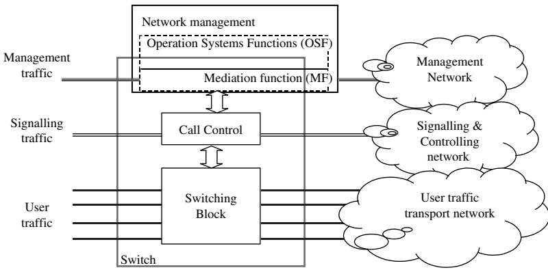
Figure 4.2 Relationships between user, signalling and management functions
