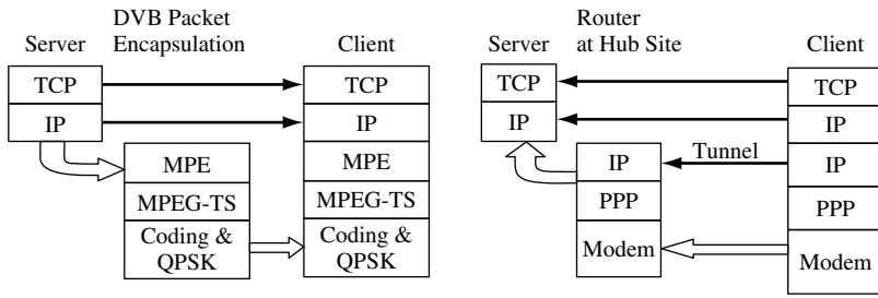
Figure 6.31 DVB-S and DVB-RCS protocol stack
