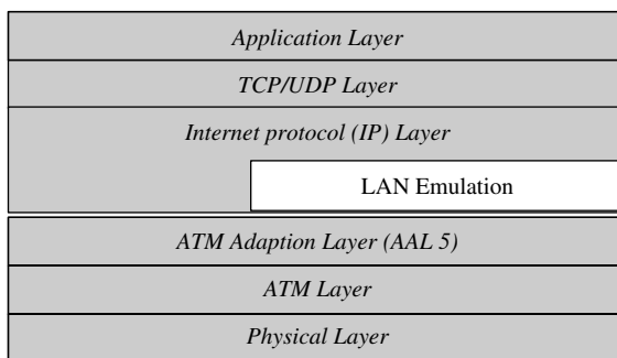
Figure 3.35 Protocol stacks for LAN emulation and classical IP over ATM
