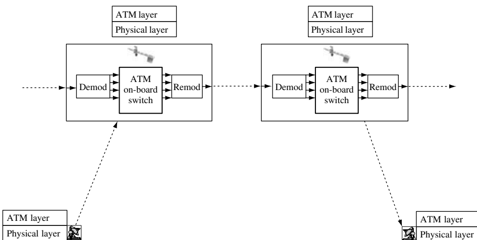
Figure 5.6 Satellite with ATM on-board switch
