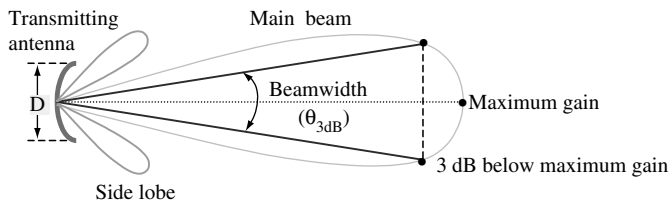
Figure 2.10 Antenna radiation pattern
