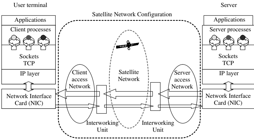
Figure 7.2 Example of satellite network configurations
