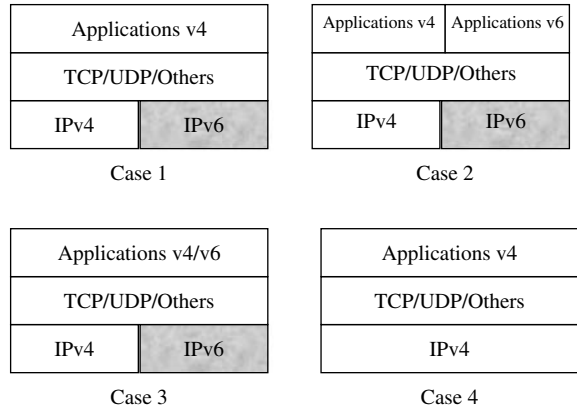
Figure 8.20 IPv6 application transitions
