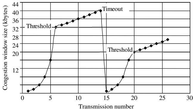
Figure 3.33 Congestion control and avoidance
