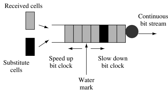
Figure 3.12 Illustration of adaptive clock method
