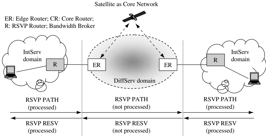
Figure 6.39 Architectural for Intserv networks via satellite DiffServ network
