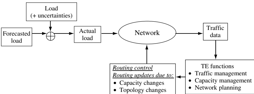
Figure 8.7 The traffic engineering process model
