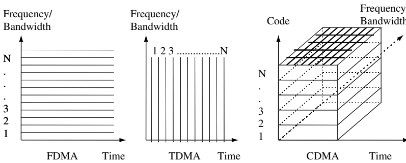
Figure 2.22 Multiple access techniques: FDMA, TDMA and CDMA
