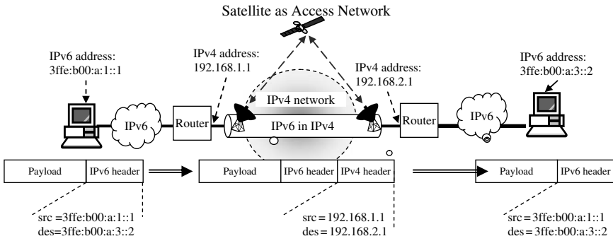
Figure 8.17 Router to router tunnelling through satellite core network
