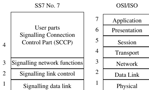
Figure 4.7 Relationship between the SS No.7 and OSI/ISO reference model
