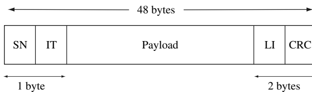
Figure 3.13 AAL 2 packet format for Class B
