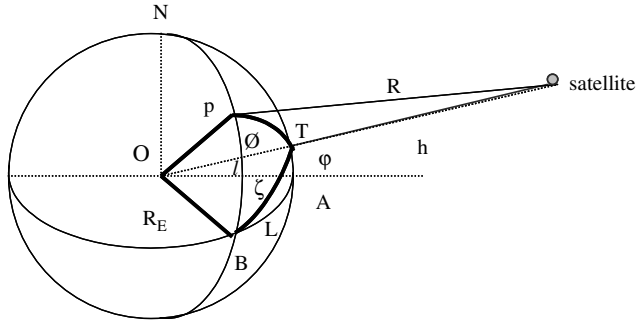
Figure 2.12 Distance between earth station and satellite
