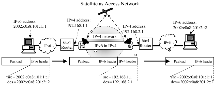
Figure 8.19 The 6to4 translation via satellite core network
