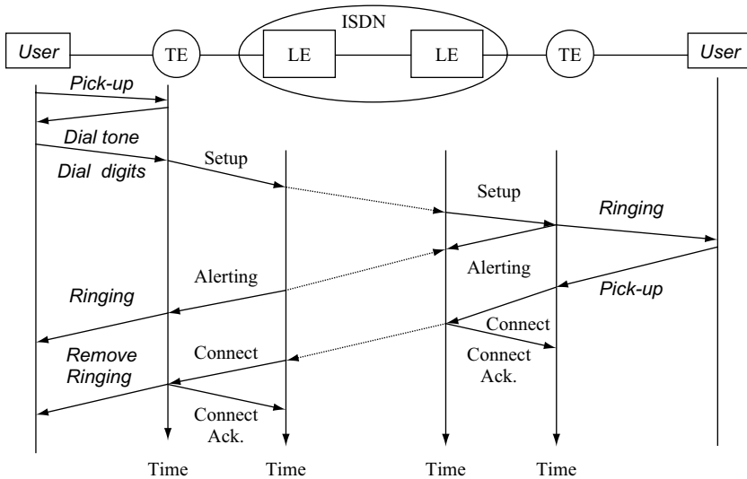
Figure 4.21 Illustration of the ISDN layer 3 signalling
