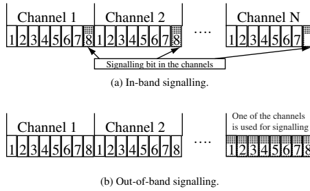
Figure 4.5 Digital network in-band signalling and out-of-band signalling
