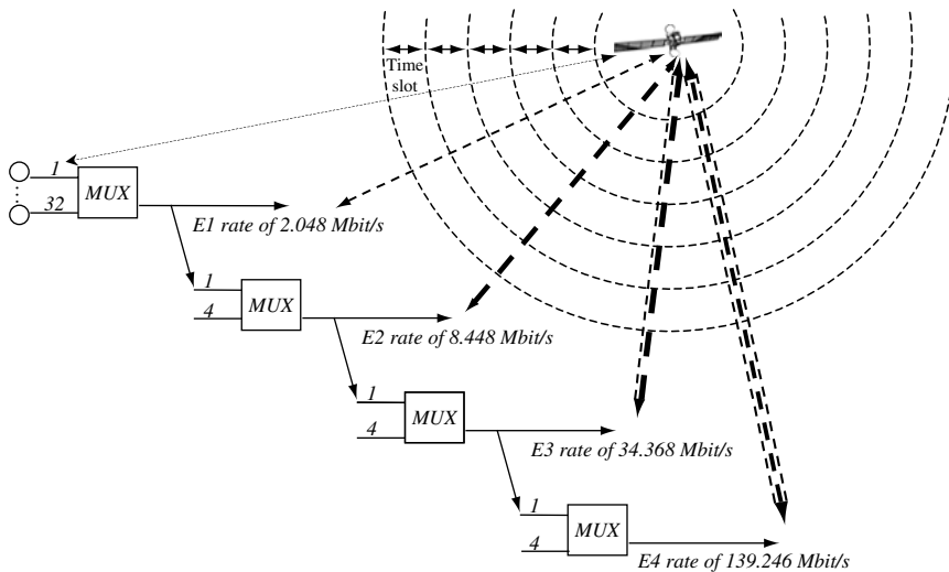
Figure 4.10 Example of traffic multiplexing and capacity requirement for satellite links
