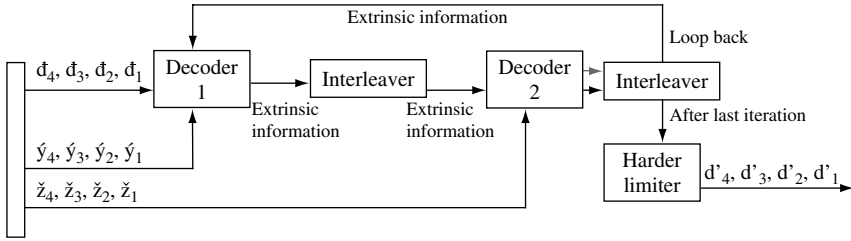
Figure 2.20 Block diagram of turbo decoder
