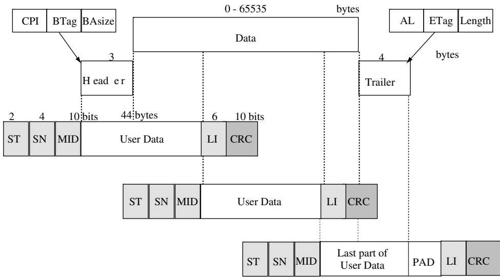
Figure 3.14 AAL 3/4 packet format for Classes C & D
