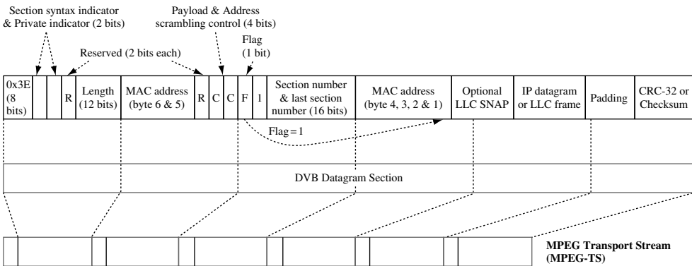
Figure 6.32 IP over DVB: multi protocol encapsulation (MPE)
