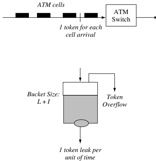
Figure 3.24 Leaky bucket algorithm (LBA)
