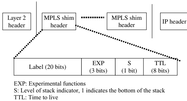
Figure 8.9 MPLS shim header structure
