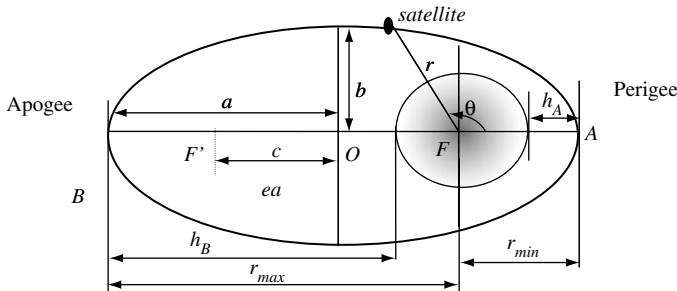
Figure 2.2 Orbit with major axis of orbit (AB) and semi-major axis of orbit (AO)
