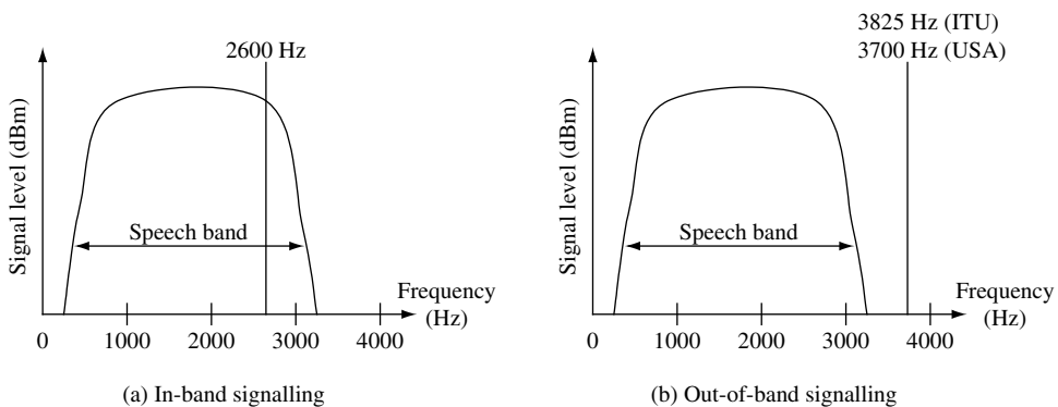
Figure 4.4 Analogue network in-band signalling and out-of-band signalling
