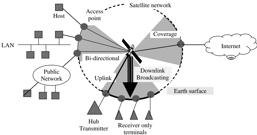
Figure 6.2 Satellite-centric viewpoint of global networks
