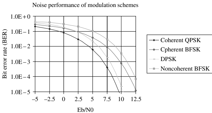
Figure 2.16 Noise performance of modulation schemes
