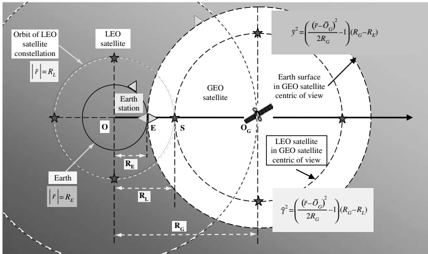
Figure 6.3 Mapping from earth-centric view to GEO-centric view
