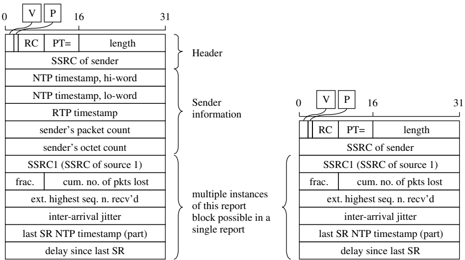
Figure 7.10 Sender report (SR) and receiver report (RR)
