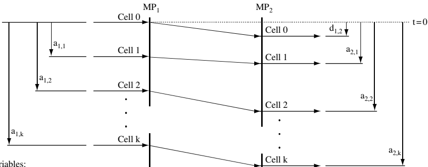
a) Cell delay variation – 1-point definition
