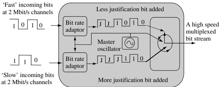
Figure 4.11 Illustration of the concept of plesiochronous digital hierarchy (PDH)
