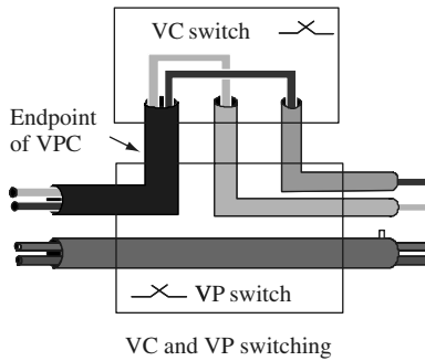
Figure 3.9 Example of VC and VP switching
