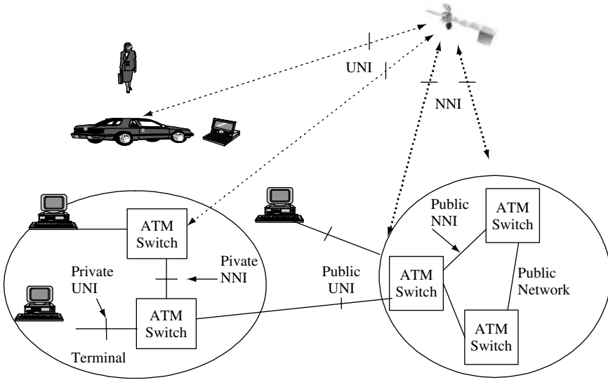
Figure 5.1 Example of user access mode via satellite ATM network
