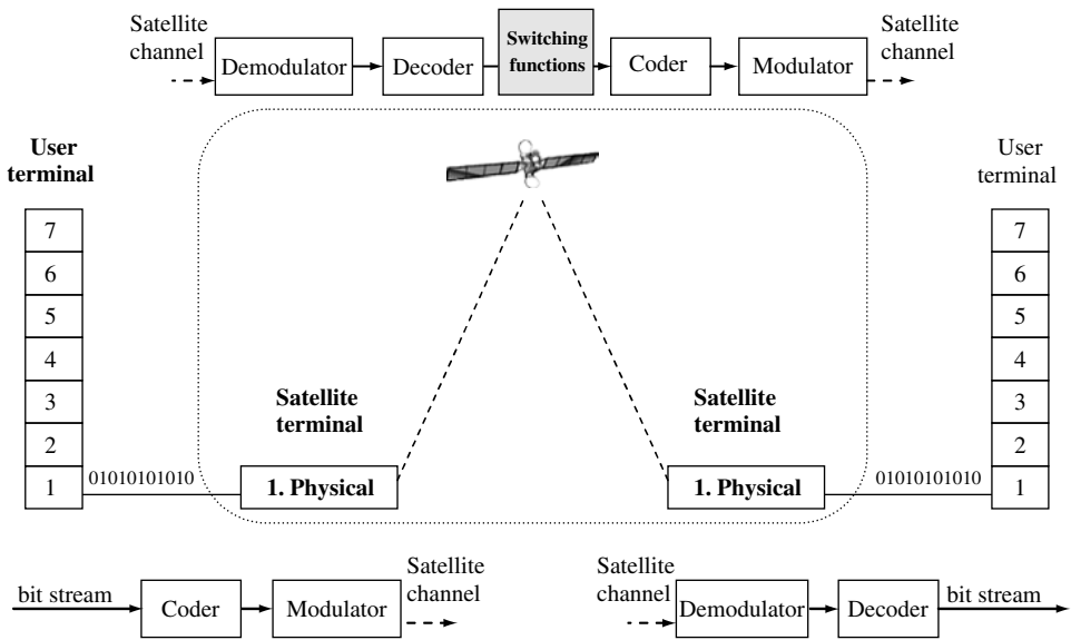
Figure 2.17 Block diagram of physical layer functions of satellite networks
