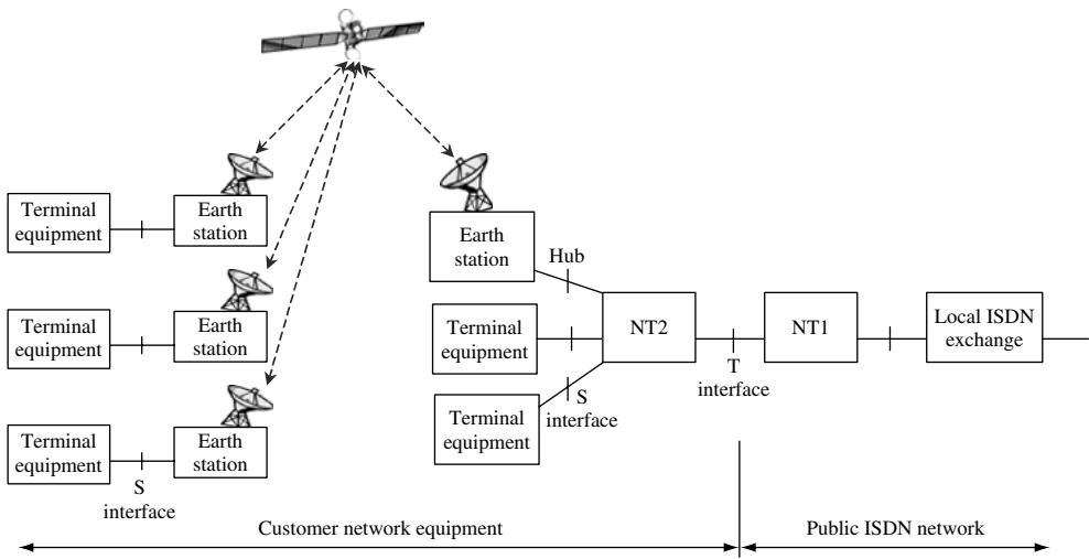
Figure 4.24 Single node distributed ISDN customer network
