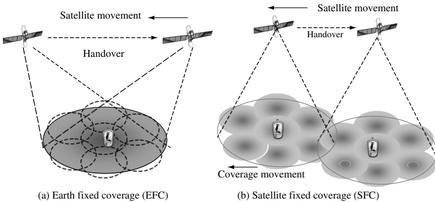
Figure 2.29 Satellite constellations of earth fixed coverage and satellite fixed coverage
