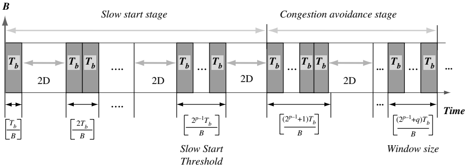
Figure 7.4 TCP segment traffic block bursts
