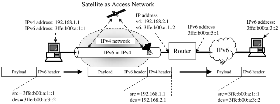
Figure 8.16 Host to router tunnelling through satellite access network
