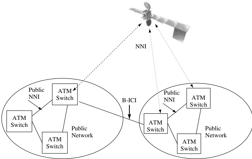
Figure 5.2 Example of network transit mode via a satellite ATM network
