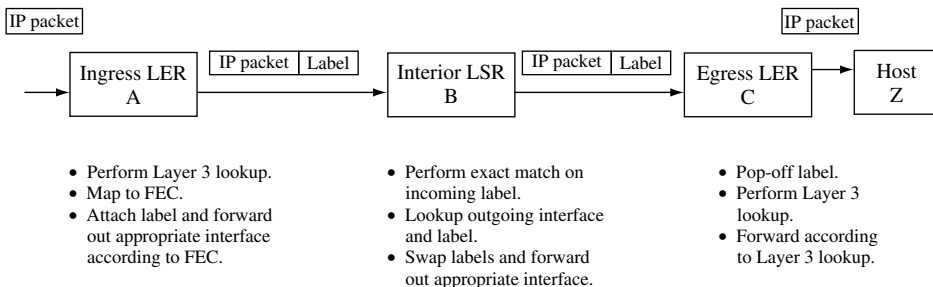
Figure 8.10 Label swapping and forwarding process
