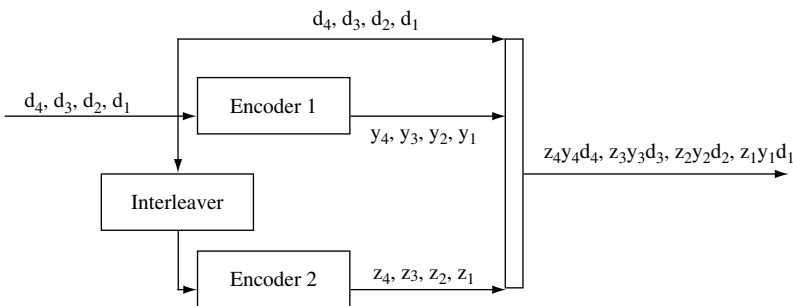
Figure 2.19 Block diagram of turbo encoder
