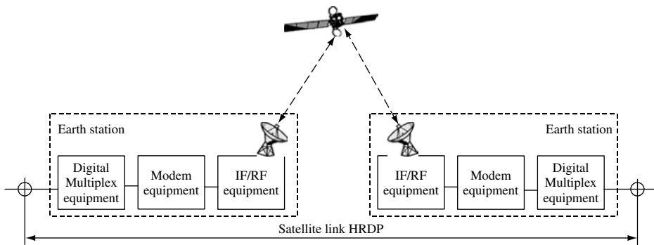
Figure 4.22 Hypothetical reference digital path (HRDP)
