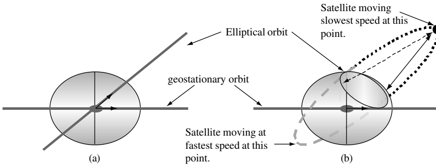
Figure 2.7 A typical high elliptical orbit
