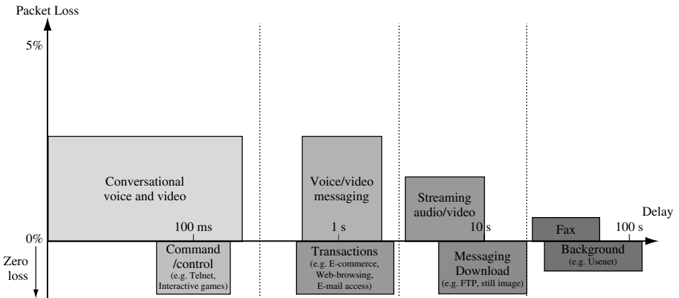
Figure 1.23 Mapping of user-centric QoS requirements into network performance (ITU-T-G1010) (Reproduced with the kind permission of ITU.)
