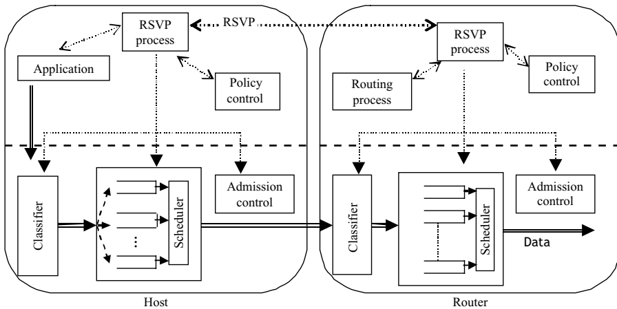
Figure 6.35 Interaction between the different RSVP components
