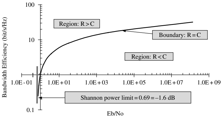
Figure 1.20 Capacity boundary of communication channel
