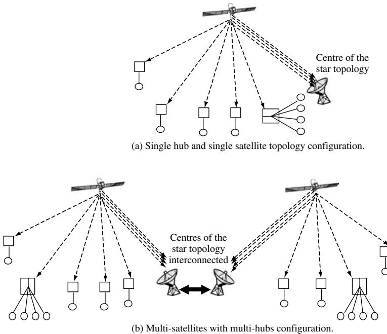
Figure 2.26 Multiple hops topology with hub at the centre
