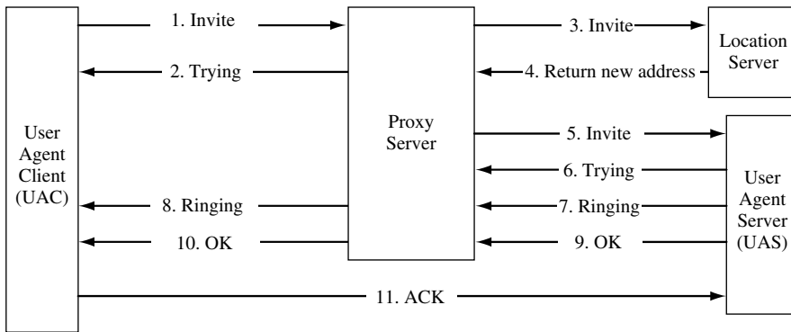
Figure 7.13 A typical SIP call using a proxy server and location server
