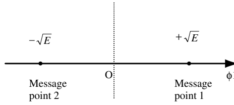
Figure 2.14 Signal-space diagram for coherent BPSK
