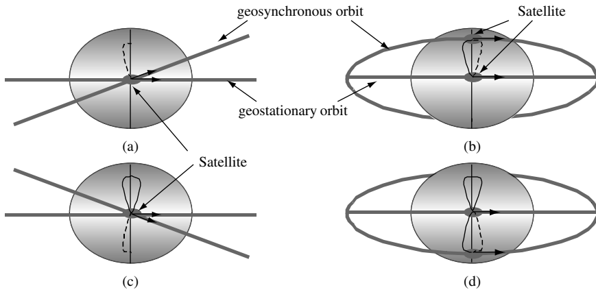
Figure 2.6 Footprints of geosynchronous satellites
