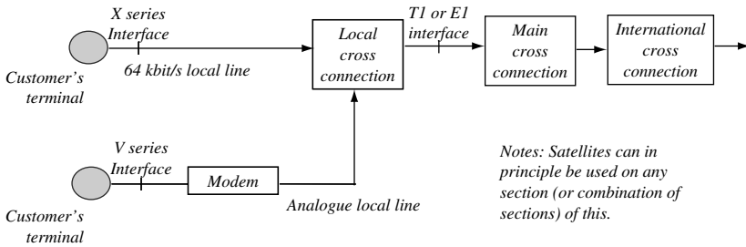
Figure 4.3 Example of network connections and interfaces
