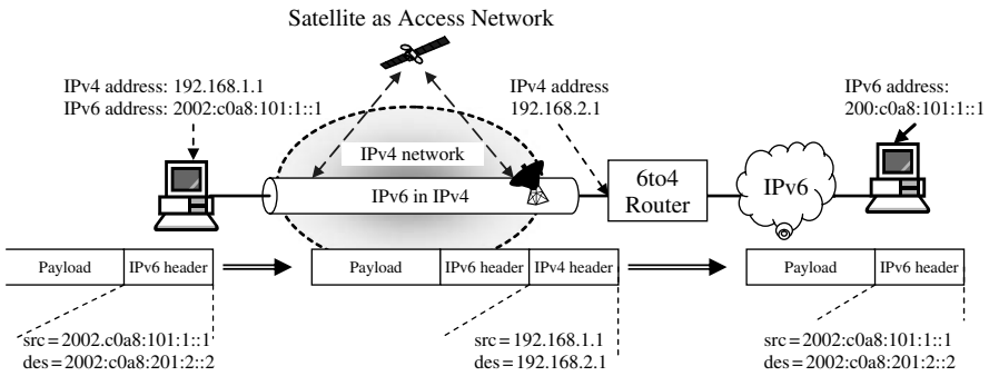
Figure 8.18 The 6to4 translation via satellite access network
