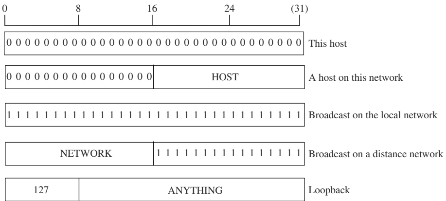
Figure 3.31 Special IP addresses
