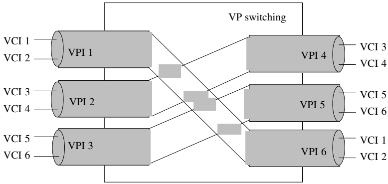
Figure 3.8 Example of VP switching
