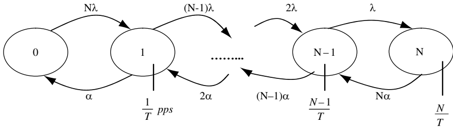
Figure 8.5 Superposition of N voice sources with exponentially distributed inter-arrivals
