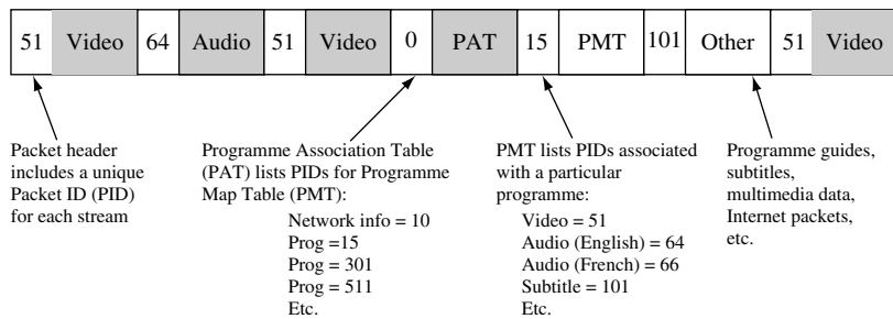
Figure 6.28 DVB service information (DVB-SI) and MPEG signalling
