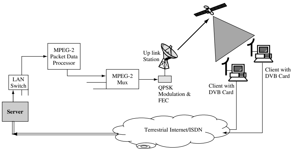
Figure 6.23 DVB-S with return channel via terrestrial networks
