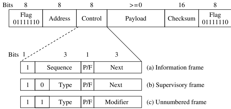
Figure 6.6 HDLC frame structure
