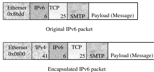
Figure 8.15 Encapsulation of IPv6 packet into IPv4 packet
