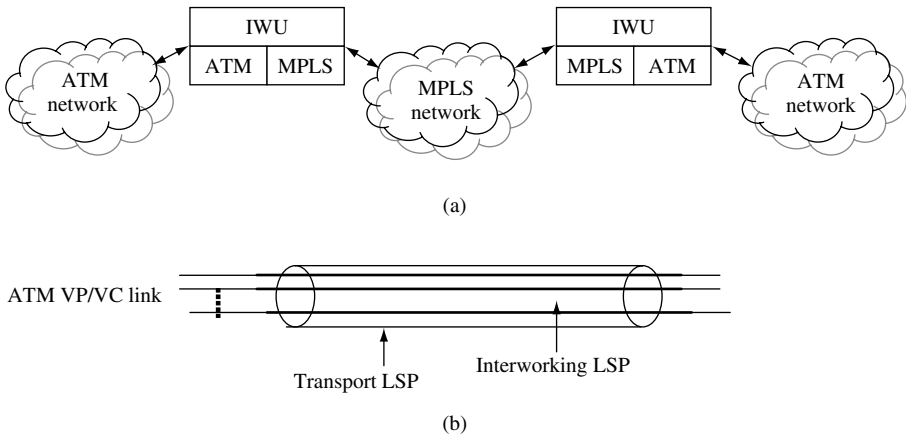
Figure 8.11 ATM-MPLS networks interworking. (a) ATM-MPLS network interworking architecture. (b) the relationship between transport LSP, interworking LSP and ATM link
