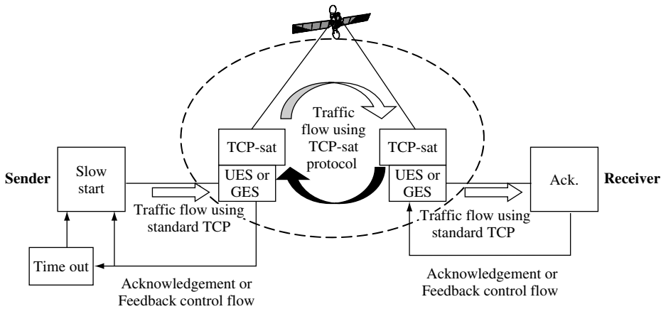
Figure 7.6 The concept of satellite-friendly TCP (TCP-sat)
