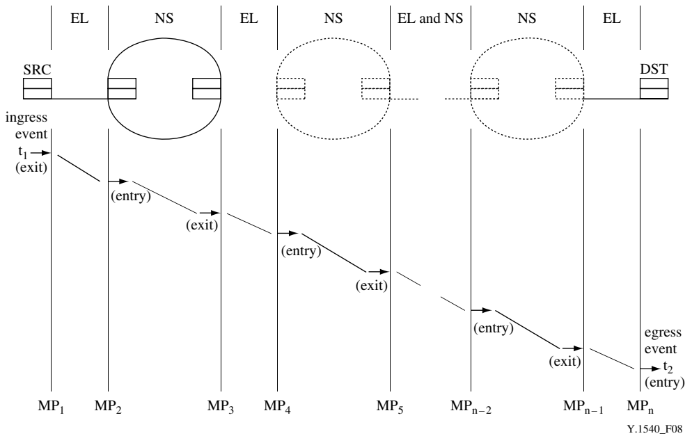
Figure 6.34 IP packet transfer delay events [ITU-Y.1540] (illustrated for the end-to-end transfer of a single IP packet) (Reproduced with the kind permission of ITU.)
