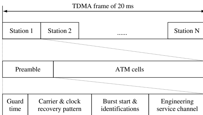
Figure 5.4 TDMA frame format (earth station to satellite)
