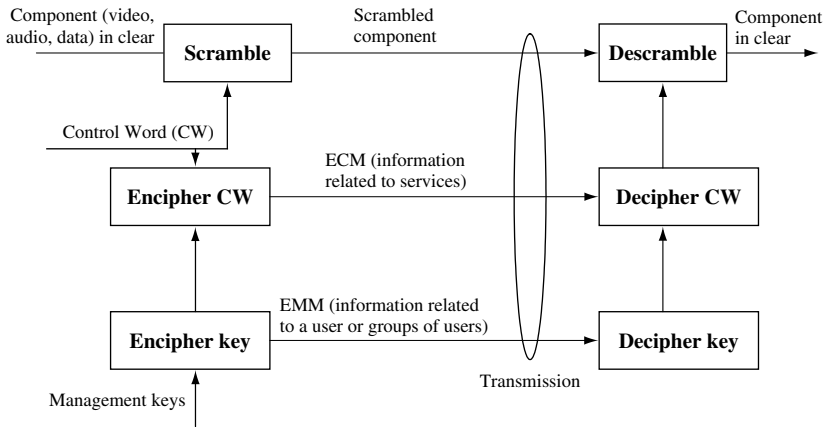
Figure 6.30 DVB conditional access
