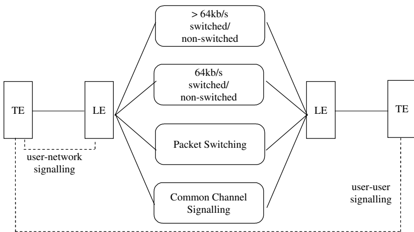
Figure 4.17 Basic architectural features of an ISDN
