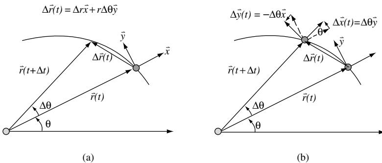
Figure 2.1 Vector from earth to satellite
