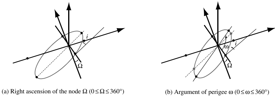
Figure 2.5 Right Ascension of the node \Omega and argument of perigee \omega
