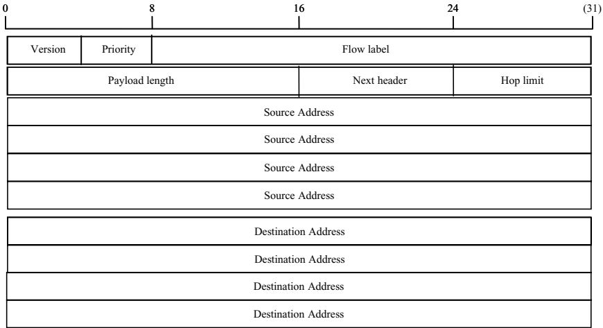
Figure 8.12 IPv6 packet header format
