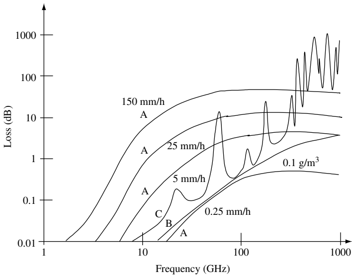
Figure 1.19 Attenuations of different frequency bands due to A: rain, B: fog and C: gas
