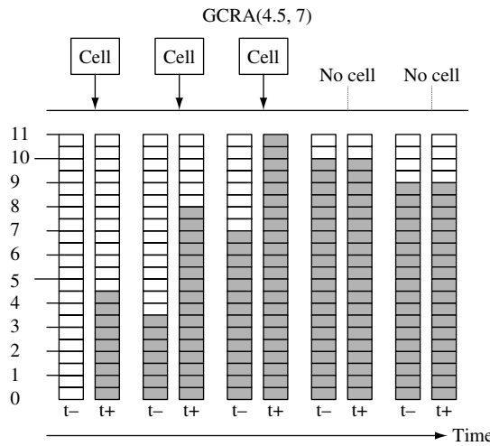
Figure 3.26 Illustration of burst traffic coming to the leaky bucket - GCRA(4.5, 7)
