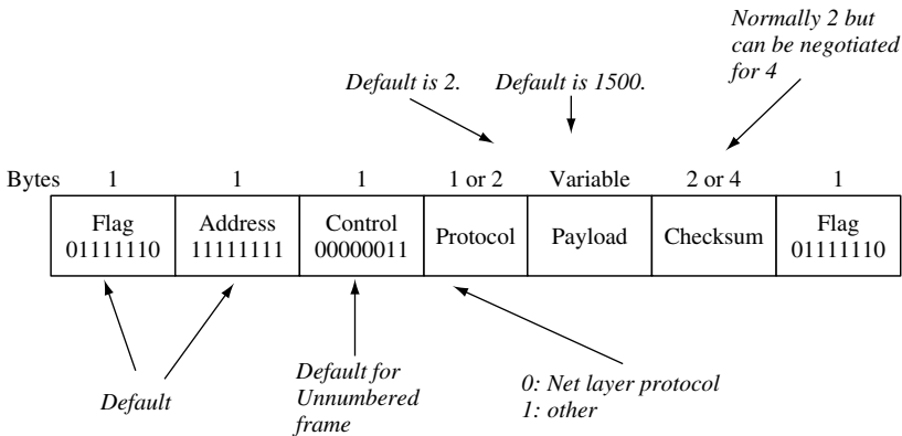
Figure 6.7 Frame structure of the point-to-point protocol (PPP)
