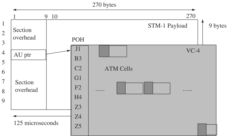
Figure 3.17 SDH STM-1 frame
