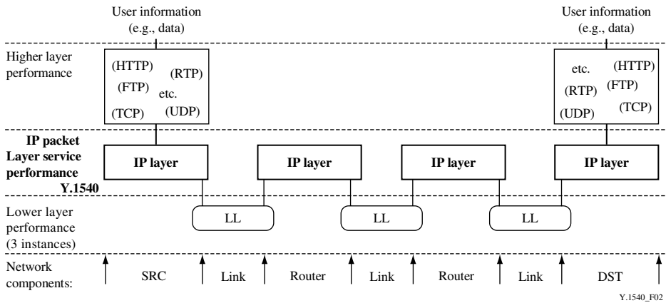
Figure 6.33 Layered model of performance for IP service (ITU-T, Y.1540) (Reproduced with the kind permission of ITU.)
