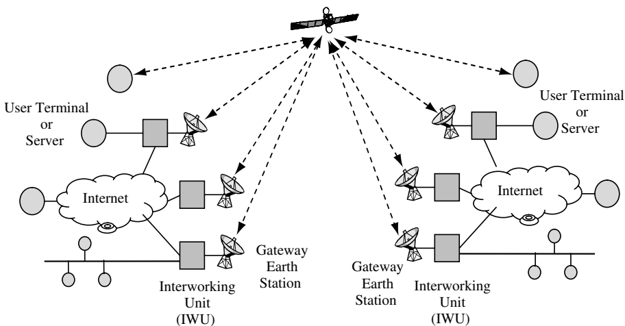
Figure 7.7 Satellite configuration with caches at IWU
