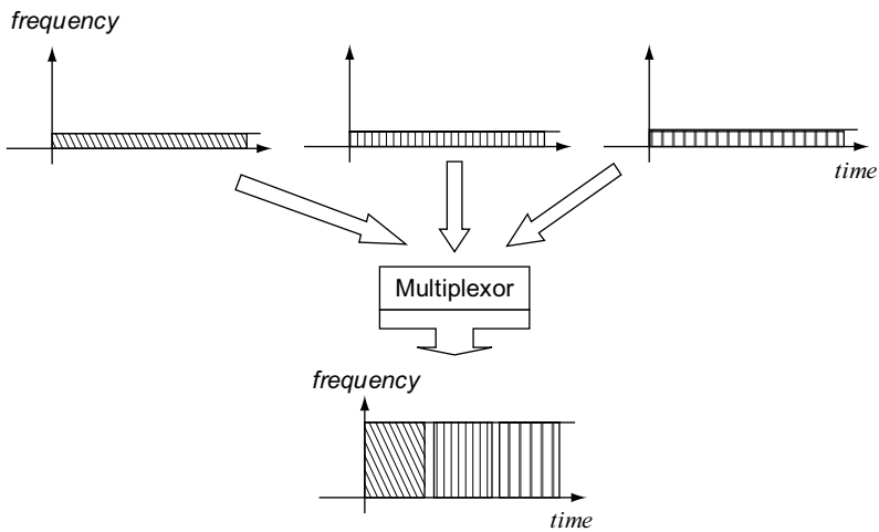
Figure 1.7 Concept of multiplexing in the time domain
