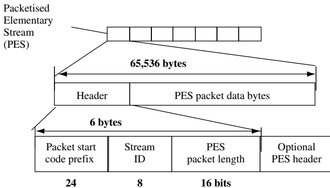
Figure 6.25 MPEG-2 packetised elementary stream (PES)
