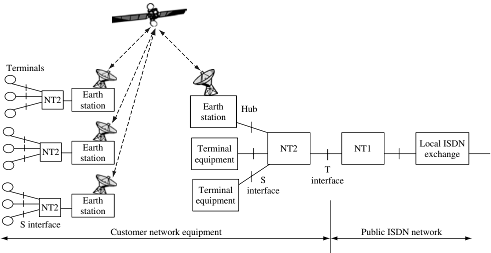
Figure 4.25 Multiple nodes distributed ISDN customer network
