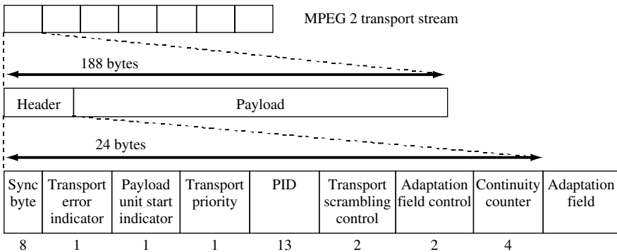
Figure 6.26 MPEG-2 transport stream (MPEG-TS)
