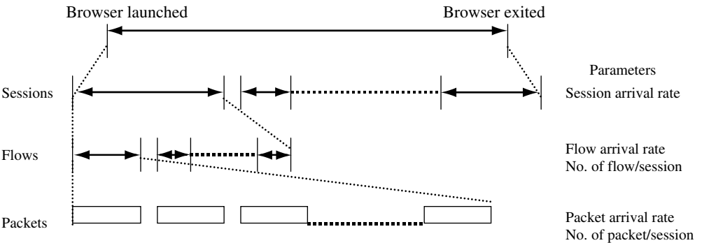
Figure 8.6 Multi-layer modelling
