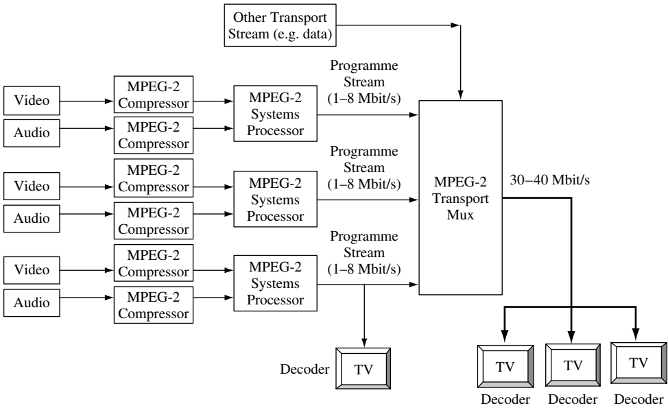
Figure 6.24 MPEG-2 source coding and multiplexing DVB-S streams
