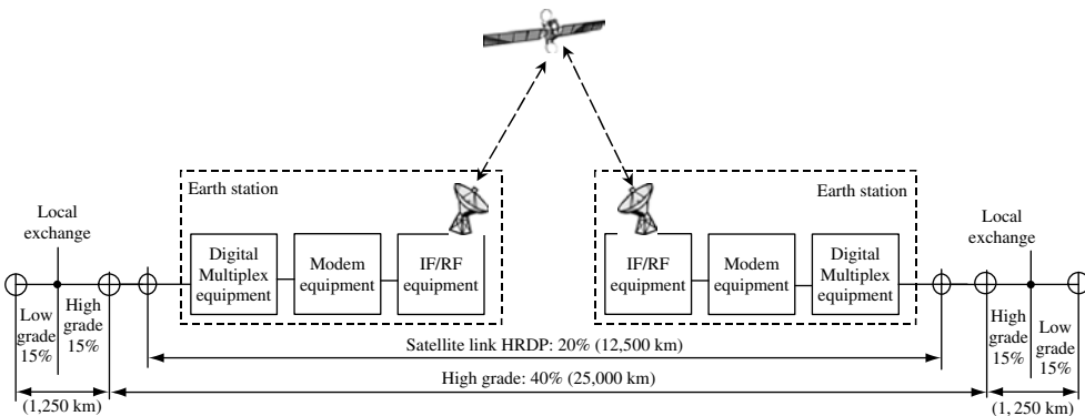
Figure 4.23 HRDP in ITU-T IRX at 64 kbit/s
