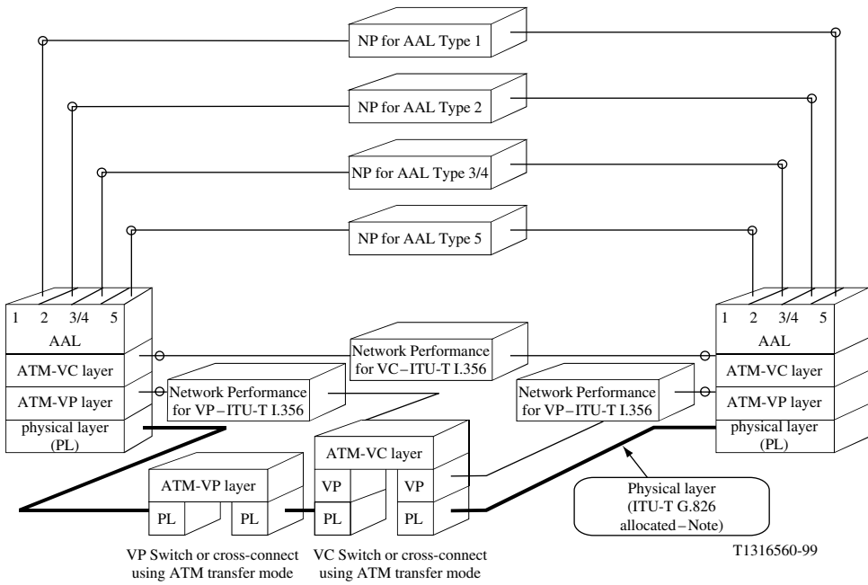
Figure 5.8 Layered model of performance for B-ISDN (ITU-T-1356) (Reproduced with the kind permission of ITU.)
