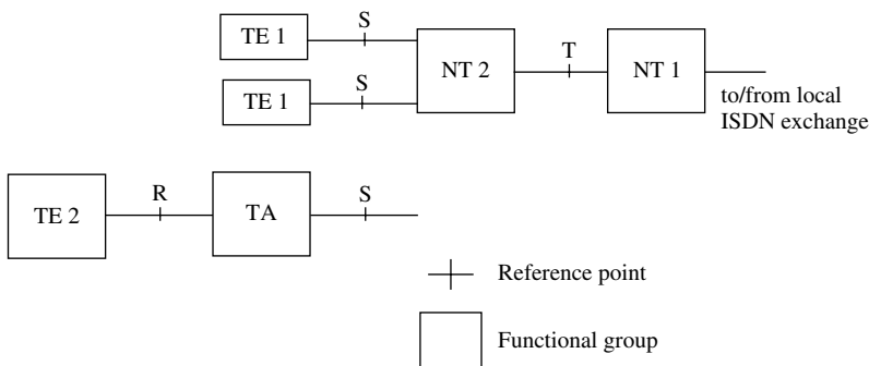
Figure 4.18 Narrowband ISDN (N-ISDN) reference points and functional groups
