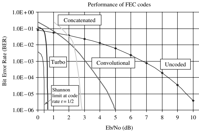
Figure 2.21 Comparison of FEC codes
