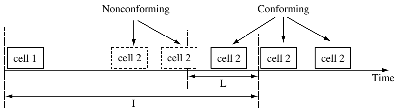
Figure 3.27 Virtual scheduling algorithm (VSA)
