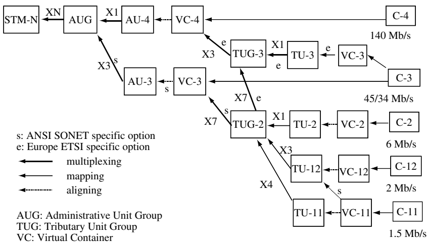
Figure 4.15 Mapping from PDH to SDH
