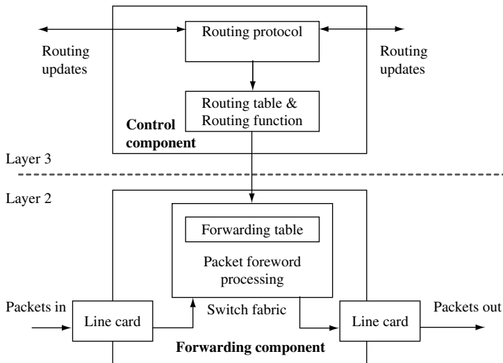
Figure 8.8 Functional components of MPLS
