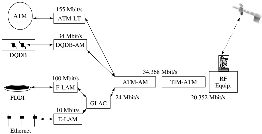
Figure 5.3 Ground-segment modules
