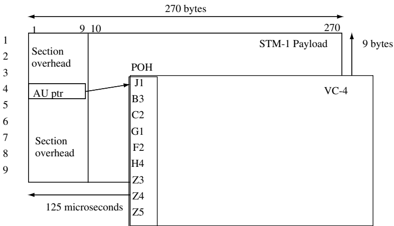
Figure 4.14 STM-1 frame of the SDH network
