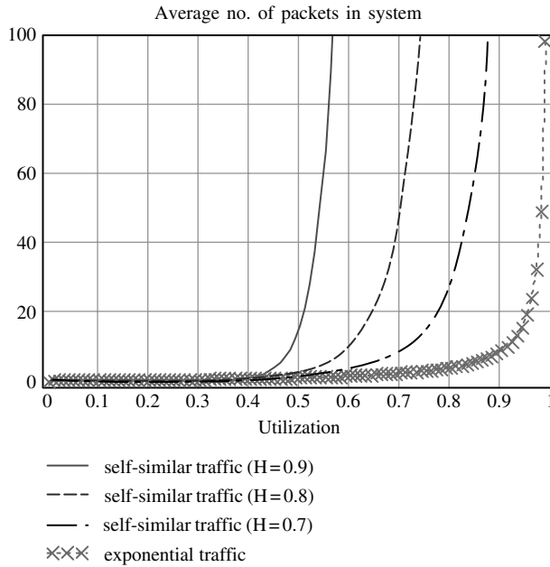
Figure 8.2 Comparison between self-similar traffic and exponential traffic
