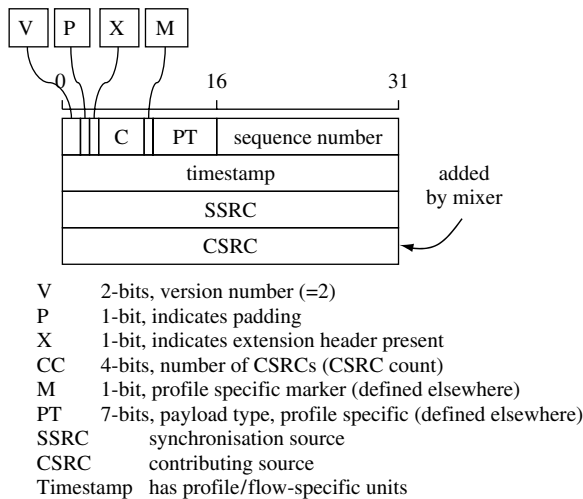
Figure 7.9 RTP header information
