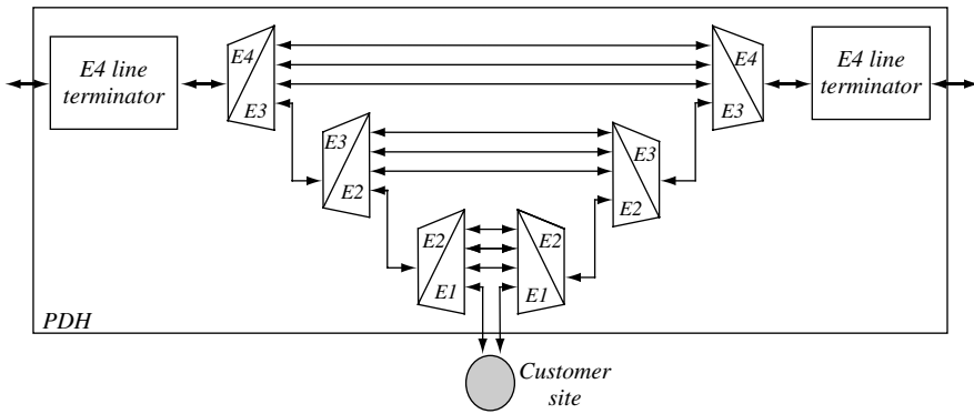
Figure 4.12 Multiplexing and de-multiplexing to insert a network node in PDH network
