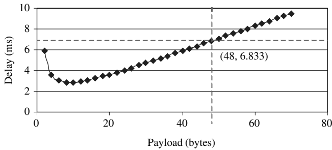
Figure 3.4 Delay due to packetisation and queuing
