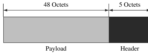
Figure 3.1 ATM cell
