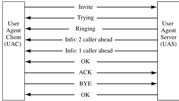
Figure 7.11 A typical SIP call of initiate and terminate session
