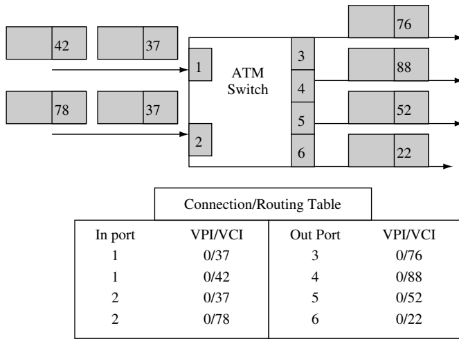
Figure 3.6 Connection/routing table in ATM switch
