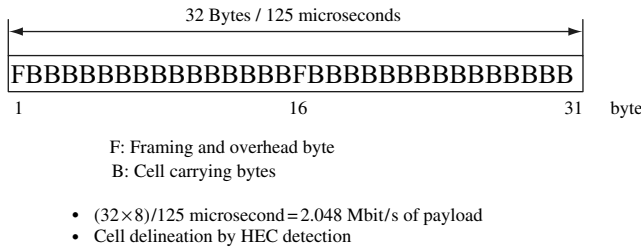
Figure 3.19 E1 frame structure of 2.048 Mbit/s
