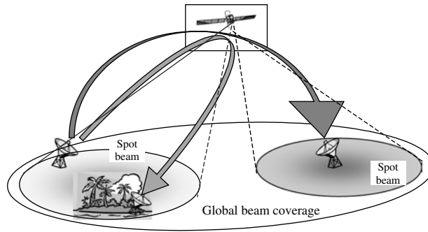
Figure 4.9 Illustration of on-board circuit switching
