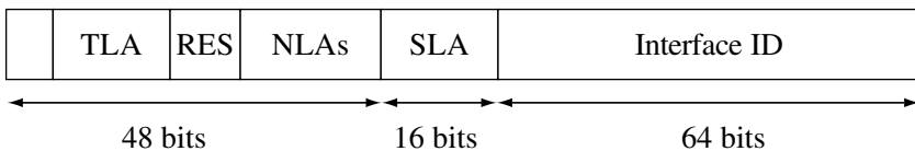
Figure 8.13 Structure of the aggregatable global address
