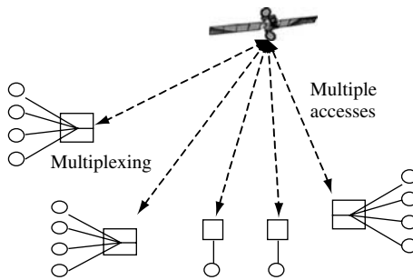
Figure 2.23 Comparison between the concepts of multiplexing and multiple access
