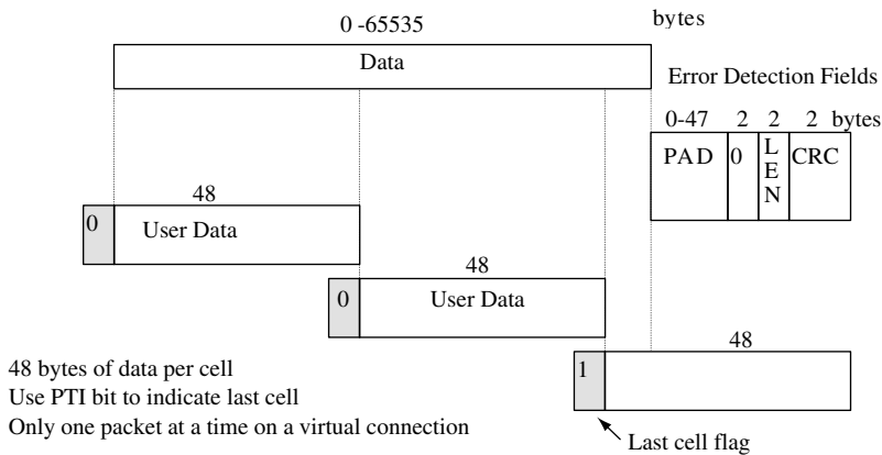
Figure 3.15 AAL 5 format for Internet protocol
