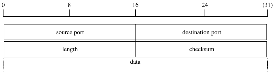
Figure 3.34 The UDP datagram header format
