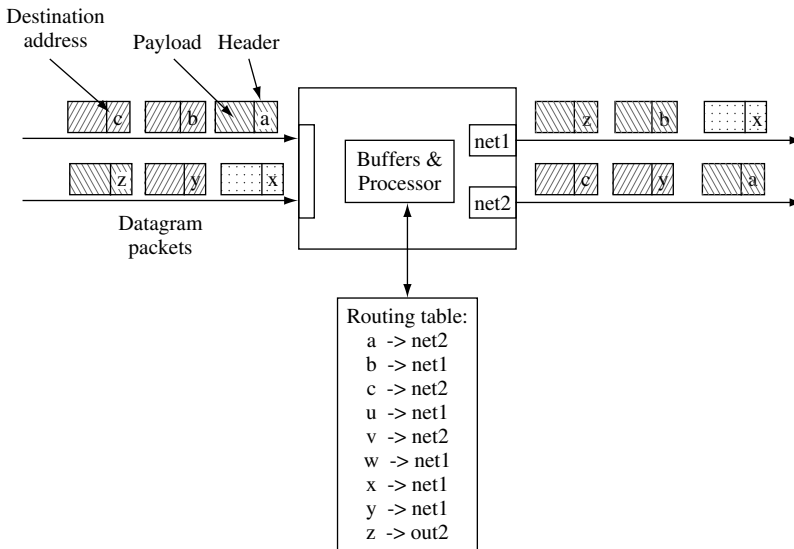
Figure 1.12 Datagram routing concept
