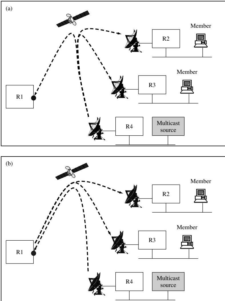
Figure 6.16 Multicast routing flooding: two approaches
