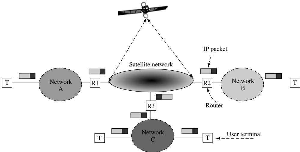
Figure 1.22 Using routers to internetwork with heterogeneous terrestrial networks
