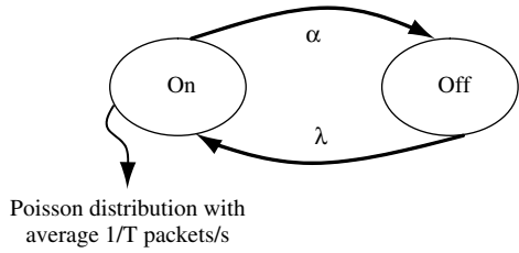
Figure 8.4 A single voice source, represented by a two-state MMPP
