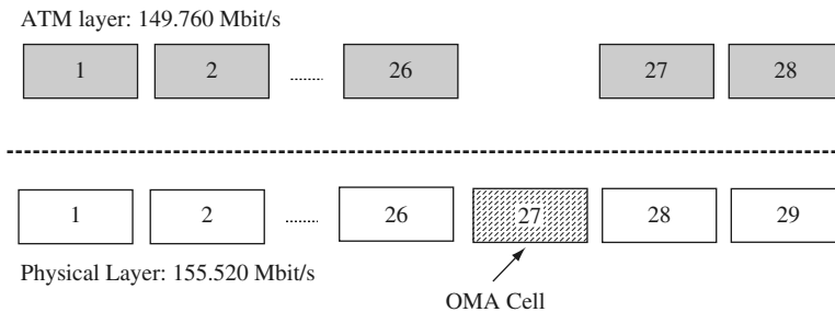
Figure 3.16 The ITU-T target solution for ATM cell transmission
