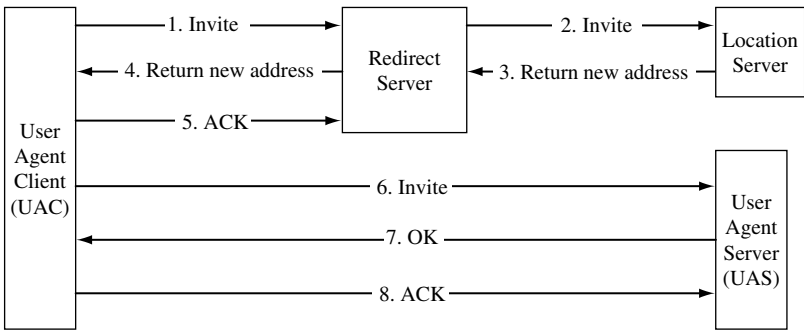
Figure 7.12 A typical SIP call using a redirect server and location server
