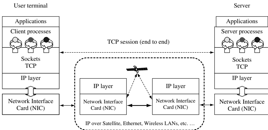
Figure 7.1 The TCP protocol over satellite Internet
