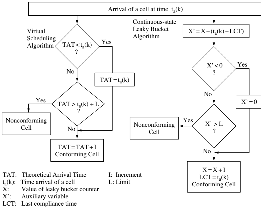
Figure 3.23 Generic cell rate (GCRA) algorithm
