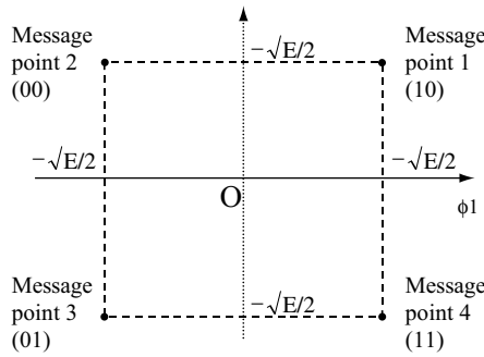
Figure 2.15 Signal-space diagram for coherent QPSK
