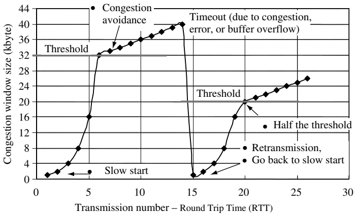
Figure 7.3 An example of TCP operations
