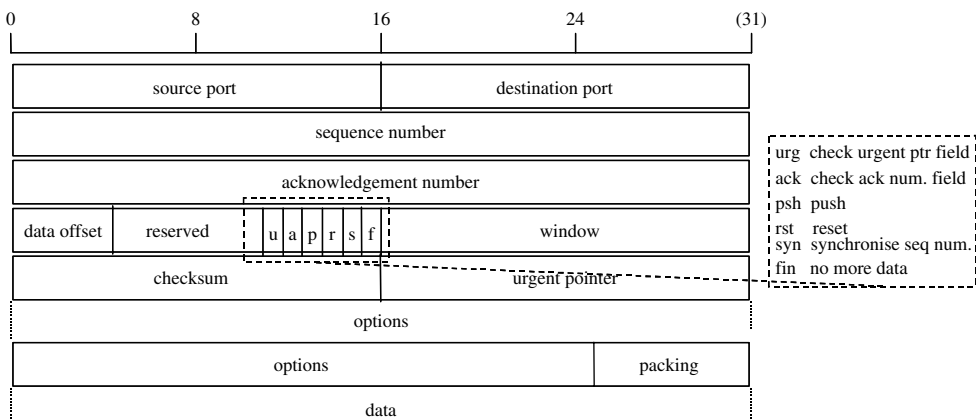
Figure 3.32 The TCP segment header
