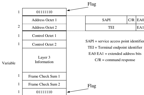
Figure 4.20 LAP-D frame structure (layer 2)
