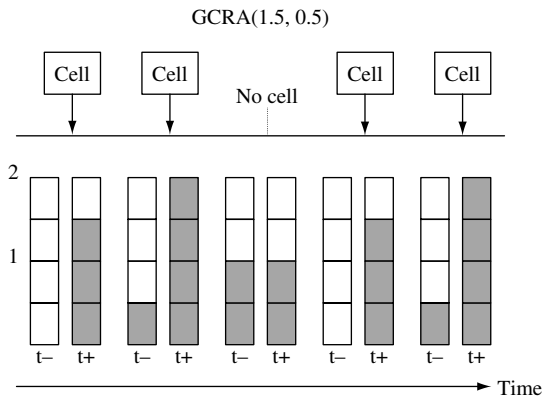
Figure 3.25 An illustration of smooth traffic coming to the leaky bucket - GCRA(1.5, 0.5)
