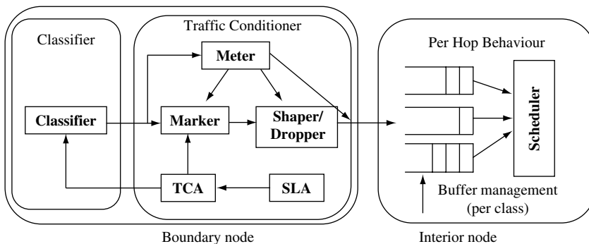
Figure 6.38 Logical view of Diffserv components
