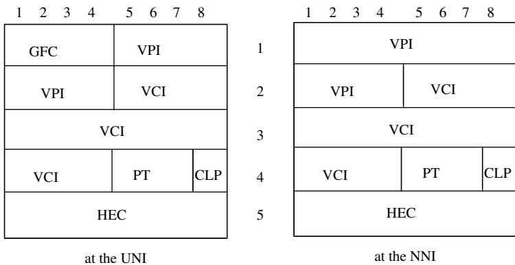
Figure 3.5 The ATM cell header format at the UNI and NNI
