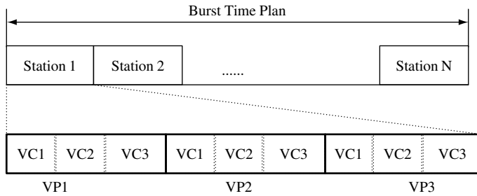
Figure 5.5 Satellite resource management
