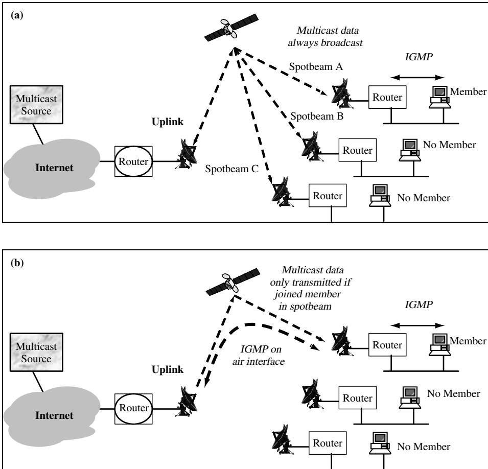
Figure 6.15 IGMP over satellite: (a) static and (b) dynamic multicast
