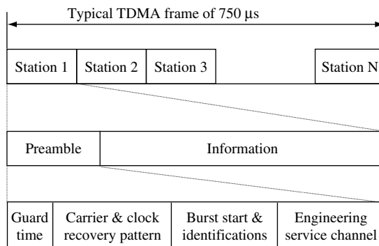
Figure 2.24 A typical example of satellite TDMA scheme
