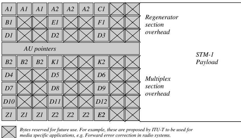
Figure 4.16 Section Overhead (SOH) of the STM-1 frame
