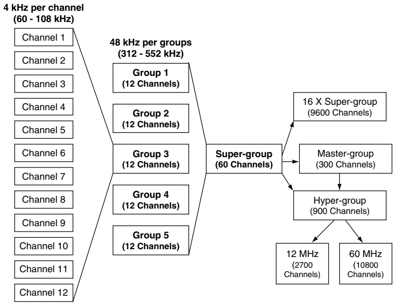
Figure 1.6 Analogue transmission multiplexing hierarchy
