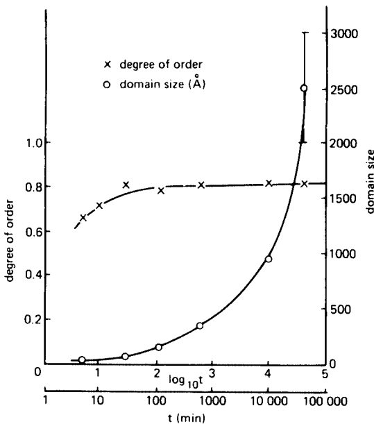
Figure 6.15 Degree of order (x) and domain size (O) during isothermal annealing at 350^\circ\text{C} after quenching from 465^\circ\text{C} (after Morris, Besag and Smallman, 1974; courtesy of Taylor and Francis).
