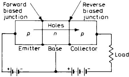
Figure 6.25 Schematic diagram of a p-n-p transistor.
