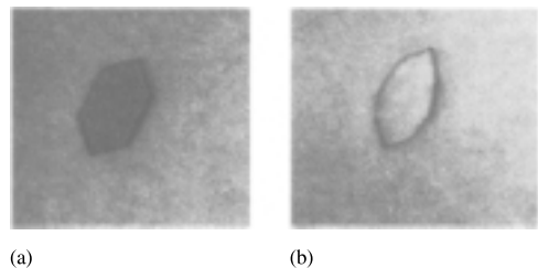
Figure 4.39 Removal of the stacking fault from a Frank sessile dislocation by stress (after Goodhew and Smallman).
