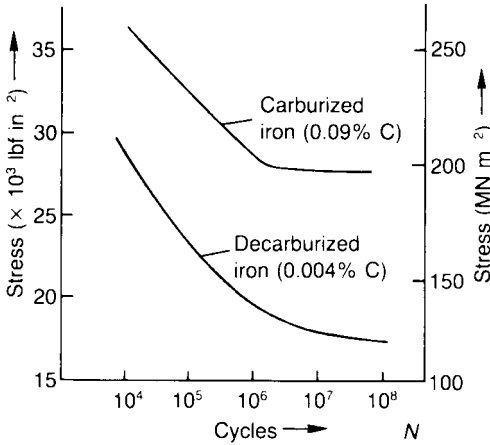
Figure 7.5 S-N curve for carburized and decarburized iron.
