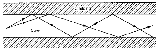
Figure 6.37 Optical guidance in a multimode fibre.
