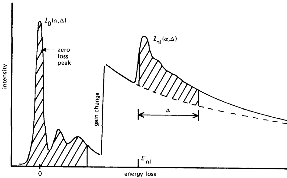
Figure 5.36 Schematic energy-loss spectrum, showing the zero-loss and plasmon regions together with the characteristic ionization edge, energy E_{n1} and intensity I_{n1} .
