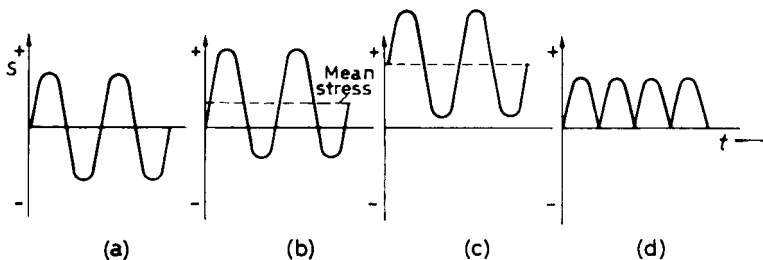
Figure 7.4 Alternative forms of stress cycling: (a) reversed; (b) alternating (mean stress ≠ zero), (c) fluctuating and (d) repeated.
