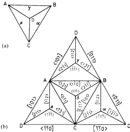
Figure 4.37 A Thompson tetrahedron (a) closed and (b) opened out. In (b) the notation [1\ 1\ 0] is used in place of the usual notation [1\ 1\ 0] to indicate the sense of the vector direction.
