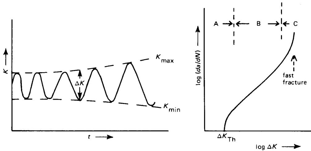
Figure 8.40 (a) Increase in stress intensity \Delta K during fatigue; (b) variation of crack growth rate with increasing \Delta K .
