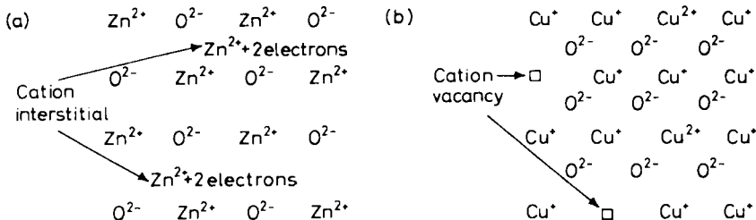
Figure 4.6 Schematic arrangement of ions in two typical oxides. (a) Zn >1 O, with excess metal due to cation interstitials and (b) Cu <2 O, with excess non-metal due to cation vacancies.
