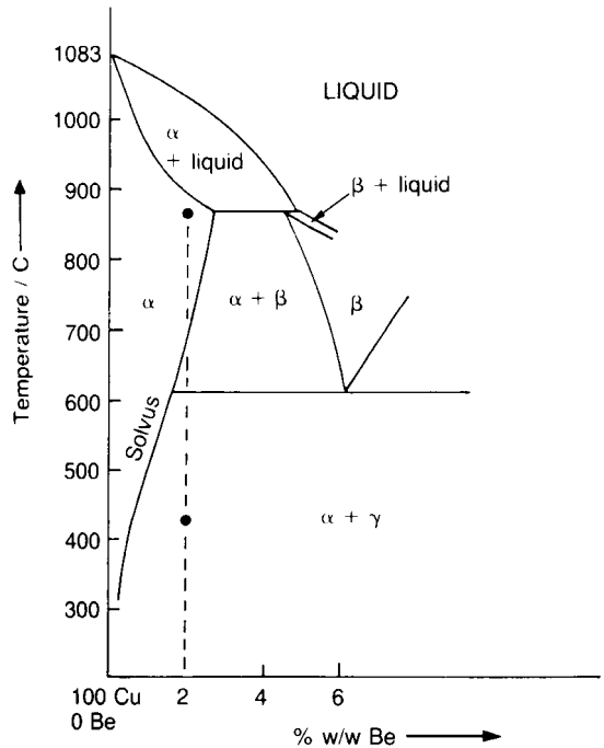
Figure 3.13 Cu-rich end of phase diagram for Cu–Be system, showing field of primary solid solution ( \alpha ).
