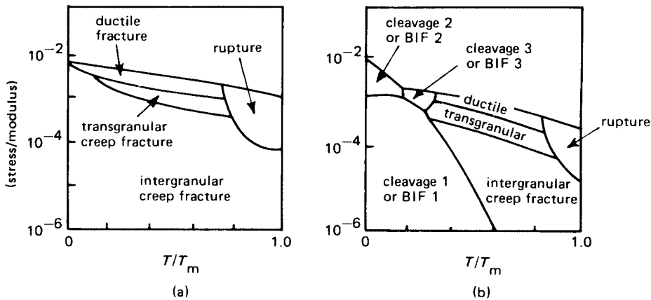
Figure 8.39 Schematic fracture mechanism maps for (a) fcc and (b) bcc materials.
