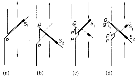
Figure 7.74 Formation of intrusions and extrusions (after Cottrell; courtesy of John Wiley and Sons).
