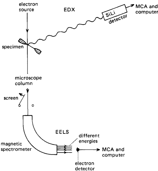
Figure 5.33 Schematic diagram of EDX and EELS in TEM.
