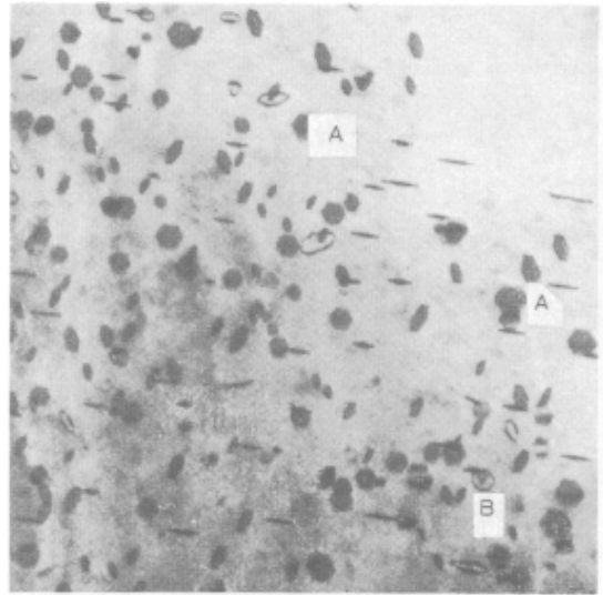
Figure 4.38 Single-faulted, double-faulted (A) and unfaulted (B) dislocation loops in quenched aluminium (after Edington and Smallman, 1965; courtesy of Taylor and Francis).
