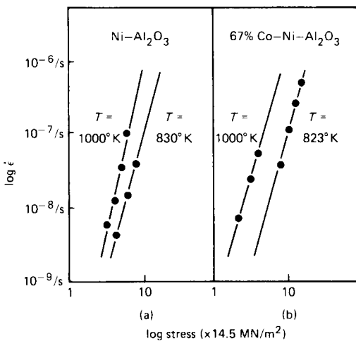
Figure 7.63 \log \dot{\epsilon} versus \log \sigma for (a) \text{Ni-Al}_2\text{O}_3 , (b) \text{Ni-67Co-Al}_2\text{O}_3 (after Hancock, Dillamore and Smallman, 1972).
