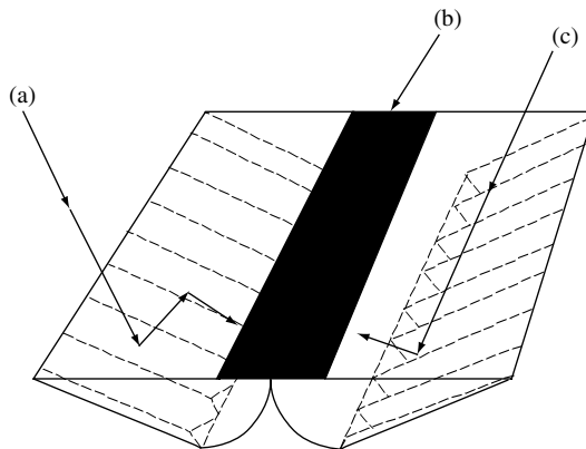
Figure 11.35 Static concentrator using bifacial cells with dielectric prisms. Bowden S, High Efficiency Photovoltaic Roof Tiles with Static Concentrators , First World Conference on Photovoltaic Energy Conversion © 1994 IEEE
