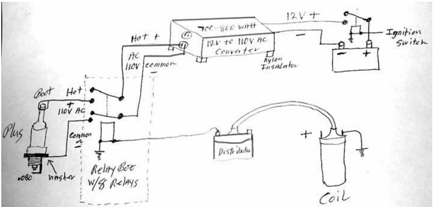
Simple Drawing of Water Power CAR 2
