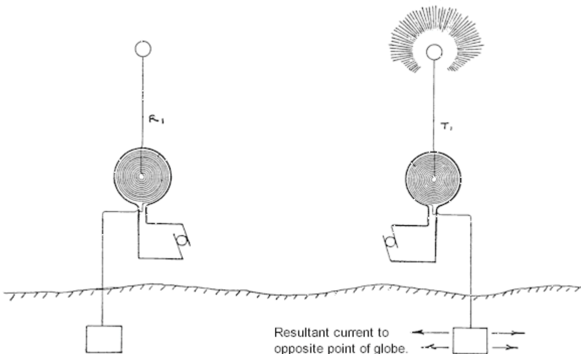
Fig. 2 — System Devised by Tesla
