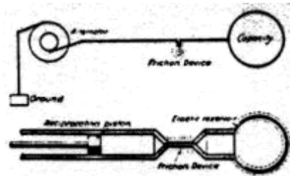
Fig. 4. Electric Transmission Thru a Single Wire Hydraulic Analog.
