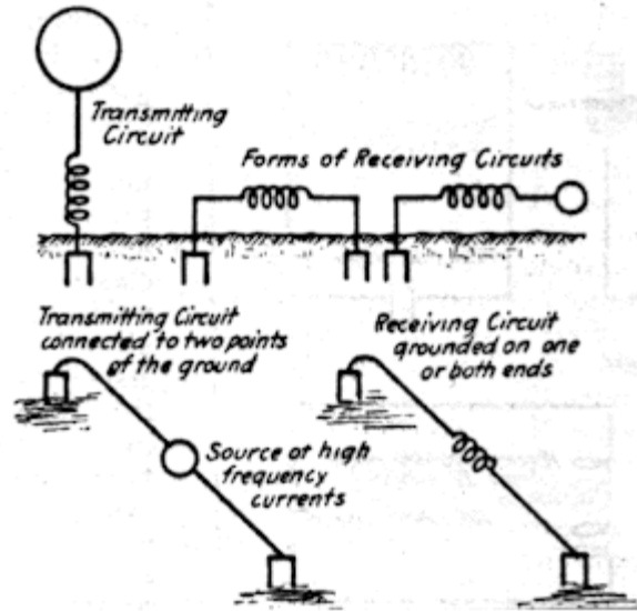
Fig. 12. Arrangements of Directive Circuits Described In Tesla's U. S. Patent No. 613,809 of November 8. 1898, on "Method of and Apparatus for Controlling Mechanism of Moving Vessels or Vehicles."
