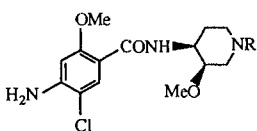
(153); R = CH 2 C 6 H 5
