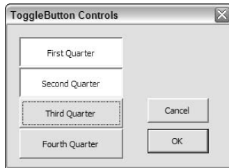
Figure 17-17: ToggleButton controls.
