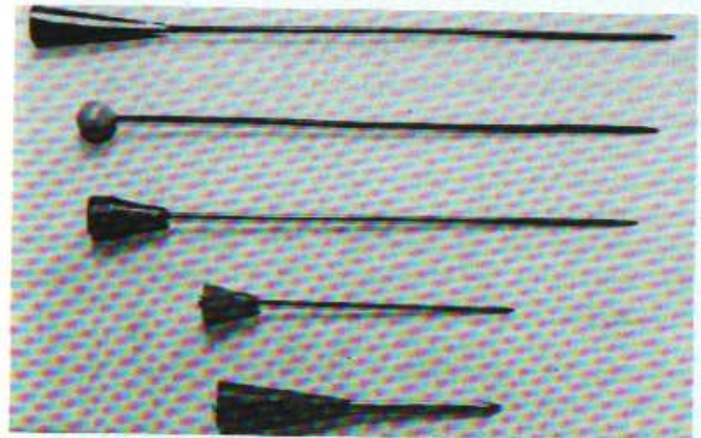
Examples of steel darts. From top to bottom: a homemade spring steel dart with paper cone stopper, a commercial bead dart, a homemade steel dart with a golf tee stopper, a commercial cone dart, and a dart made from a finishing nail with a paper cone stopper.
