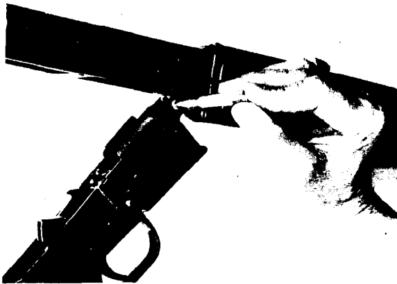
Disengage/Engage Receiving Pivot Pin Figure 3-18
