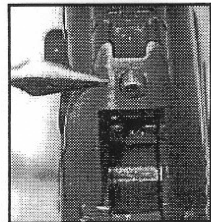
FIG. 3 — LOADED CHAMBER INDICATOR PROTRUDING—DENOTING CARTRIDGE IN CHAMBER..
