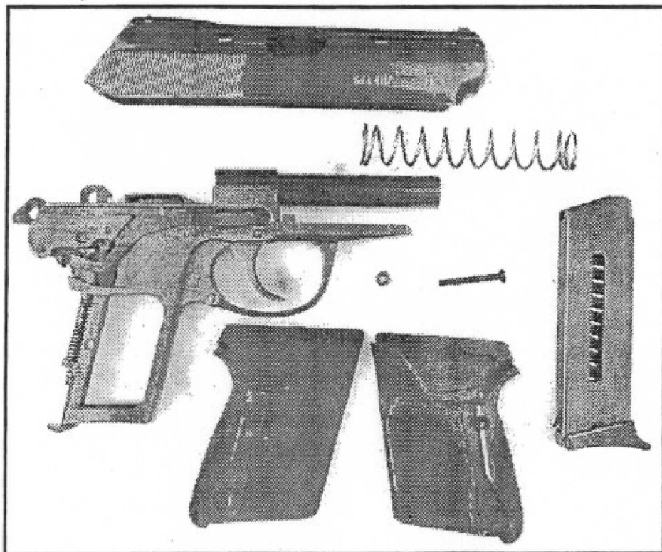
FIGURE 5: PISTOL DISASSEMBLED FOR CLEANING.
