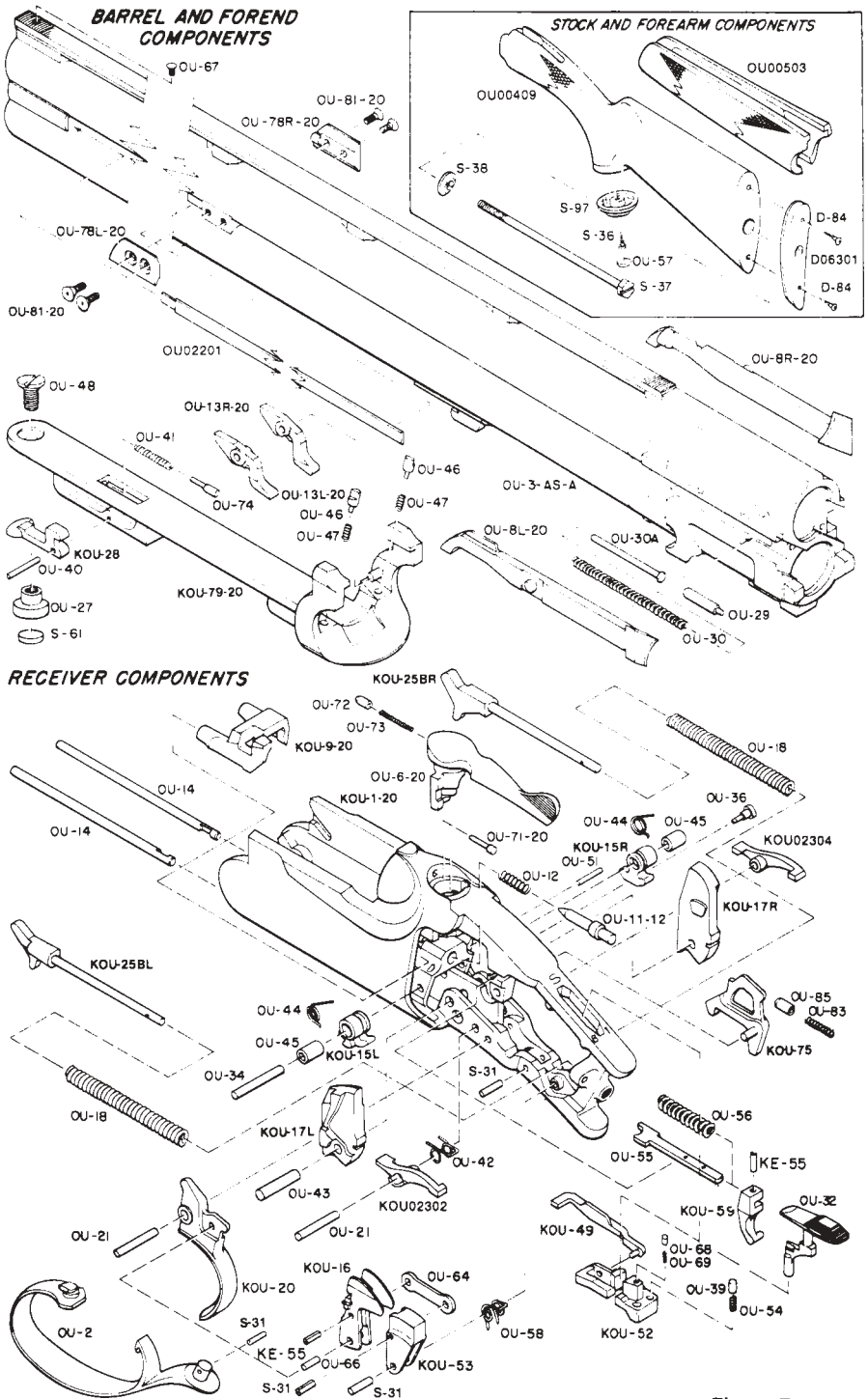
Figure 7 COMPONENT PARTS FOR 20 GAUGE
