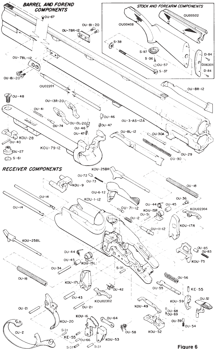
Figure 6 COMPONENT PARTS FOR 12 GAUGE
