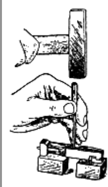
Figure 13: Driving out the pin to remove the firing pin and extractor.
