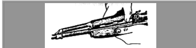
Figure 5: Removing the gas tube with handguard
