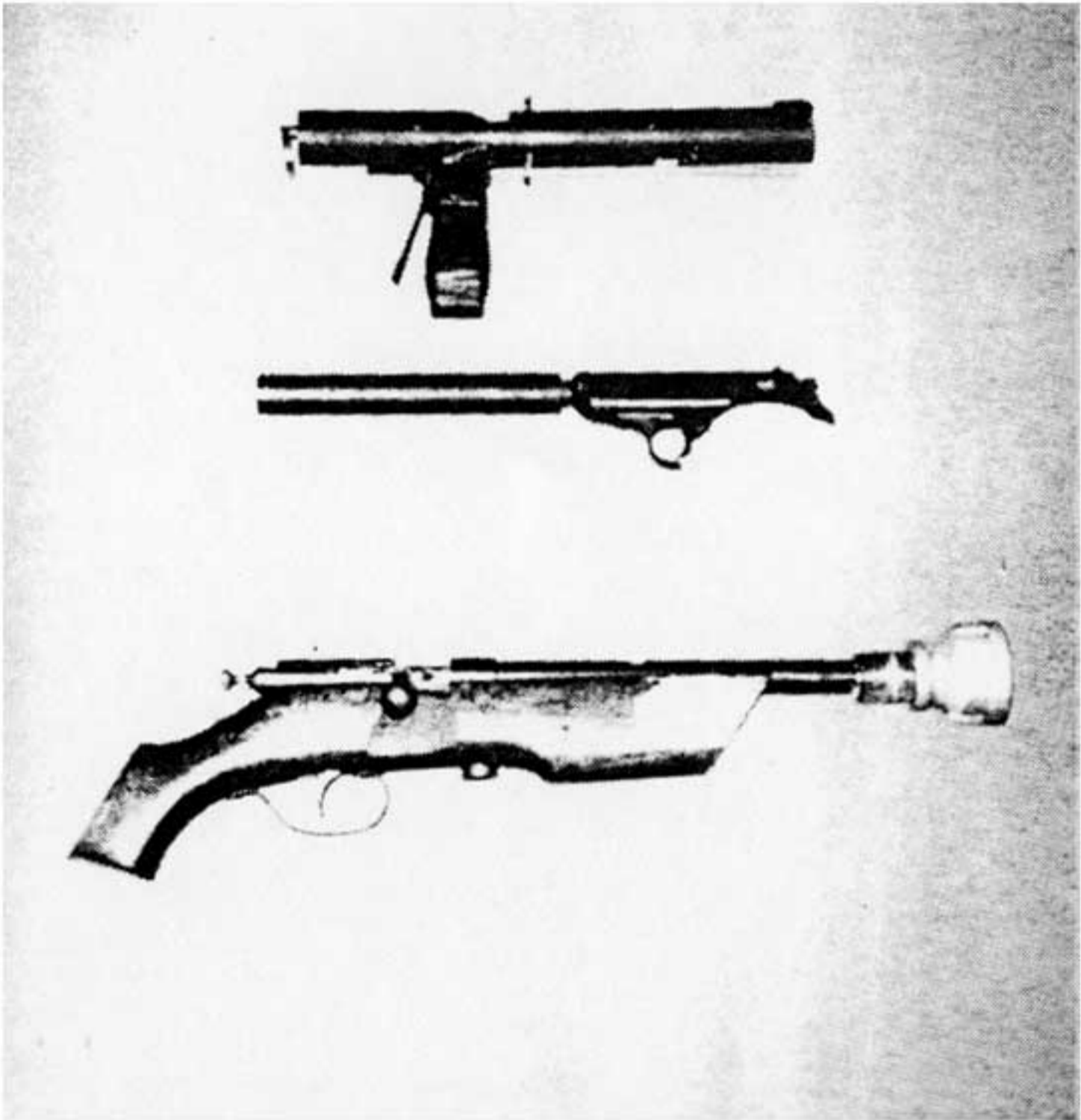
SILENT PISTOLS Top to bottom i Librod 22 cal ii PPK .22 cal with Parker-Hale moderator iii Cut-down .22 rifle with bell reducer (point blank) silencer-muzzle to skin
